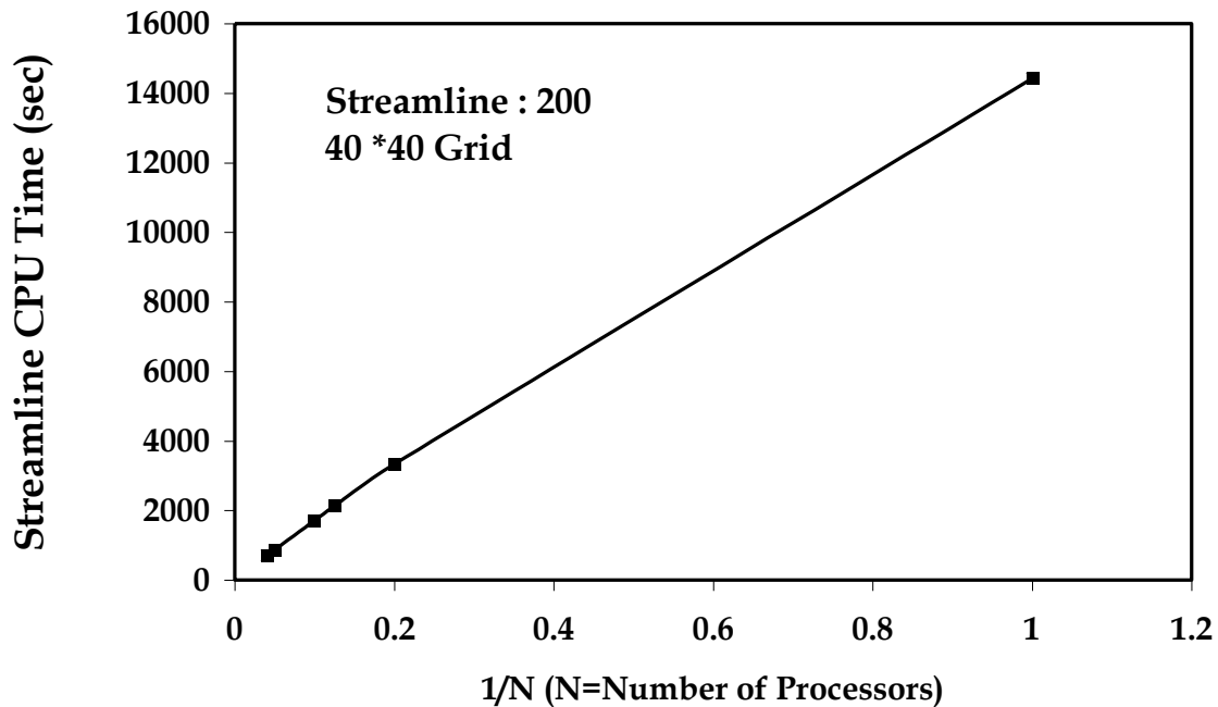
Fig. 66 - Streamline CPU time vs. (1 / Number of Processors)
