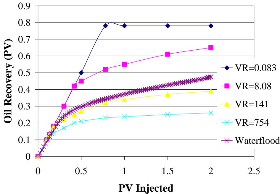
Fig. 14 – Comparison of waterflood recovery in 5-spots with literature data 34
