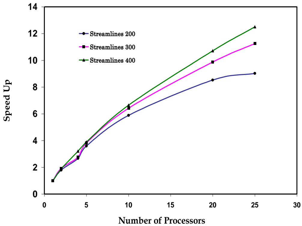
Fig. 71 - Speed up vs. number of processors with different number of streamlines
