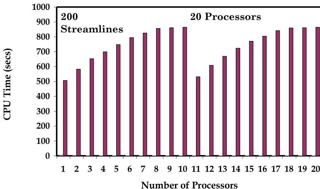
Fig. 67 - CPU load distribution for a 20 processor run on 40 *40 grid and 200 streamlines
