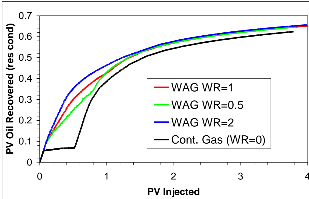
Fig. 79 - Continuous gas vs. WAG oil recovery
