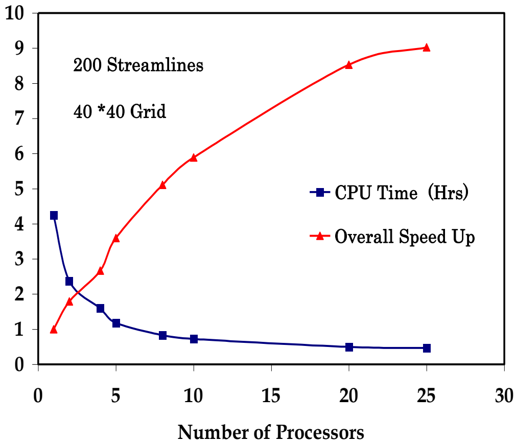
Fig. 64 - CPU time and overall speed up vs. number of processors for 200 streamlines
