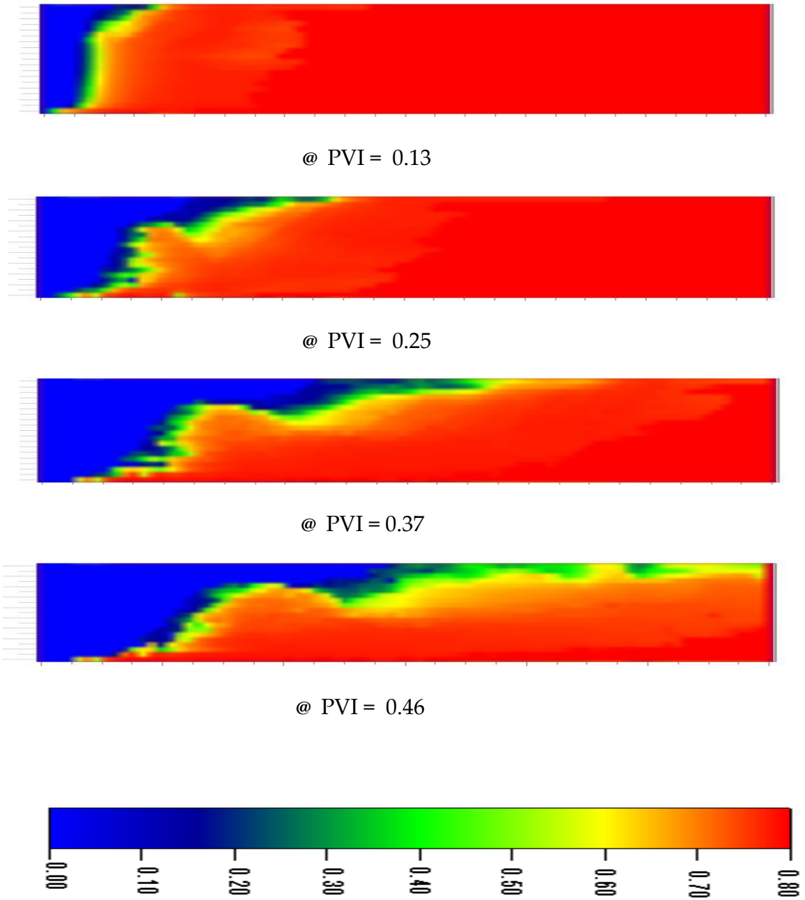
Fig. 46 - Oil saturation profile for 2-D homogeneous (X-Z) gas injection ( N_g=0.186 )
