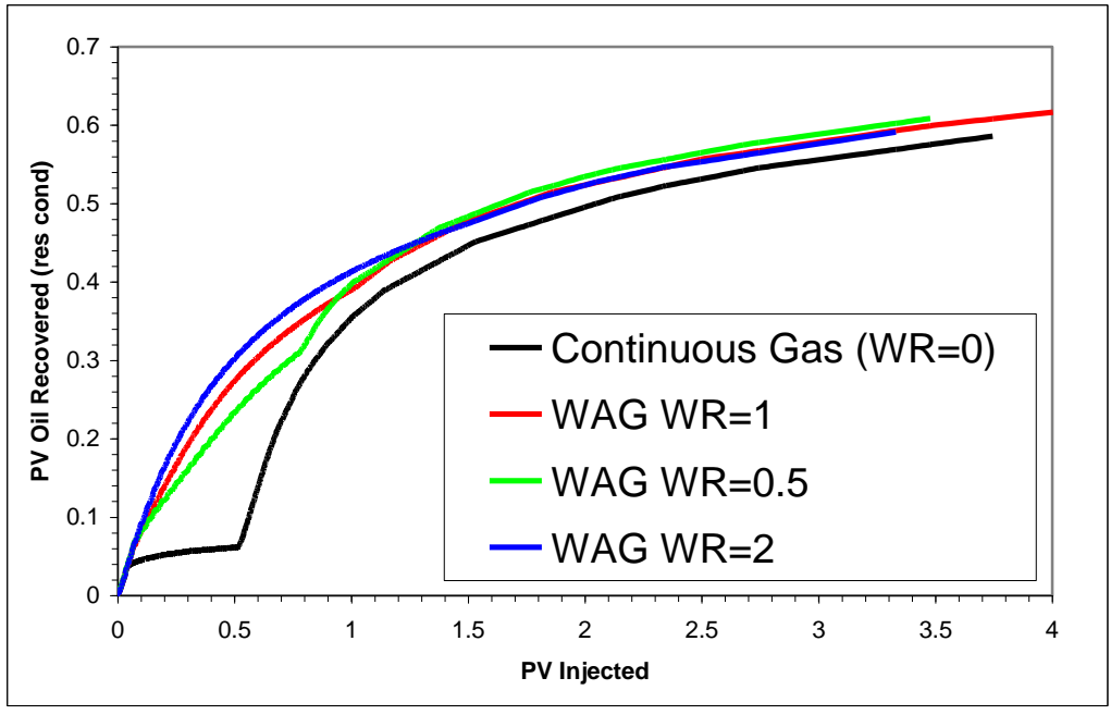
Fig. 83 - Continuous gas vs. WAG injection
