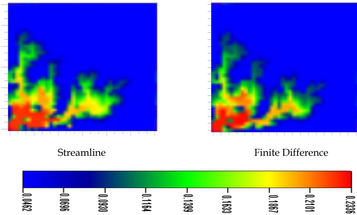
Fig. 39 - Methane concentration @ 0.10 PVI for 2-D (X-Y) gas injection - heterogeneous
