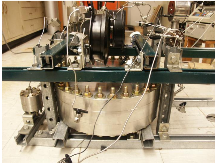
Fig. 3 - Front view of the quarter 5-spot high-pressure cell
