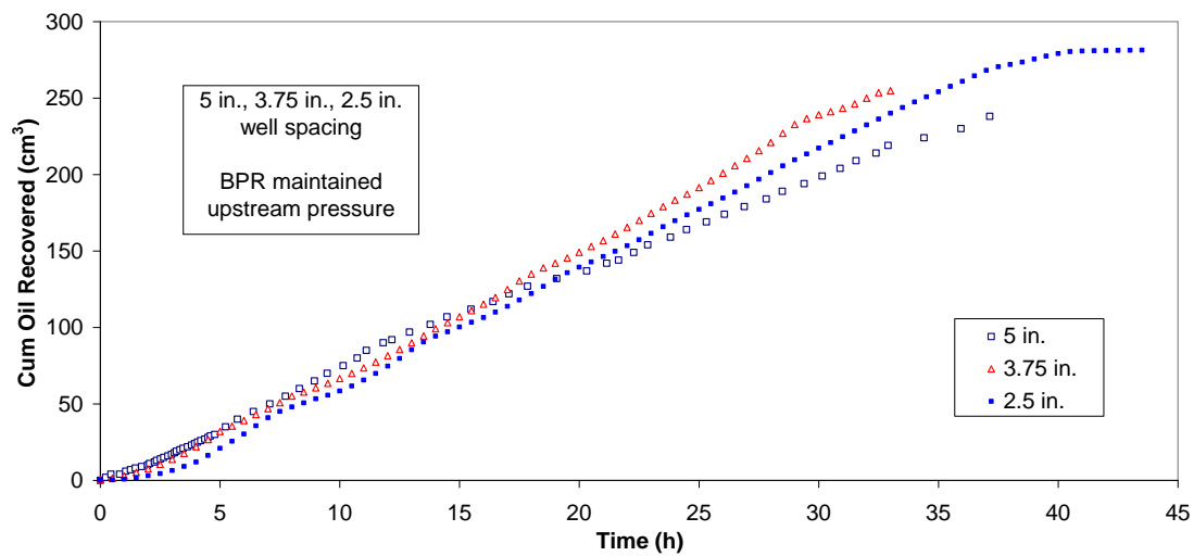
Fig. 27 – Effect of well spacing on oil recovery in VAPEX experiments
