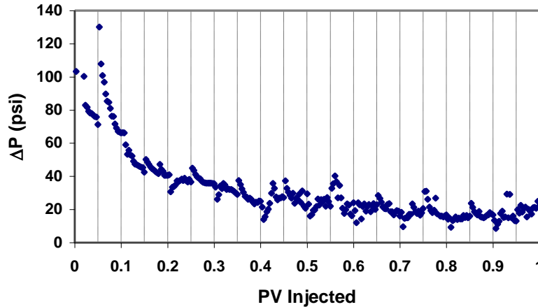
Fig. 13 – Pressure drop for WAG ratio =1 flood, slug size = 0.05 PV
