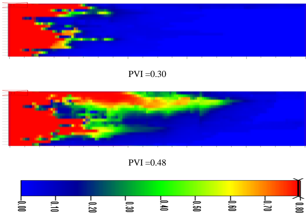
Fig. 51 - Gas saturation distribution for 2-D (X-Z) gas injection simulation with heterogeneous permeability field Perm2 ( N_g = 0.018 )
