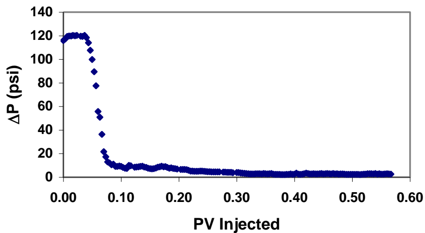
Fig. 11 – Pressure drop in coreflood during gas injection
