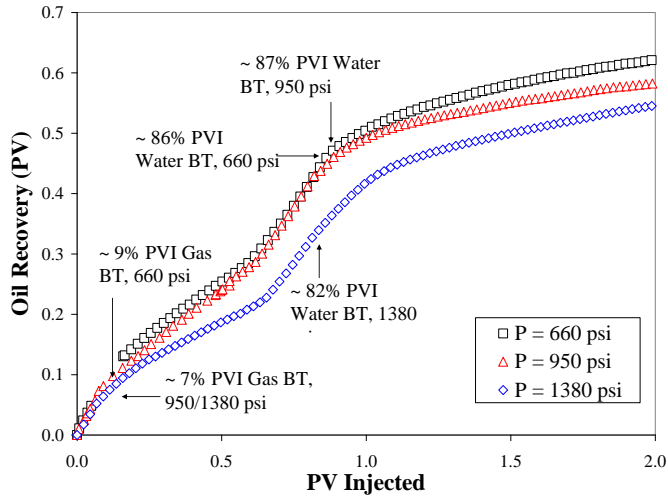
Fig. 17 – Effect of BPR pressure on gasflood oil recovery in the 5-spot model
