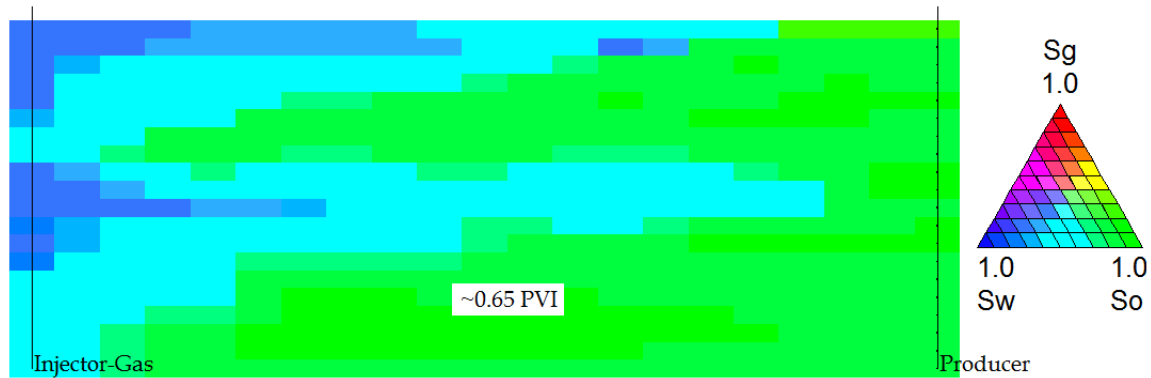
Fig. 77 - In-situ saturation distribution \sim 0.65 PVI ( k_v/k_h = 0.50 )
