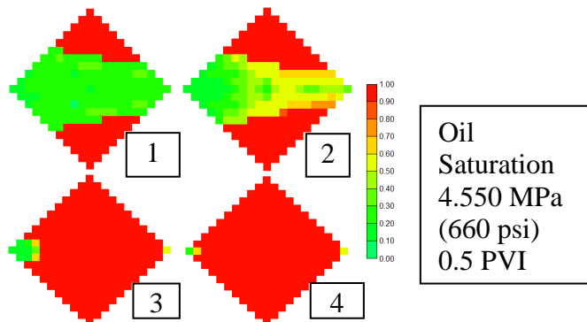
Fig. 19 – Oil saturation first 4 layers in 5-spot
