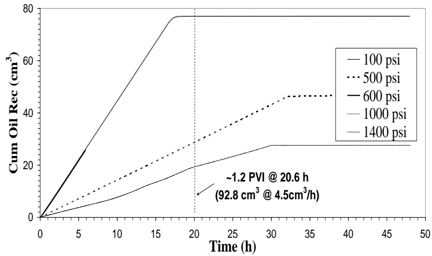
Fig. 9 – Cumulative oil recovery slimtube simulation
