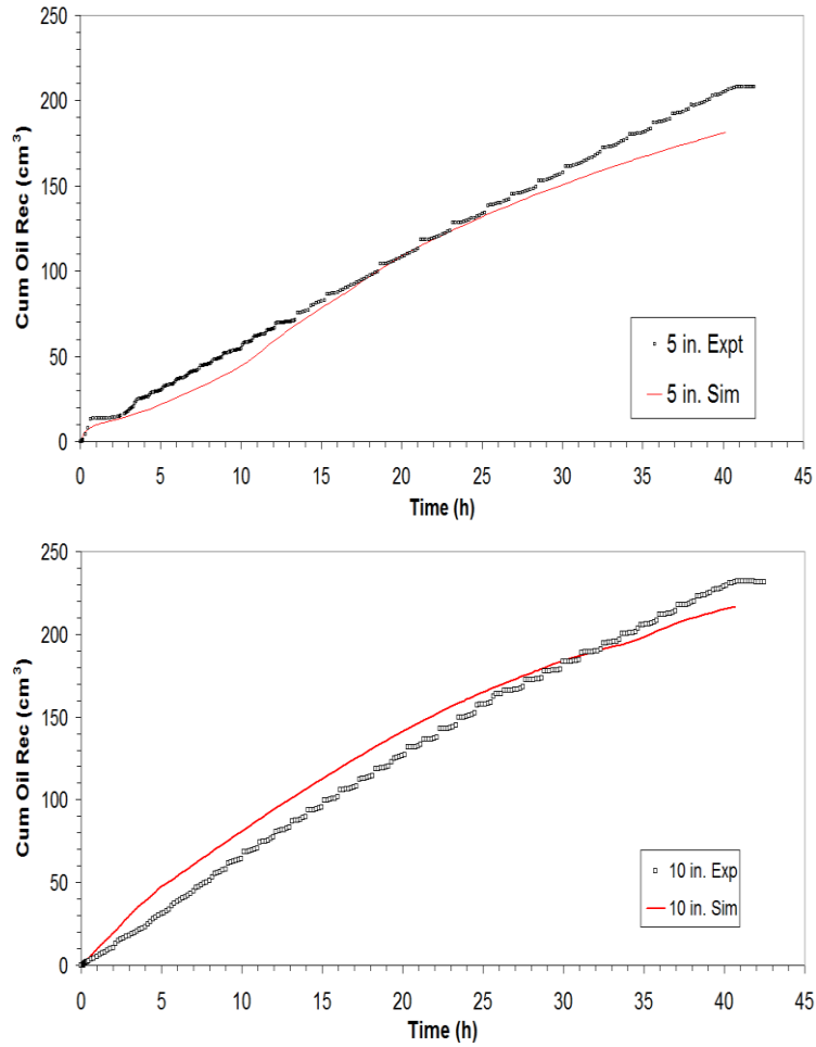
Fig. 29 – Simulated vs. experimental oil recovery in VAPEX
