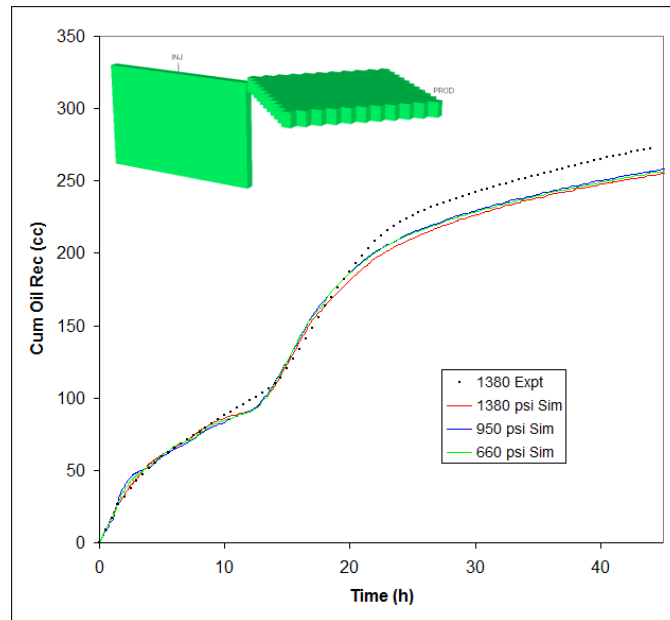
Fig. 17 – Effect of BPR pressure on gasflood oil recovery in the 5-spot model
