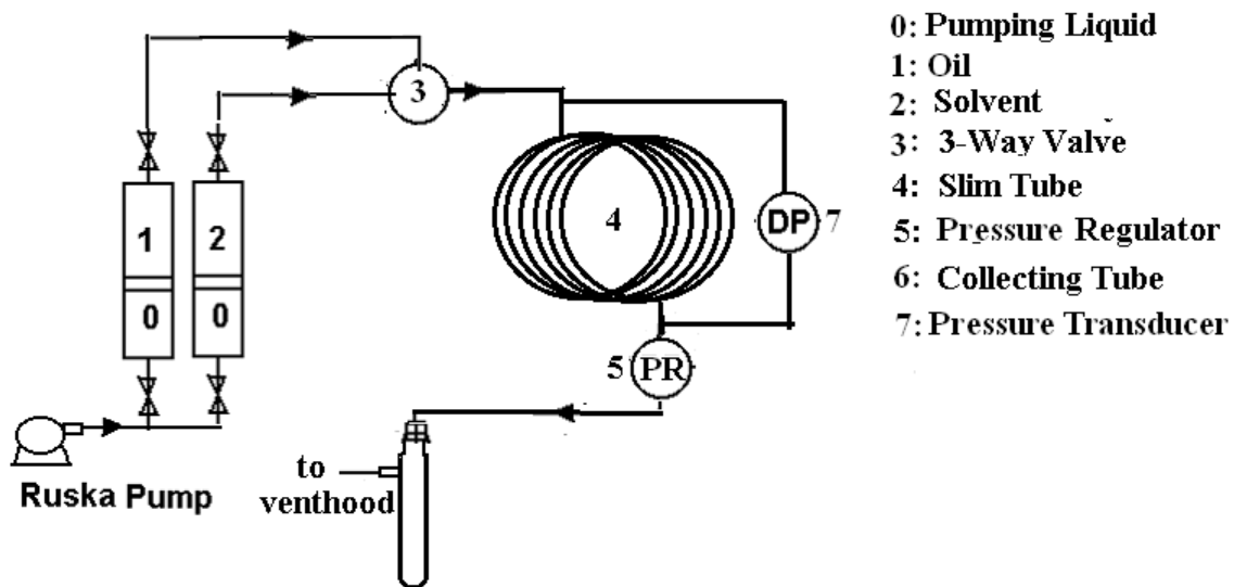
Fig. 1 - Flow loop for slim tube experiments
