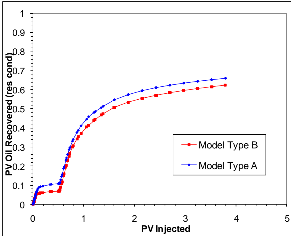
Fig. 78 - Oil Recovery A & B models, k_v/k_h = 0.5
