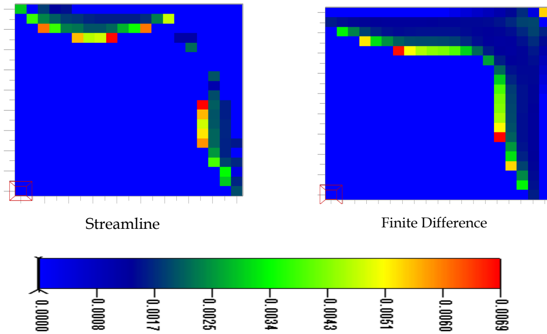
Fig. 56 - Gas saturation profiles @ 0.13 PVI for 2-D (X-Y) immiscible gas injection (3 HC phase system)
