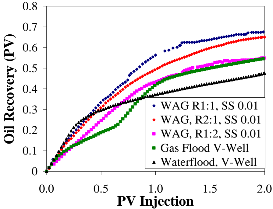
Fig. 21 – Effect of WAG ratio in the quarter 5-spot model
