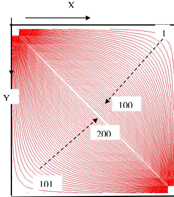
Fig. 68 - Streamlines in 2-D homogeneous gas injection (200 streamlines)
