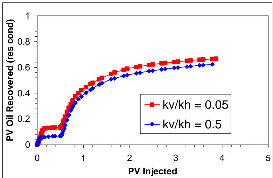
Fig. 76 - Cumulative oil recovery in the field 2D example
