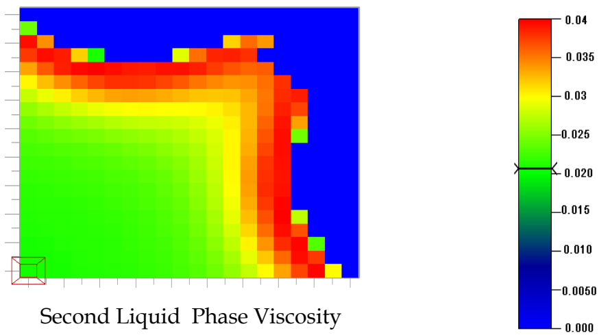
Fig. 58 - Phase viscosities at 0.13 PV injected in 2-D gas injection (3 HC phase system)
