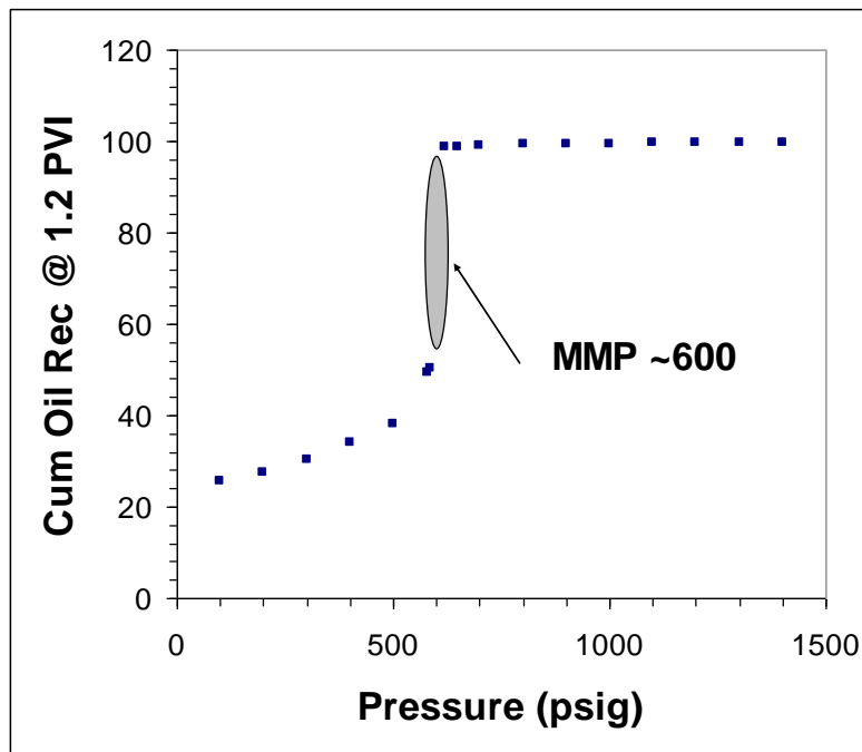
Fig. 10 – Simulated oil recovery at 1.2PVI
