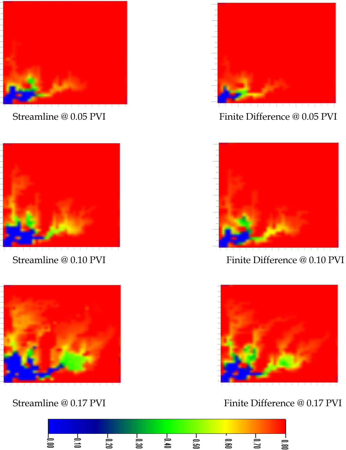
Fig. 40 - Oil saturation distribution for 2-D (X-Y) gas injection - heterogeneous
