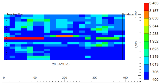
Fig. 73 - Horizontal permeability fields (Type A, B Models)
