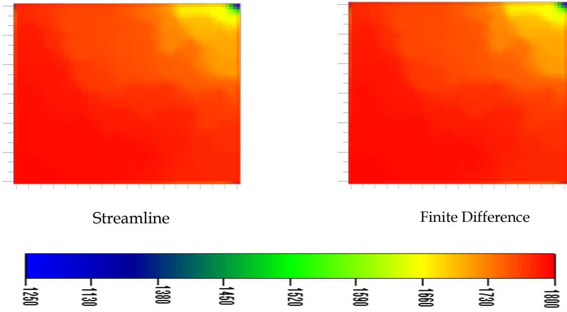
Fig. 38 - Pressure contours @ 0.10 PVI for 2-D (X-Y) gas injection - heterogeneous
