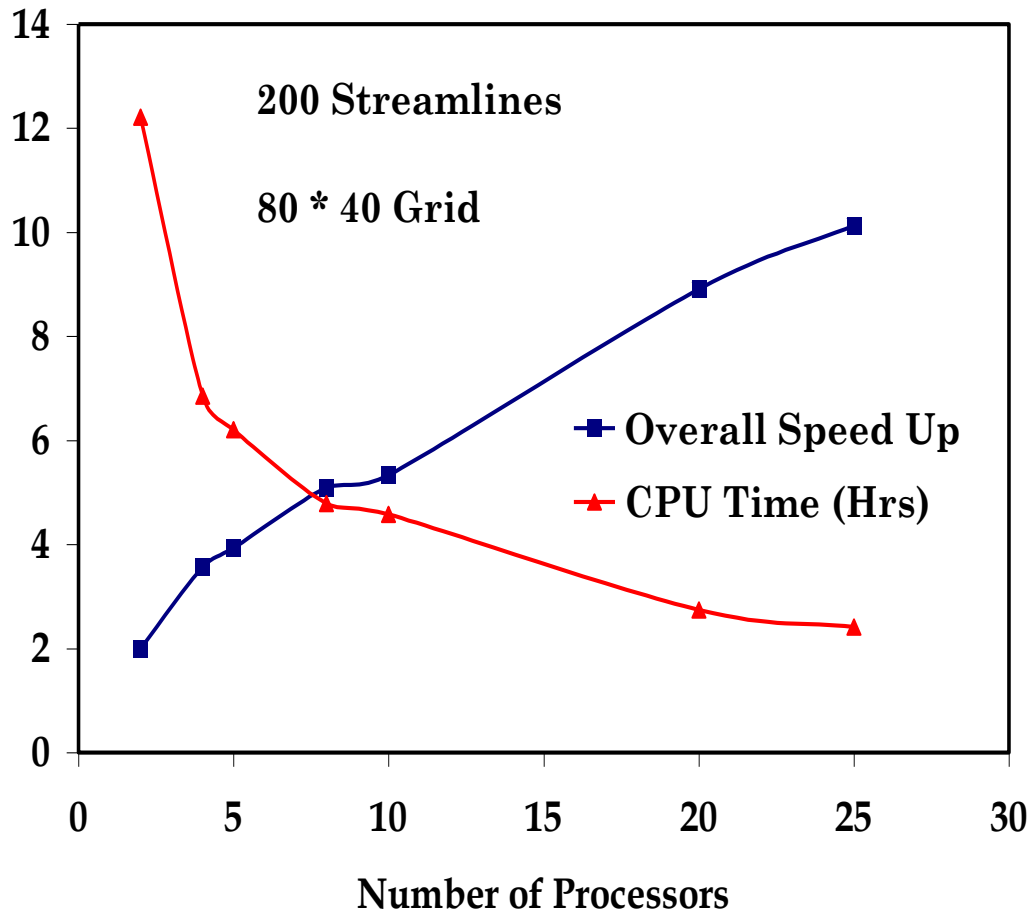
Fig. 72 - Run time and overall speed up vs. number of processors for 2-D gas injection simulation (X-Z)
