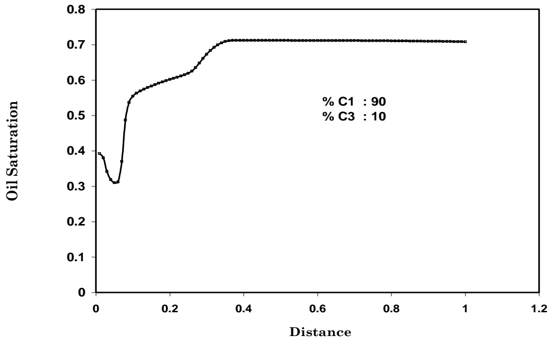
Fig. 37b - Oil saturation distribution in 1-D immiscible gas injection (with Oil 1)
