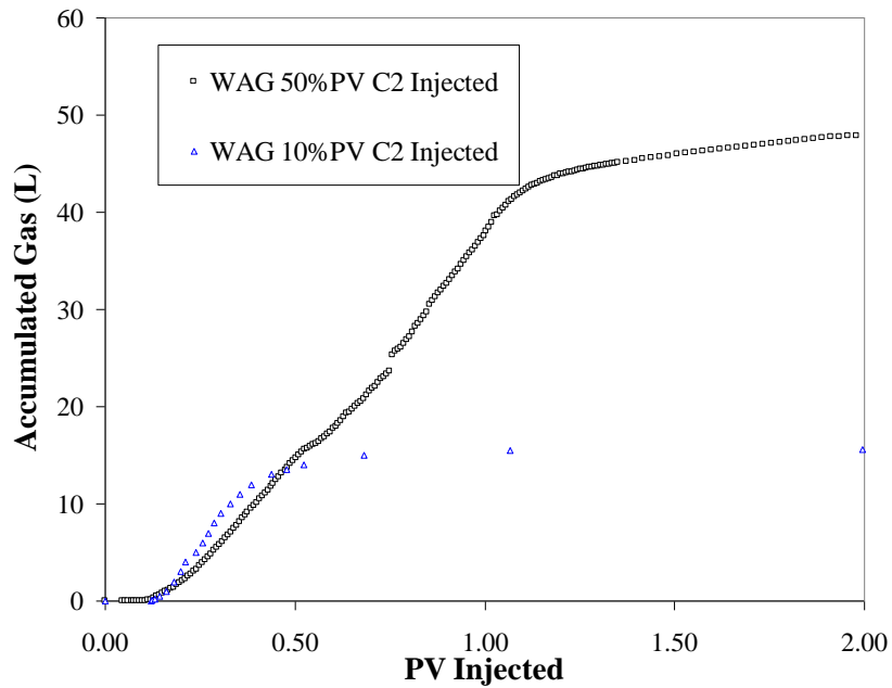
Fig. 23 - Gas production during WAG injection in the quarter 5-spot model
