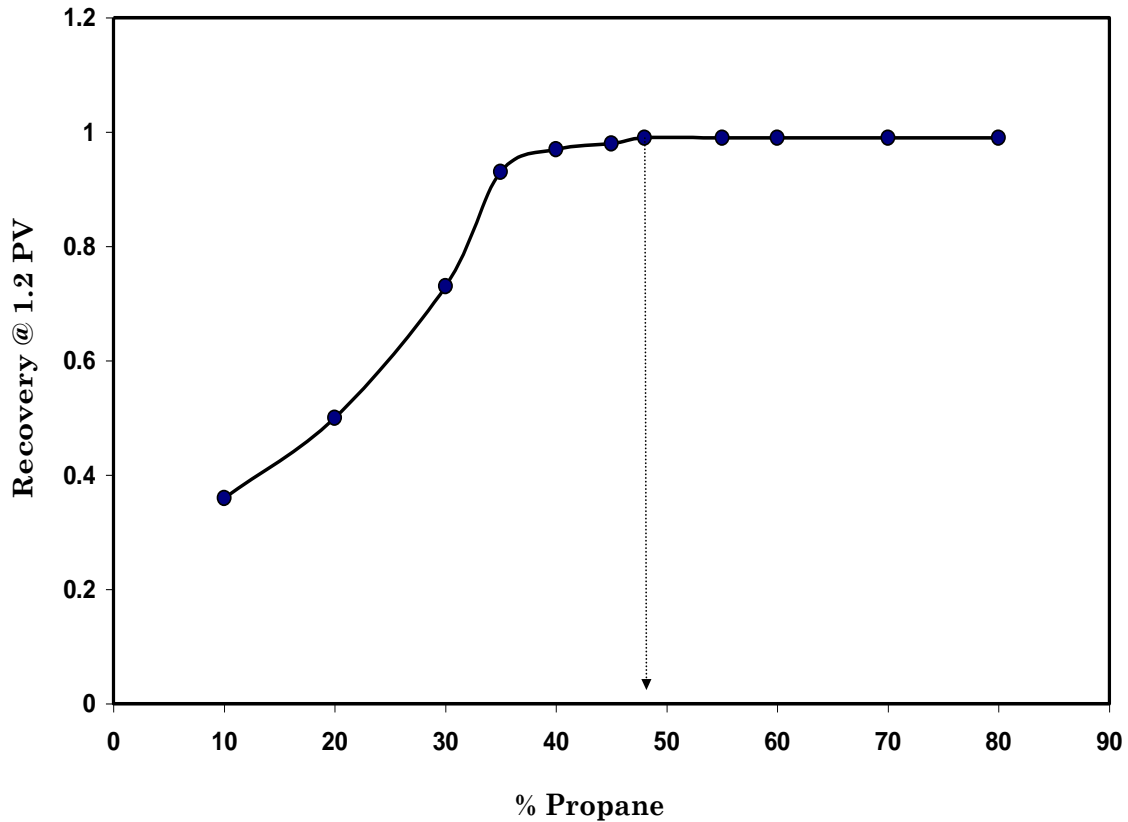
Fig. 36 - Minimum miscibility enrichment (MME) of methane with propane (Oil 1)
