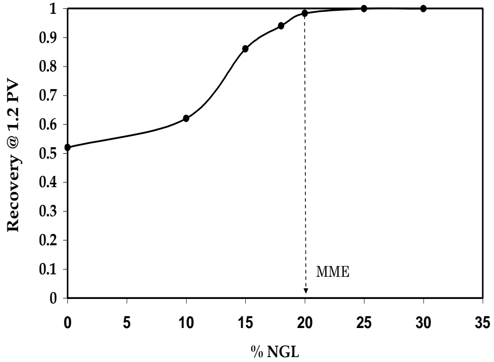
Fig. 53 - Minimum miscibility enrichment (MME) of CO 2 with NGL (Oil 2)
