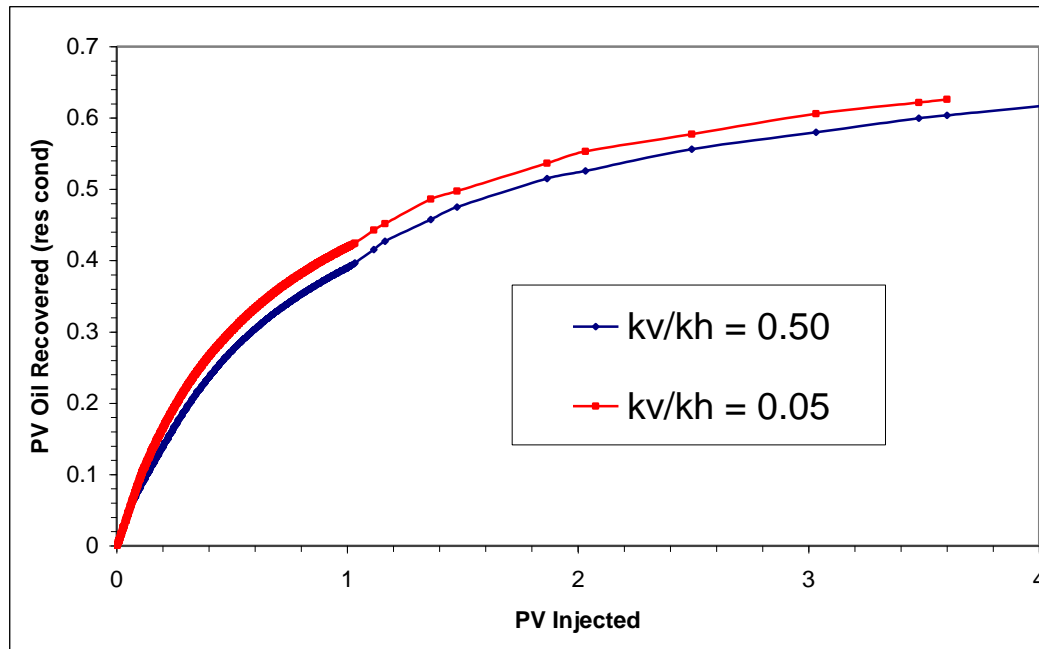
Fig. 82 - Effect of k_v/k_h on recovery in 3D WAG simulations
