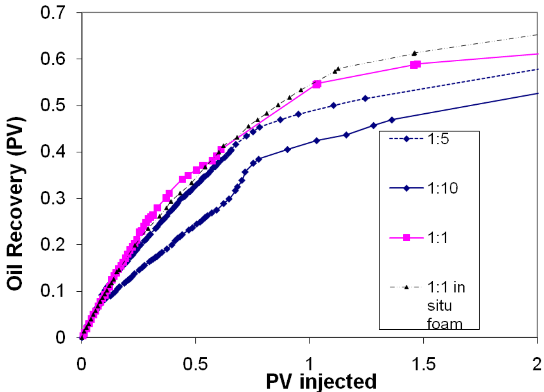
Fig. 25 – Oil recovery in foam flooding experiments in the quarter 5-spot
