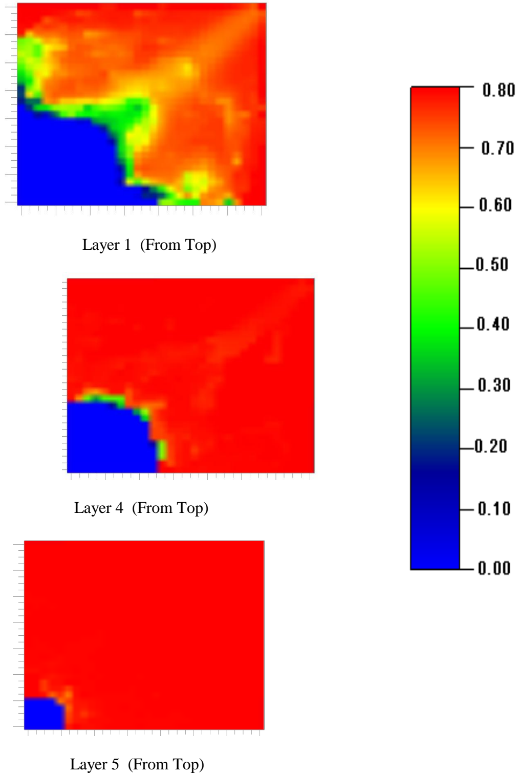
Fig. 52 - Oil saturation profiles @ 0.45 PVI for 3-D gas injection ( N_g = 0.46 )
