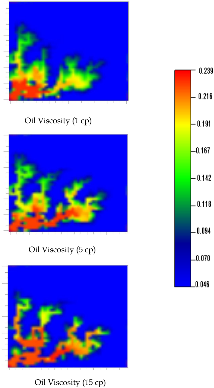
Fig. 41 - Methane concentration @ 0.16 PVI for 2-D (X-Y) gas injection: effect of oil viscosity
