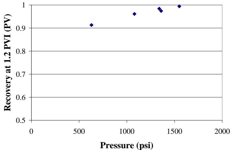
Fig. 8 – Slimtube recovery at 1.2 PV solvent injection
