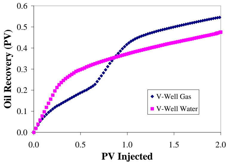
Fig. 15 – Oil production in the 5-spot model
