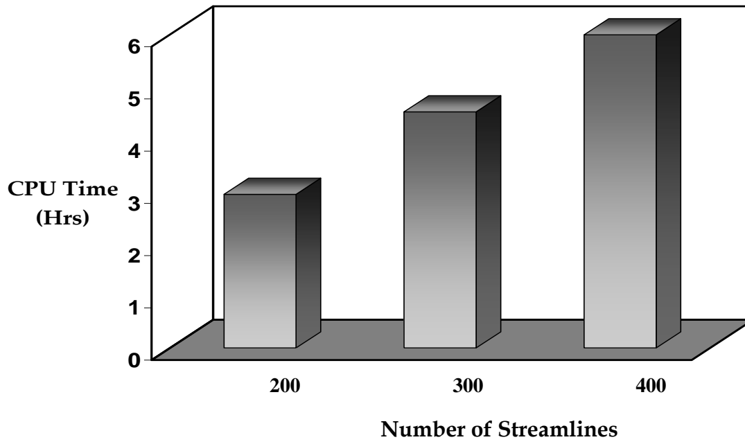
Fig. 69b - Flash calculation time on a single processor for different number of streamlines
