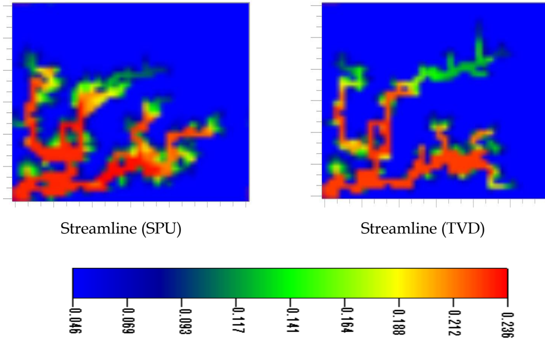
Fig. 45 - Comparison of methane concentration distribution @ 0.20 PVI in 2-D (X-Y) heterogeneous miscible gas simulation: effect of numerical schemes
