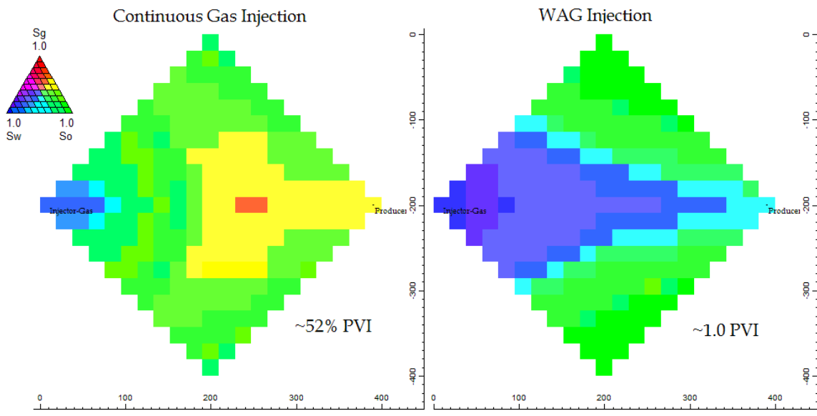
Fig. 84 - In-situ saturation distribution; continuous gas vs. WAG (x-y view)
