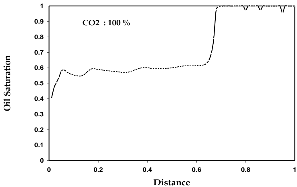
Fig. 54a - Oil saturation distribution in 1-D immiscible gas injection (with Oil 2)
