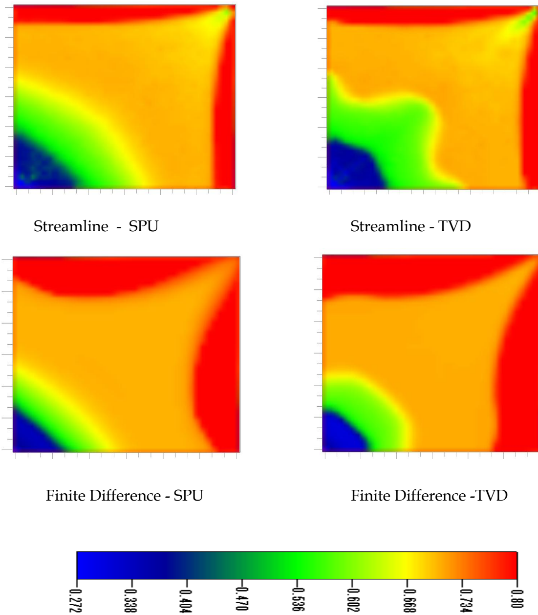
Fig. 44 - Comparison of oil saturation distribution @ 0.17 PVI in homogeneous 2-D
