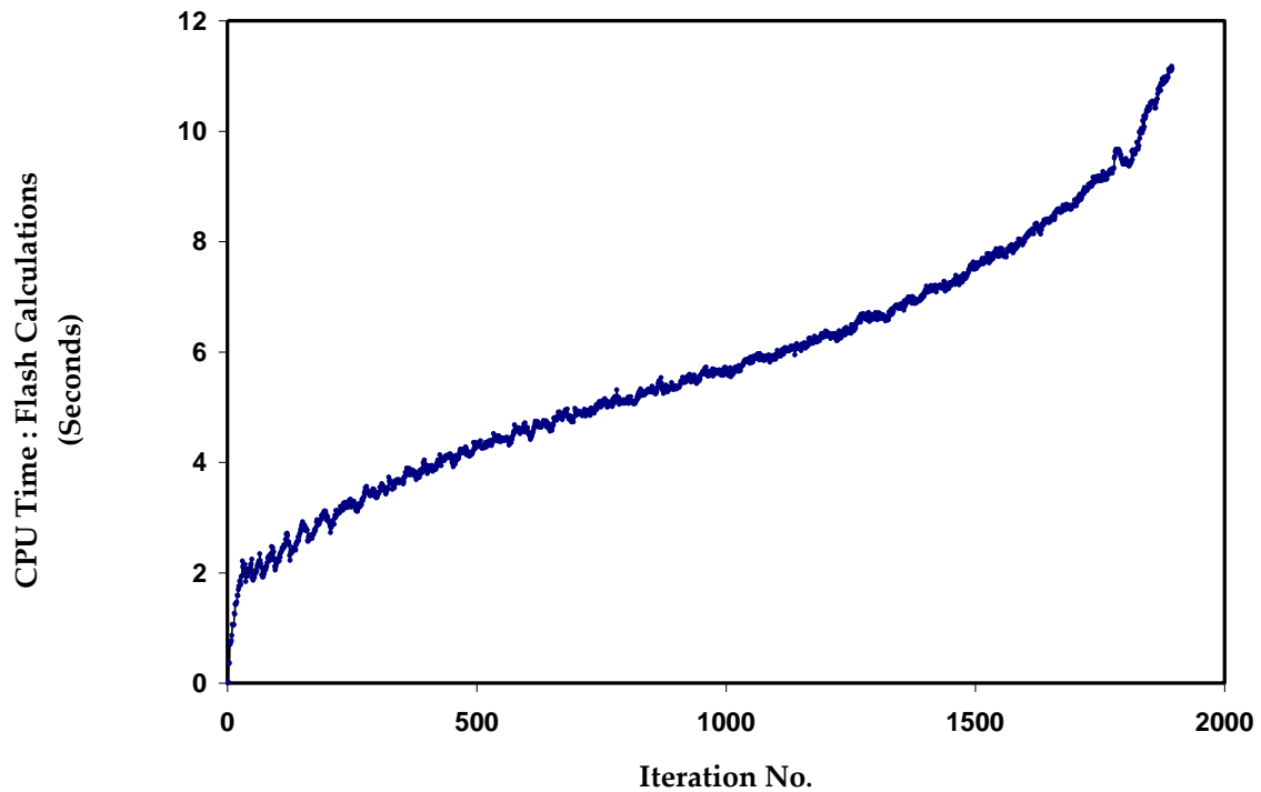
Fig. 63 - CPU time spent in flash calculations per global time step
