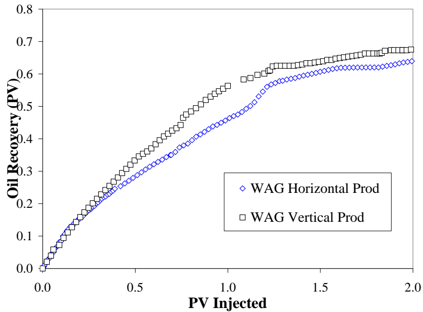
Fig. 24 – Effect of horizontal production well in WAG injection in the quarter 5-spot model
