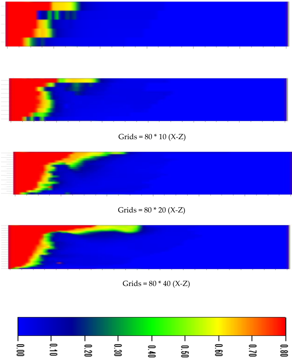
Fig. 47 - Gas saturation profile @ 0.25 PVI for 2-D homogeneous (X-Z) gas injection: effect of number of grids in the vertical direction ( N_g = 0.186 )
