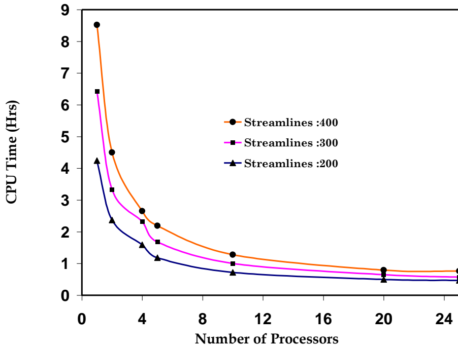
Fig. 70 - Run time vs. number of processors with different number of streamlines
