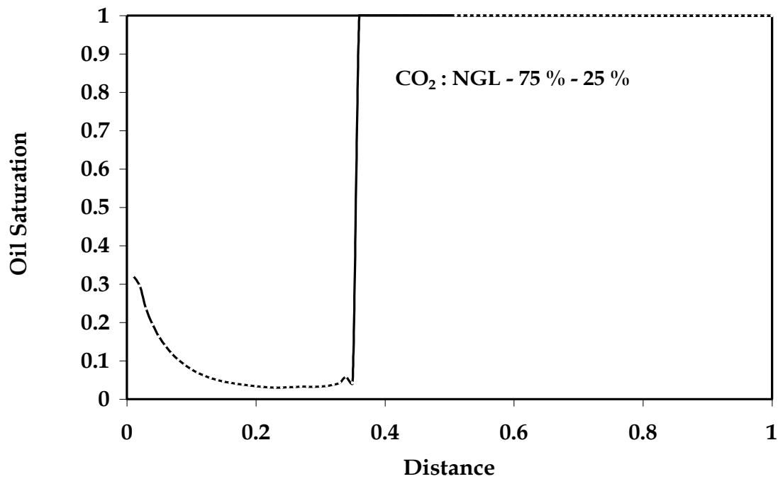
Fig. 54b - Oil saturation distribution in 1-D miscible gas injection (with Oil 2)
