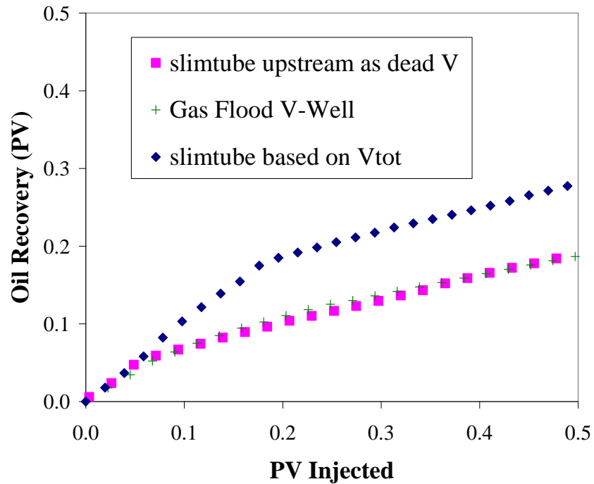
Fig. 16 – Comparison of gasfloods with and without an upstream slimtube
