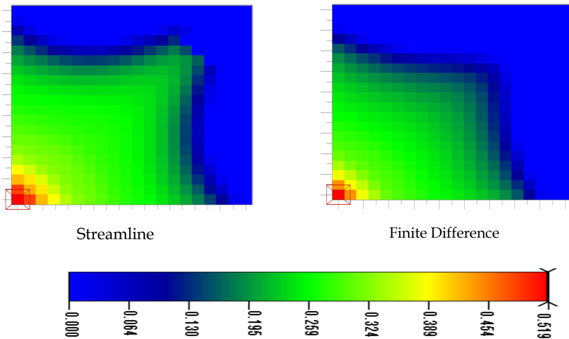
Fig. 57 - Second liquid phase saturation profiles @ 0.13 PVI for 2-D (X-Y) immiscible gas injection (3 HC phase system)
