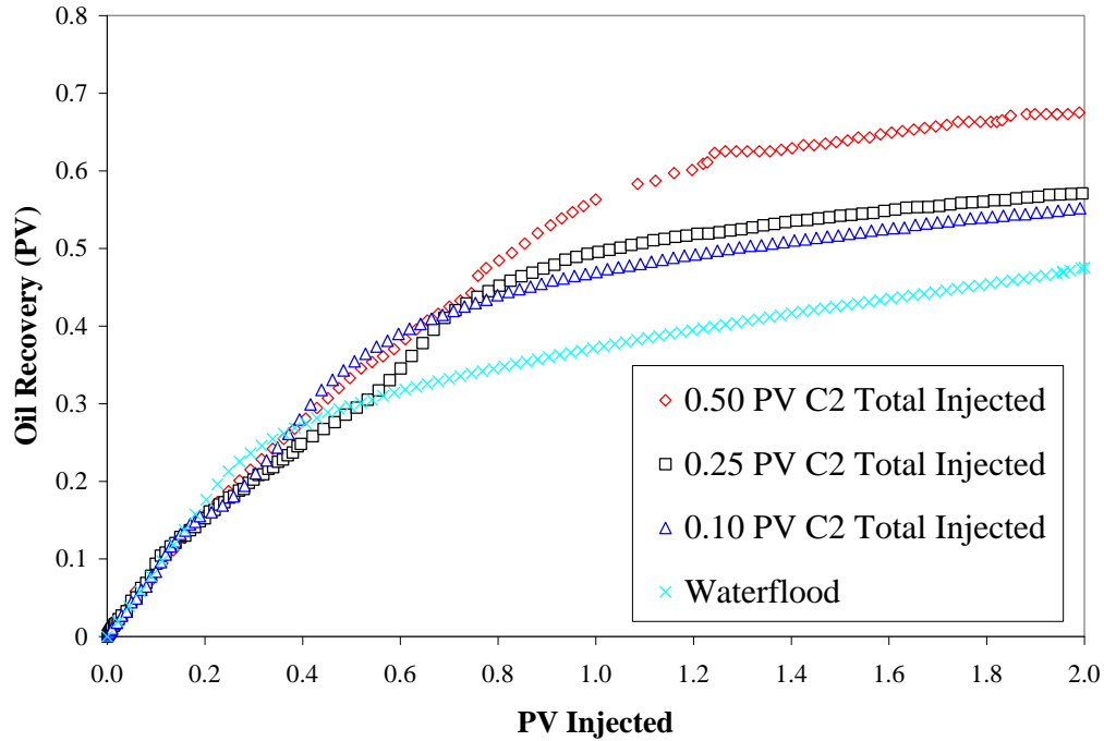
Fig. 22 – Effect of solvent amount in WAG injection in the quarter 5-spot model
