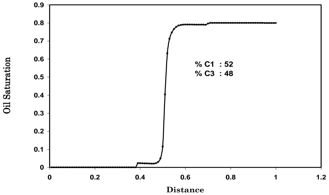
Fig. 37a - Oil saturation distribution in 1-D miscible gas injection (with Oil 1)
