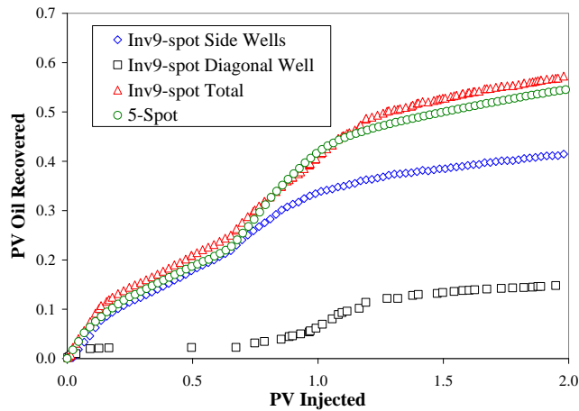
Fig. 20 – Comparison of oil recovery between an inverse 9-spot and 5-spot models
