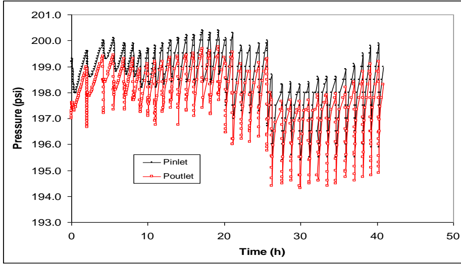
Fig. 31 – Injector and producer pressures in VAPEX: 10 in. run
