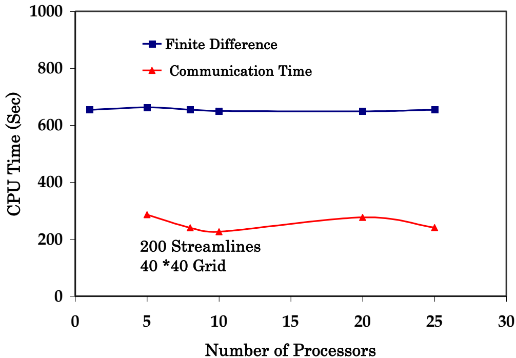
Fig. 65 - Finite difference and communication time vs. number of processors
