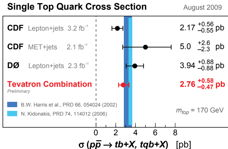
Figure 3: Tevatron single top cross section measurements and their combination.
