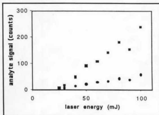
Fig. 2. Dependence of analyte signals on laser pulse energy for Sr (circles) and Fe (boxes). Similar results were obtained for other elements.
