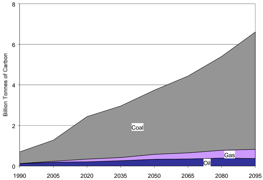
Figure 10. CO 2 Emissions by Fuel – China Reference Case (Billion Tonnes of Carbon)
