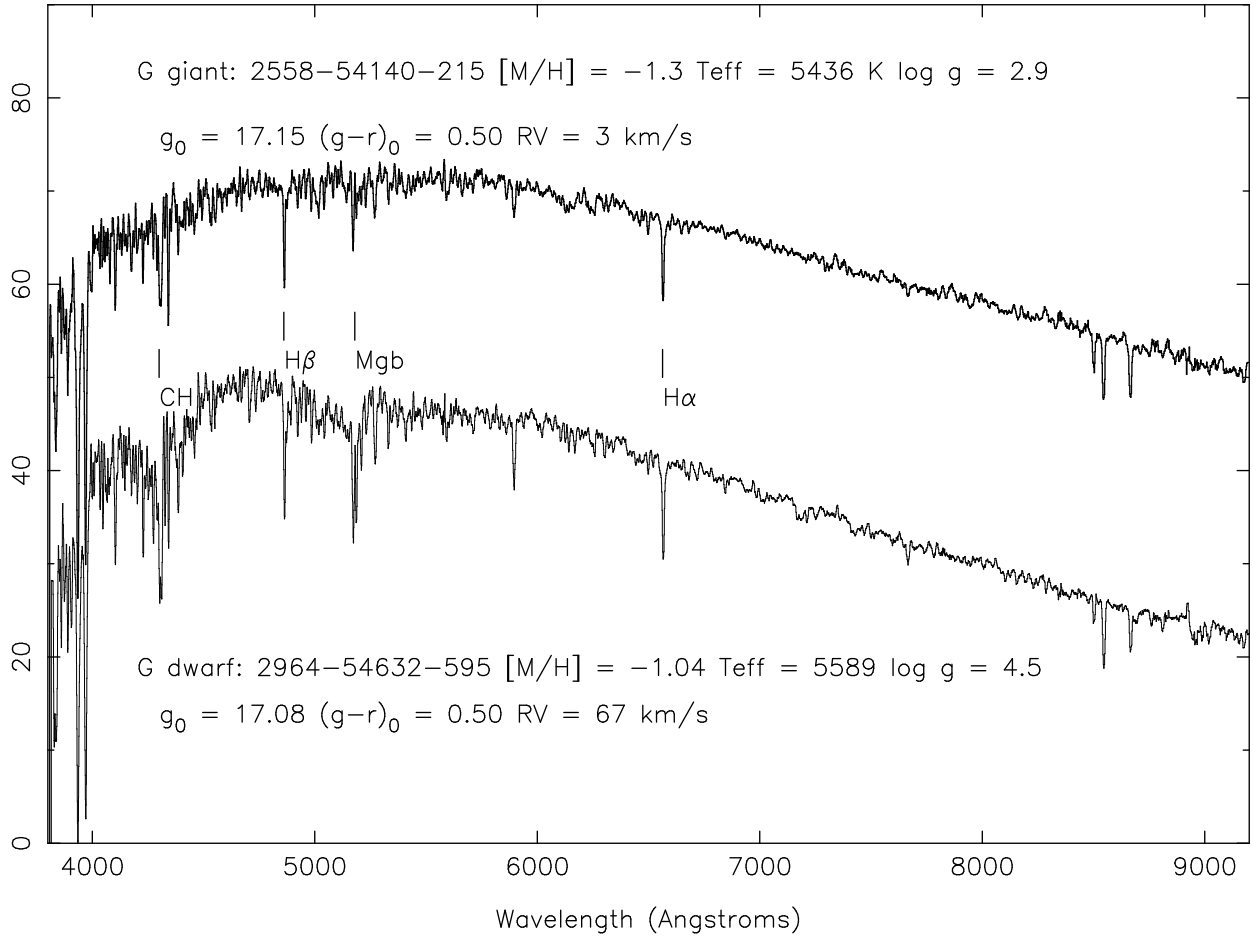
Fig. 9.— Upper: the weak Mgb/H feature at \lambda 5140 indicates that this G star is actually a higher luminosity evolved subgiant, on its way up the red giant branch. Approximately 7% of the SEGUE G star sample shows low surface gravity. Lower: a more typical G dwarf star.
