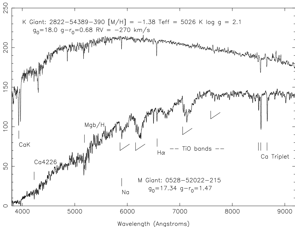
Fig. 11.— Top: a sample SEGUE K giant star, weak Mgb/H feature, the weak Ca 4226 and the weak Na I \lambda 5890 . Bottom: a sample SEGUE red K giant star. Even though this spectrum shows strong TiO bands, usually found in early M dwarfs, it is clearly a giant, due to its relatively weak Mgb/H , nearly absent Na I \lambda 5890 , weak Ca \lambda 4226 , and strong Ca IR triplet. This star has an absolute M_g = -1 and is at a distance of 45 kpc from the Sun in the Sagittarius tidal stream’s Northern leading tail.
