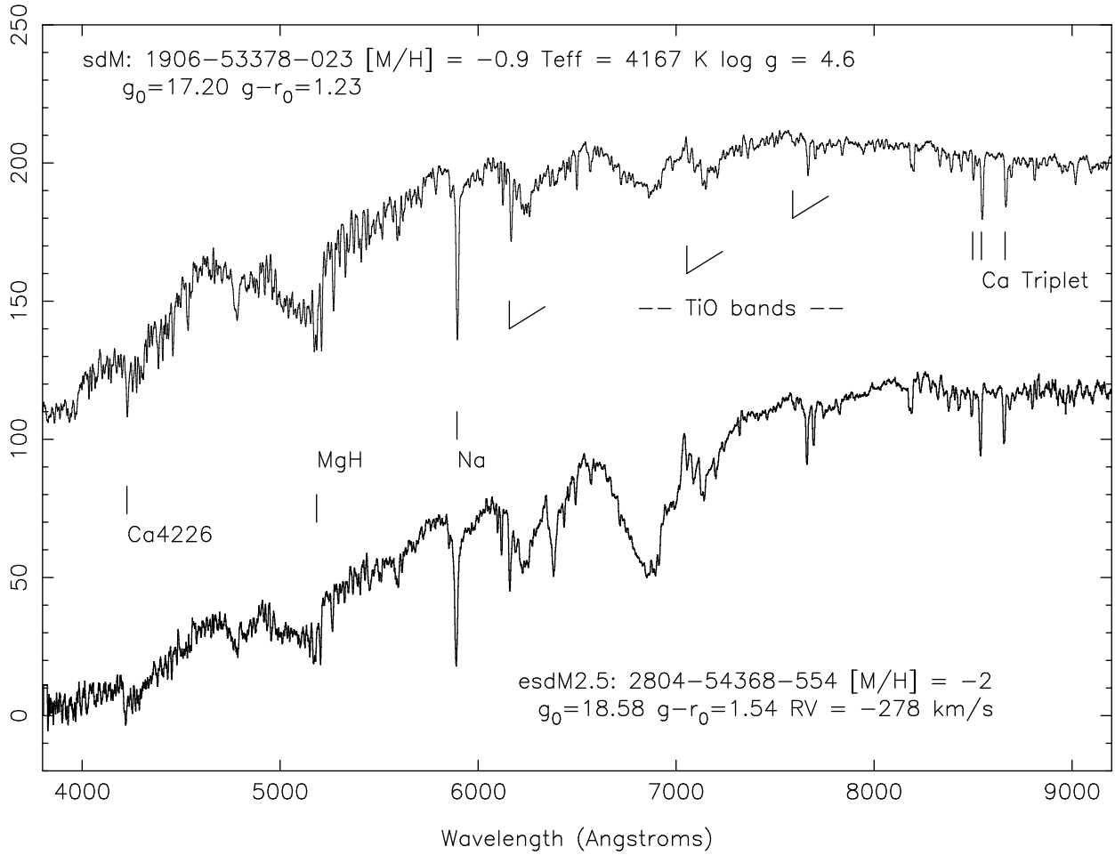
Fig. 13.— a sample SEGUE M subdwarf, the SEGUE estimate of metallicity is uncertain at these cool temperatures. An AMNH proper motion and color selected SEGUE esdM2.5 extreme subdwarf. Note that the TiO bands are nearly gone.
