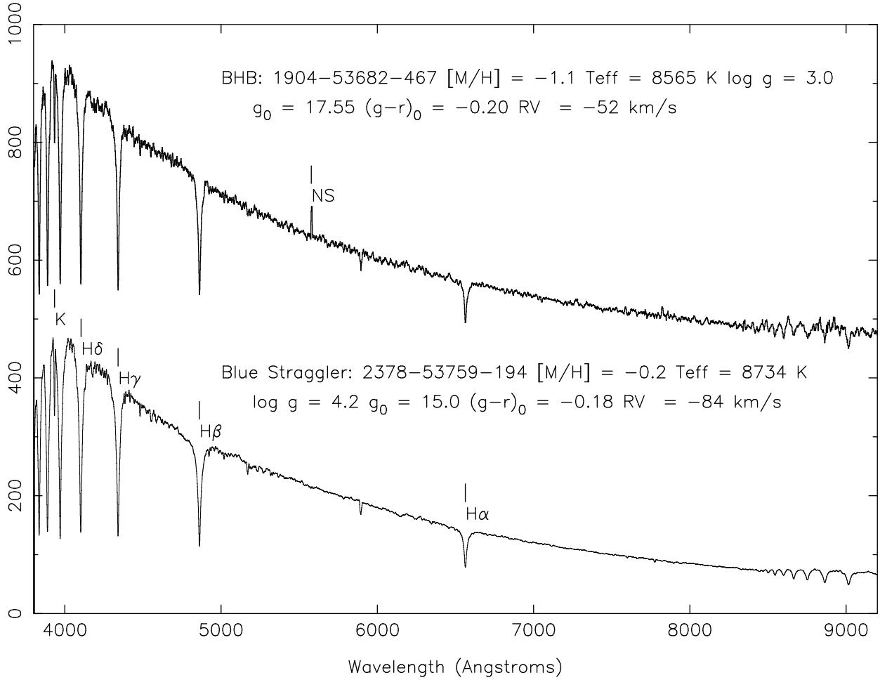
Fig. 6.— Upper: a sample SEGUE BHB star. Note the low surface gravity, \log g = 3.0 , deep and narrow Balmer lines characteristic of this type. Lower: a sample SEGUE BS star. Note the somewhat broader Balmer lines, the strong Paschen series lines in the IR and the higher measured surface gravity \log g = 4.2 .
