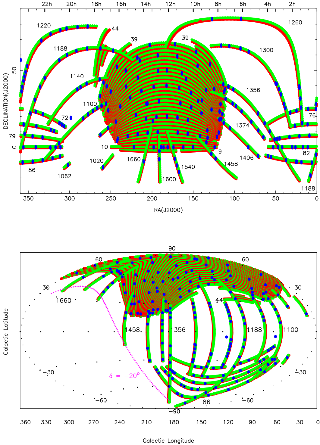
Fig. 1.— Upper panel: the SEGUE Survey footprint in the Equatorial coordinates from 360^\circ to 0^\circ (left to right) and -26^\circ to 90^\circ (bottom to top). Selected stripes are labeled with their stripe number. The SDSS North Galactic Cap stripes are numbered from 9 to 44. Southern SDSS stripes are numbered 76, 82 and 86. SEGUE fills in Southern stripes 72 and 79. SEGUE’s constant Galactic longitude stripes are numbered with stripe = 1000 + 2l where l is the Galactic longitude. Each SEGUE plate pointing (usually representing a pair of 640 hole plates), is indicated with a blue circle. Lower panel: the SEGUE Survey footprint in (l, b) in Aitoff projection, centered on the Galactic anticenter. The line marking the Southern limit of the telescope observing site \delta = -20^\circ is indicated in magenta. Red and green filled areas represent South and North SDSS and SEGUE strips respectively.
