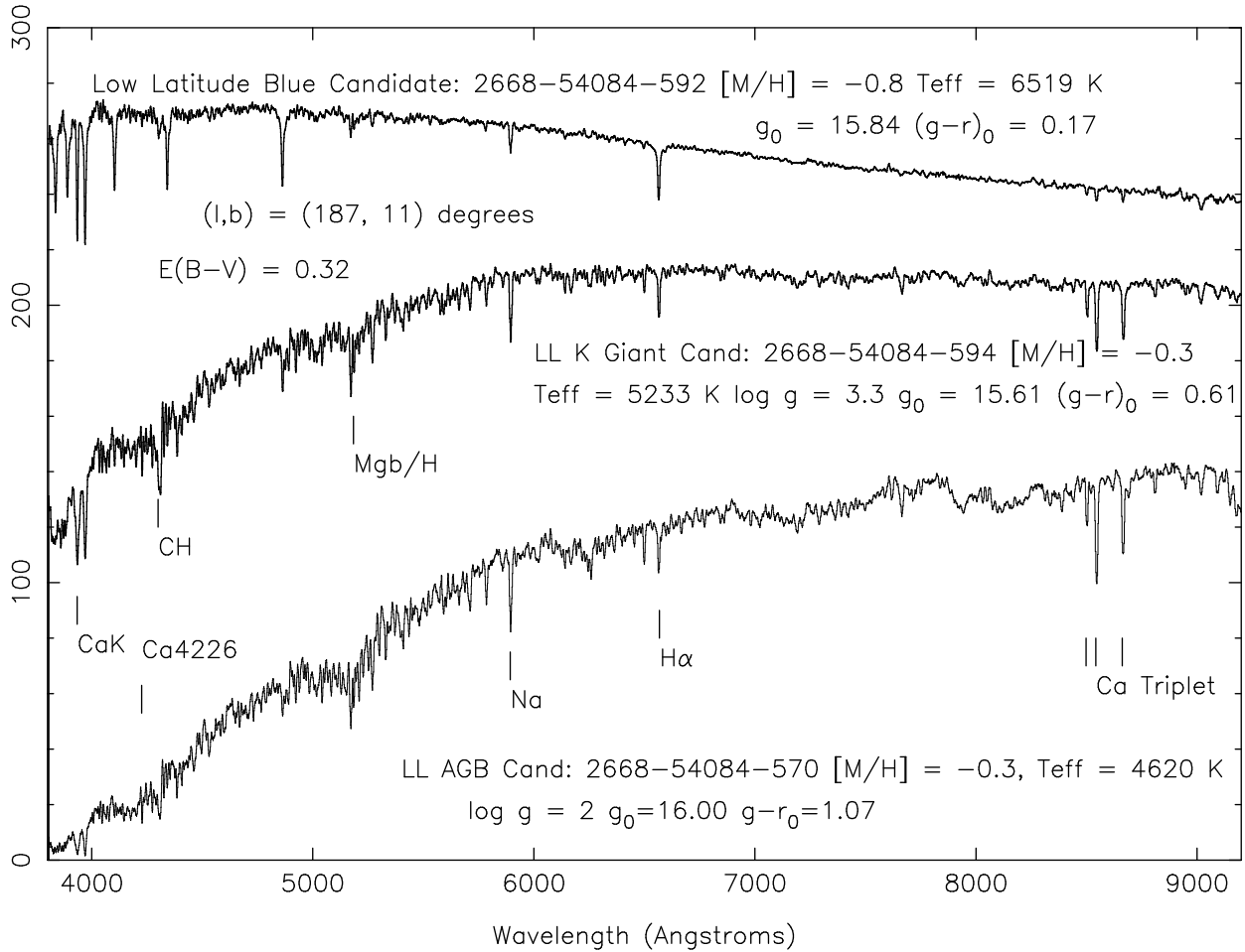
Fig. 16.— a sample of three SEGUE low-latitude target-selection objects from the same SEGUE plate. Upper: a blue-tip candidate object, clearly of spectral type F. Middle: a K giant candidate. Lower: a candidate AGB object.
