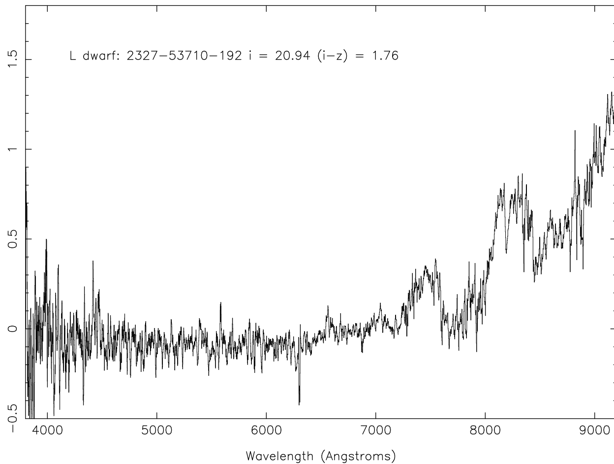
Fig. 15.— a sample SEGUE brown dwarf of approximate spectral type L0 (or M9). The u , g and r band flux is nearly completely missing from these objects.
