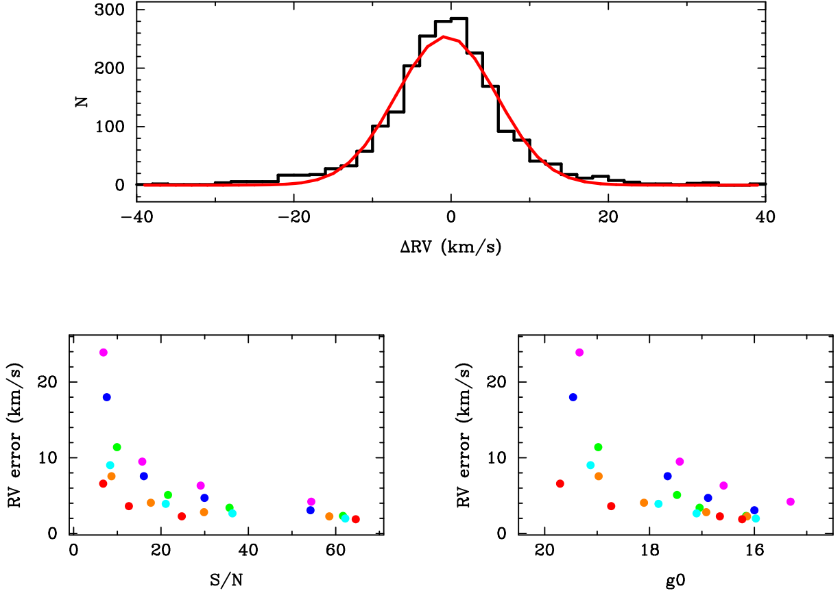
Fig. 2.— top panel shows the histogram of differences in spectroscopic pipeline measurements of RV for two separate observations of the same star on different survey SEGUE plates for 2200 stars with r \sim 18 and S/N > 10 . The quoted sigma is divided by \sqrt{2} to estimate the measurement error for a single observation. The red curve is the best fit Gaussian, it has a mean offset of < 0.3 \text{ km s}^{-1} and a \sigma/\sqrt{2} = 4.4 \text{ km s}^{-1} . Lower panel: RV accuracy by S/N and (g-r)_0 color. The color code is magenta: (g-r)_0 < 0.1 (BHB/BS/A), blue: 0.1 < (g-r)_0 < 0.3 (F), green: 0.3 < (g-r)_0 < 0.48 (F/G), cyan: 0.48 < (g-r)_0 < 0.55 (G), orange: (0.55 < (g-r)_0 < 0.75 (G/K) and red: 0.75 < (g-r)_0 < 1.0 (K).
