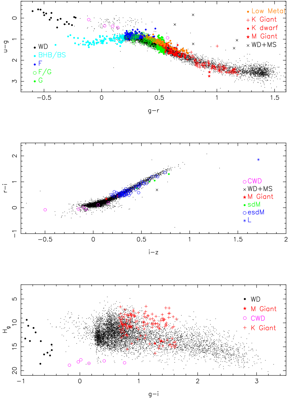
Fig. 3.— target selection categories in SEGUE. Top panel: (g-r)_0, (u-g)_0 color-color diagram showing different SEGUE target categories in different colors/symbols. Note the ‘Low Metal’ category hugs the blue side (in (u-g)_0 ) of the stellar locus, and a substantial fraction of F stars with redder (u-g)_0 and 0.2 < (g-r)_0 < 0.48 are not targeted, except by the F/G category. Middle panel: the same as above, except categories which use redder (i-z)_0, (r-i)_0 colors are highlighted. Note the L dwarf candidate at (i-z, r-i)_0 = (1.72, 1.9) . The proper motion selected extreme M subdwarf candidates are shown as open blue circles. Lower panel: a (g-i)_0, H_g selection diagram for categories which use USNO-B proper motion in their selection. H_g = g + 5 \log_{10}(\mu/1000) + 5 where \mu is the proper motion in mas yr^{-1} . Note the cool WD candidates (high proper motion) as magenta circles and the K giant candidates (consistent with 0 proper motion).
