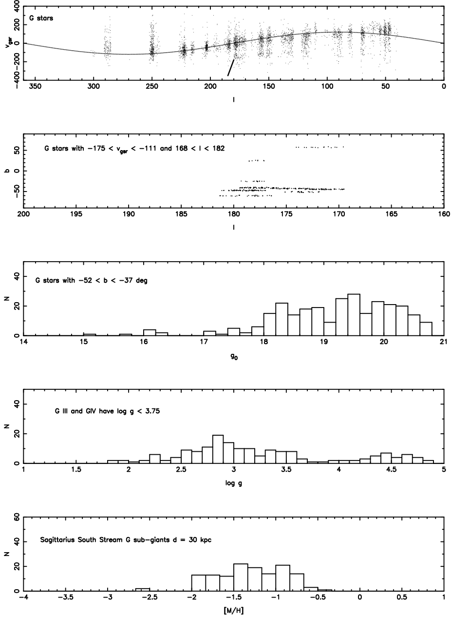
Fig. 17.— the five panels here show a step-by-step analysis of the SEGUE G star spectroscopic sample to isolate an interesting subpopulation. Top: (l, v_{gsr}) plot of 61,343 measured SEGUE G star parameters from the CAS database. A sinusoidal line, representing a rotating thick disk population is indicated with a black curve. Subsets of stars which stand out from the black curve are candidate halo dwarf galaxy or stream structures. A feature of interest for further study is highlighted with a black mark pointing to (l, v_{gsr}) = (170^\circ, -160 \text{ km s}^{-1}) . There are several other interesting features which will not be explored further here. Second from top: the set of stars selected in (l, v_{gsr}) is plotted in (l, b) to localize the interesting structure in position on the sky. Middle: the magnitude distribution of these stars is quite broad, centered near g \sim 19 , but covering in excess of a 2 mag range. It is possible that they are all at the same approximate distance only if we are sampling a steep subgiant branch population. Second from bottom: a histogram of the SSP measured surface gravity of this sample indicates that nearly all these objects ( \log g < 3.75 ) are in fact subgiants rather than dwarfs. Bottom: the metallicity distribution of these objects indicates a metallicity of [M/H] = -1.4 \pm 0.5 , with individual object errors on metallicity of about 0.3. The implied distance to these objects, if they are one population, is about 30 kpc. The spatial location of these objects is consistent with previous studies of the Sagittarius tidal stream Southern trailing tail.
