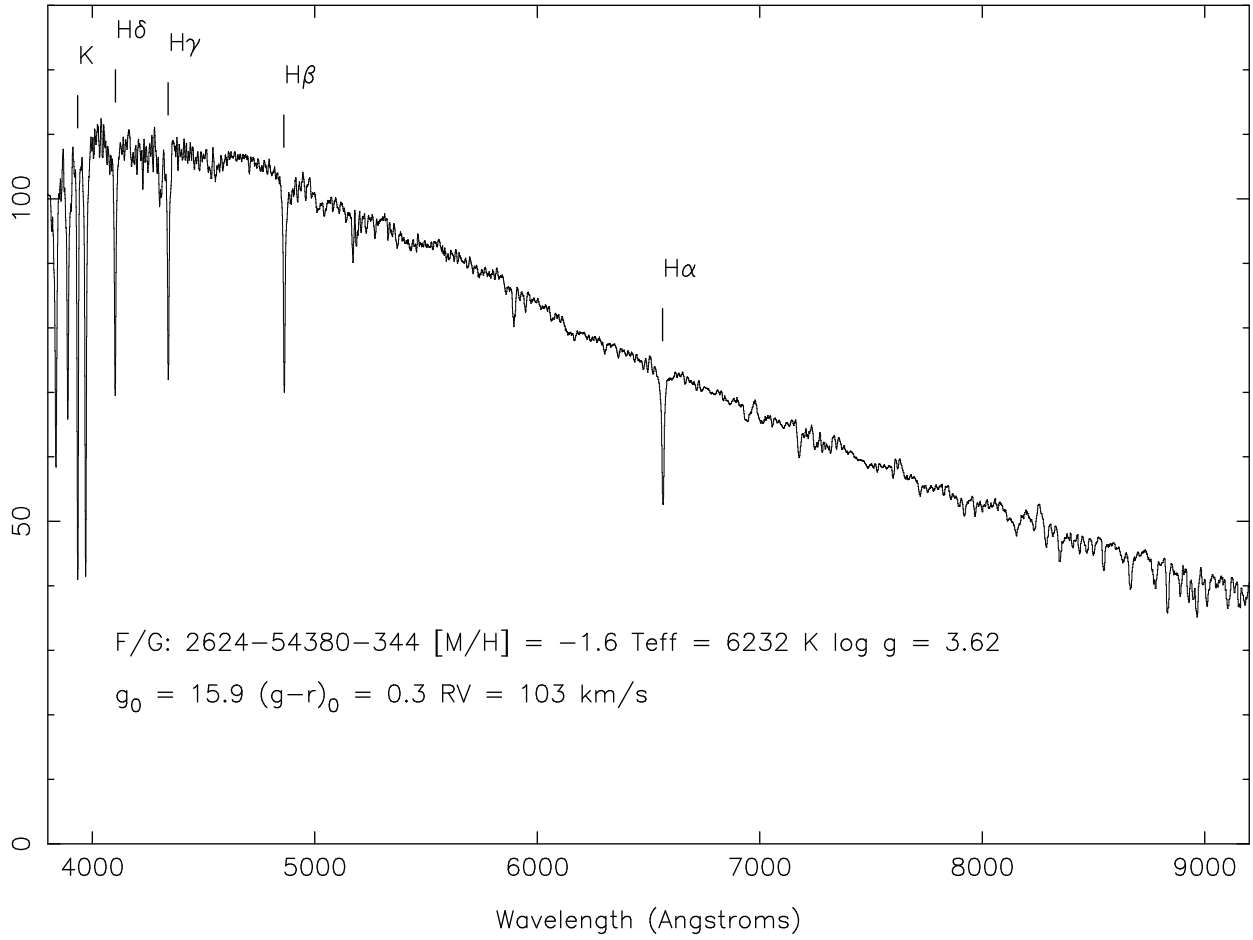
Fig. 8.— a sample SEGUE F/G star. This category samples with only a simple (g-r)_0 color cut, and is therefore nearly unbiased.
