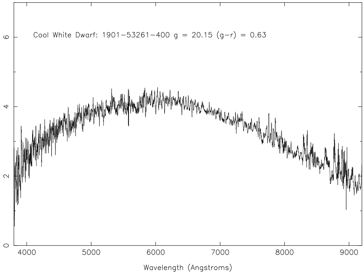
Fig. 5.— sample SEGUE cool WD where CIA due to H_2 has removed flux redward of 6000\text{\AA} , leaving a spectrum with very unusual colors.
