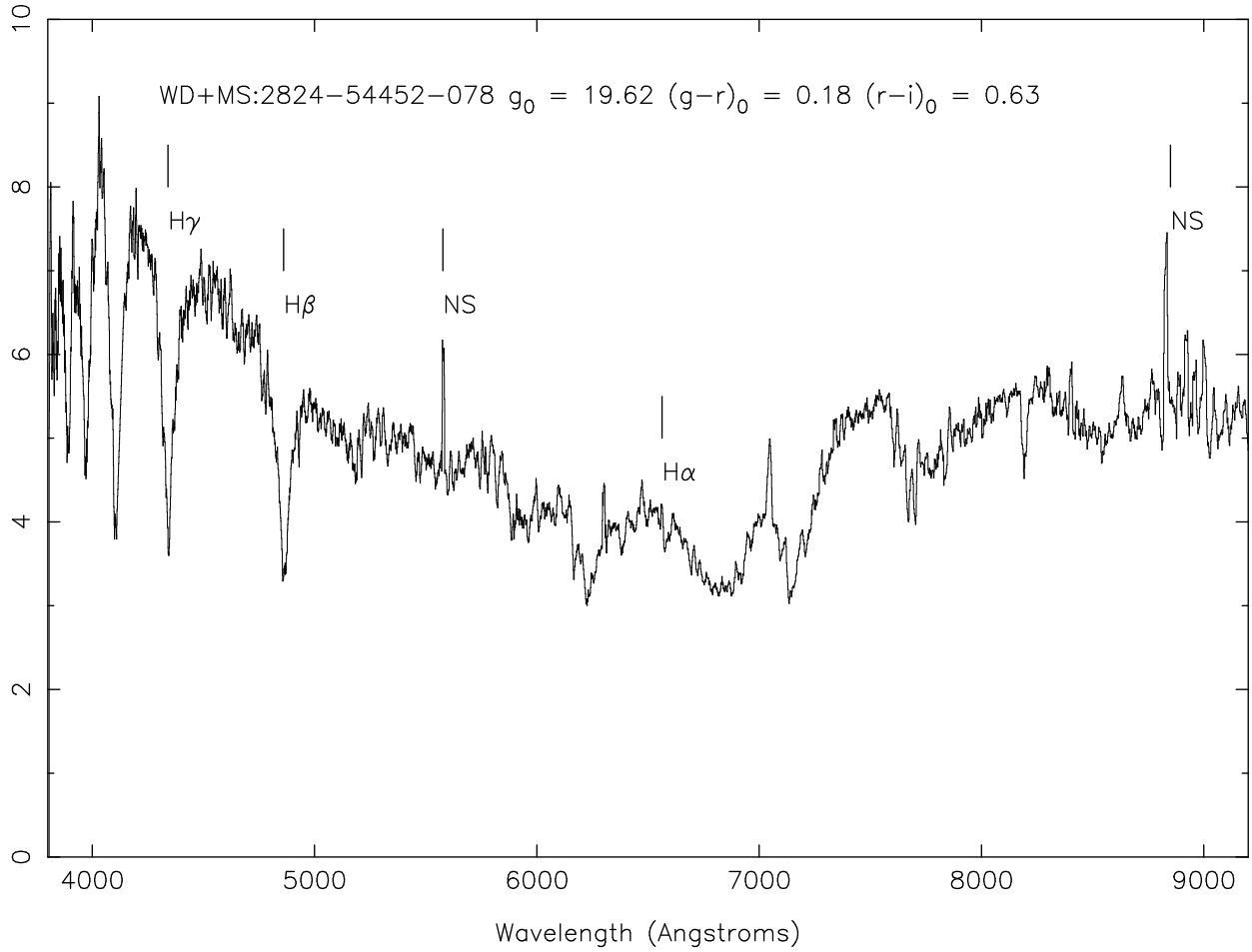
Fig. 14.— a sample SEGUE WD plus MS binary. Stellar parameters determined from modeling the SEGUE data are a WD of T_{\text{eff}} \sim 19000 K, a WD mass of \sim 0.6 M_{\odot} and a spectral type M4 for the companion.
