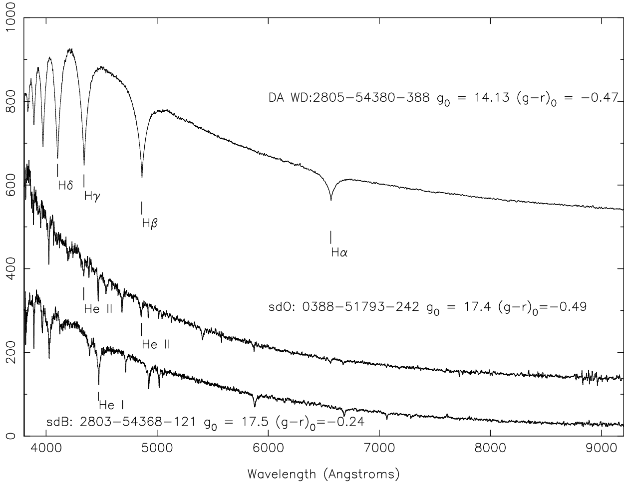
Fig. 4.— top: a sample SEGUE DA (hydrogen) WD. middle: a candidate sdO star showing a characteristic hot spectrum. lower: a candidate sdB star, which has colors similar to the WD.
