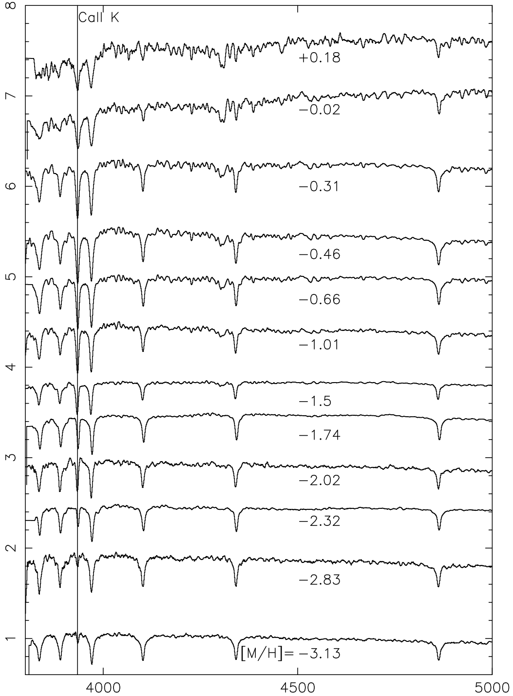
Fig. 7.— a set of SEGUE F stars, selected to show the range of metallicities sampled by the F subdwarf, F/G, spectrophotometric standard and reddening standard categories. All 13 stars have similar effective temperatures, near 6500 K, but the strength of the Ca K line at \lambda 3933 indicates metallicities ranging from less than 0.001 to 1.5 times Solar.
