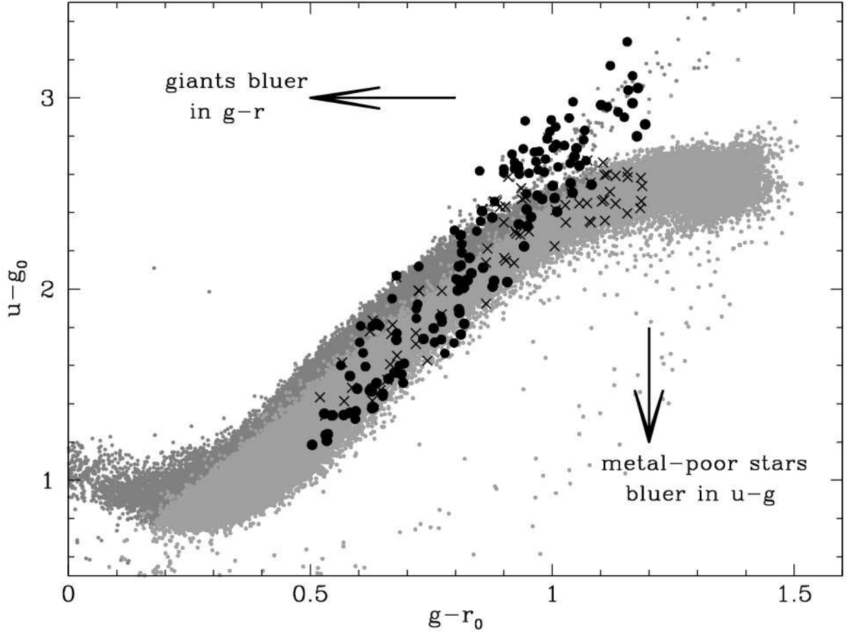
Fig. 10.— a demonstration of how the K giant locus crosses from the blue ( u - g ) side of the stellar locus at g - r = 0.6 over to the red side of the locus at g - r = 1.0 . M giants with TiO features appear at g - r > 1.3 and u - g > 3.0 . The small dot shows the photometric stellar locus in a SEGUE high latitude field (there are Sagittarius M giants present at the end of the locus). Stars with l -color greater than 0.07 are shown in light gray. Spectroscopically confirmed dwarfs are shown with large crosses, giants with large filled circles.
