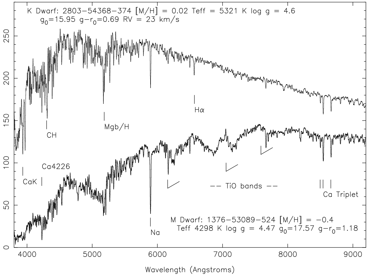
Fig. 12.— Top: a sample SEGUE K dwarf, note the strong Mg b/H and Na I. Lower: a sample SEGUE M dwarf, note the strong MgH, Na I and TiO molecular bands.
