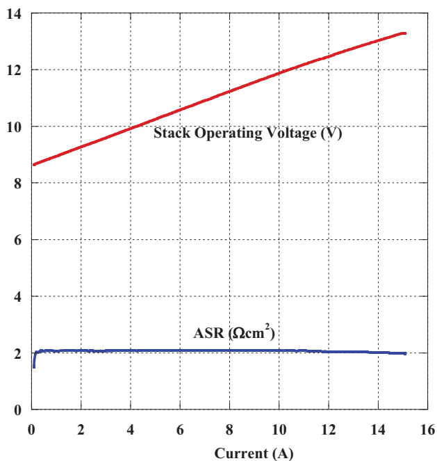
Figure 5. Initial polarization curve for stack.
