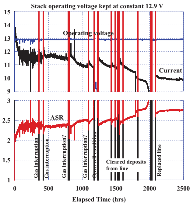
Figure 6. ASR, current, and voltage for the 2500 hour 10-cell stack test.
