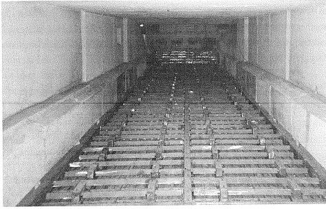
Grate clinker cooler photograph and reciprocating grate cooler diagram, both images taken from Bhatti, J. I., F. M. Miller and S. H. Kosmatka (eds.) 2004. Innovations in Portland Cement Manufacturing. Portland Cement Association.
