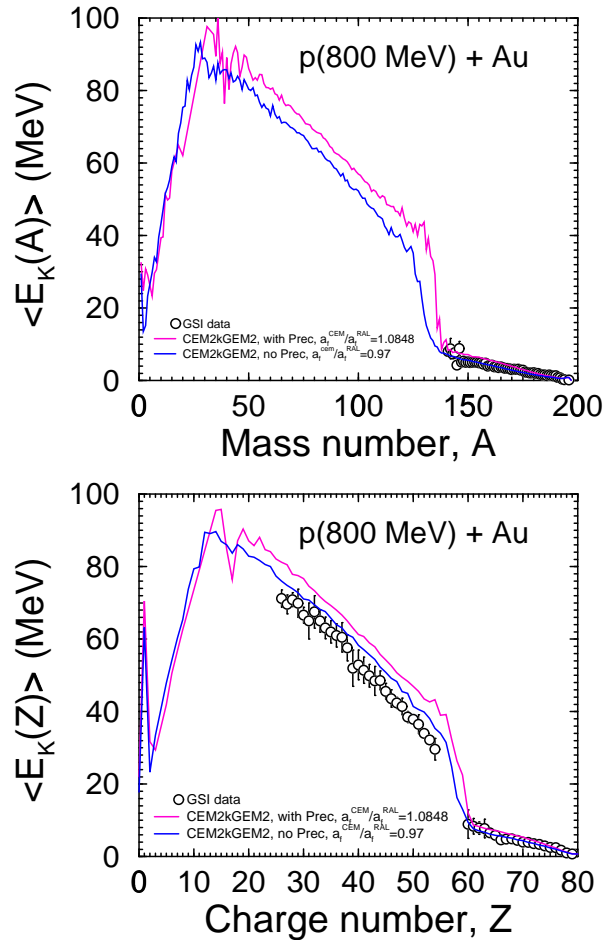
Figure 6. Comparison of the experimental 9 mass and charge distributions of the kinetic energy of the nuclides produced in the reaction p(800 \text{ MeV}) + \text{Au} (circles) with our CEM2k+GEM2 calculations: “with Prec” results are shown by red lines, “no Prec” results are shown by blue lines.
