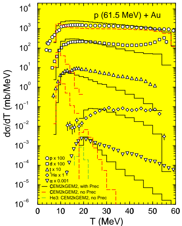
Figure 14. Angle-integrated energy spectra of p , d , t , {}^3\text{He} , and {}^4\text{He} from 61.5 MeV protons on {}^{197}\text{Au} . Calculations from the merged CEM2k+GEM2 code “with Prec” are shown by solid black histograms and “no Prec”, by dashed red (and green, for {}^3\text{He} ) histograms. Experimental data (symbols) are from Bertrand and Peelle 60 .
