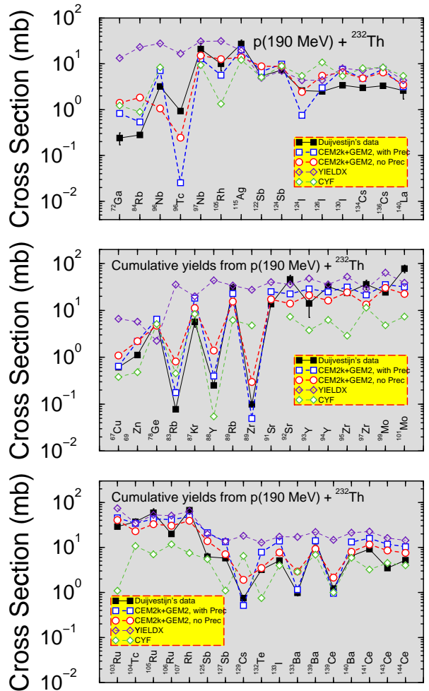
Figure 16. Detailed comparison between experimental 62 (black filled squares) and calculated cross sections of individual (upper plot) and cumulative (middle and bottom plots) reaction products. Our CEM2k+GEM2 “with Prec” results are shown by connected blue squares and the “no Prec” results are shown by connected red circles. For comparison, predictions by the phenomenological systematics YIELDX of Silberberg, Tsao, and Barghouty 23 are shown by connected indigo diamonds, and results calculated by Dr. W. B. Wilson with the phenomenological code CYF by Wahl 65 are shown with connected green diamonds. We thank Dr. Wilson for providing us with results of his calculations with the CYF code included in this figure.
