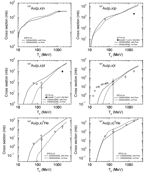
Figure 13. The same as Fig. 8 but for the production of n, p, d, t, {}^3\text{He} , and {}^4\text{He} . The complex particles are produced in CEM2k+GEM2 via evaporation and preequilibrium emission; n and p are also produced during the cascade stage.
