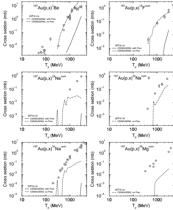
Figure 12. The same as Fig. 8 but for the production of {}^7\text{Be} , {}^{18}\text{F}^{cum} , {}^{24}\text{Ne}^{cum} , {}^{22}\text{Na}^{cum} , {}^{24}\text{Na}^{cum} , and {}^{28}\text{Mg}^{cum} . These fragments are produced in CEM2k+GEM2 only via evaporation.
