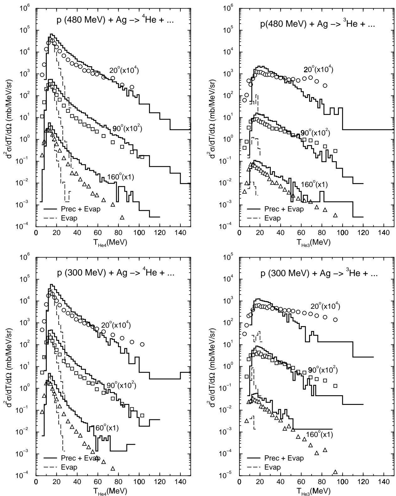
Figure 20. Double-differential spectra of {}^4\text{He} and {}^3\text{He} from 480 and 300 MeV protons on Ag. Calculations from the CEM2k2f code are shown by solid histograms and contribution from only the evaporation mode, by dashed histograms. Experimental data (symbols) are by Green and Korteling 81 .
