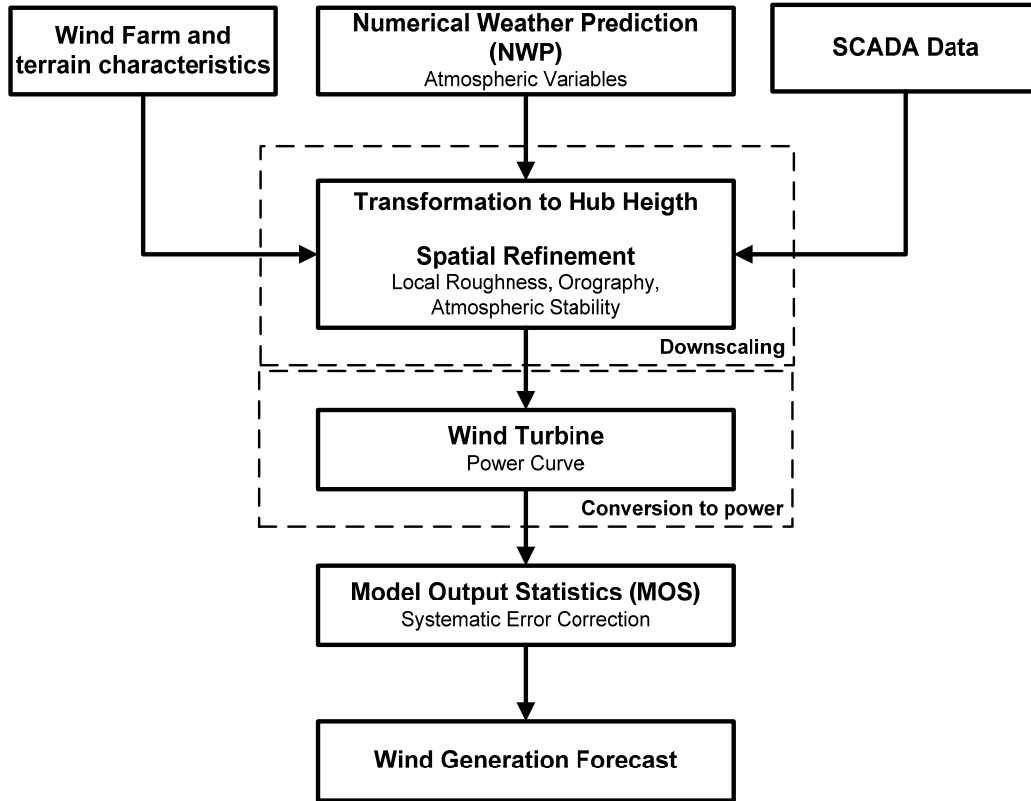
FIGURE 3-3 Main Steps of the Physical Approach
