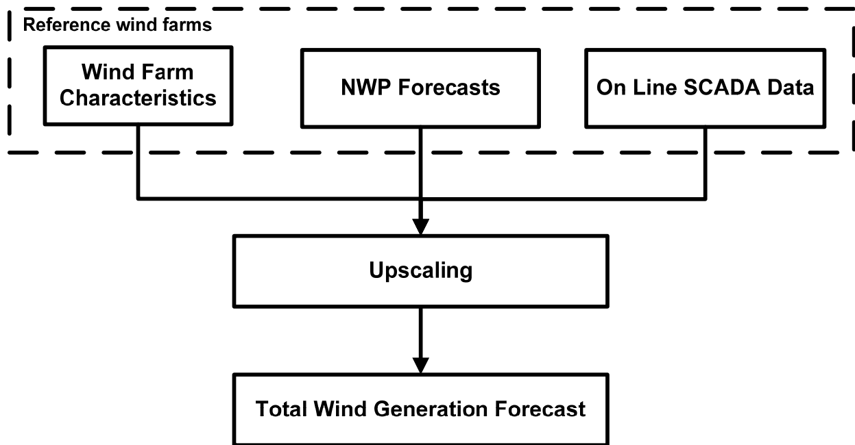
FIGURE 3-7 Direct Upscaling Method
