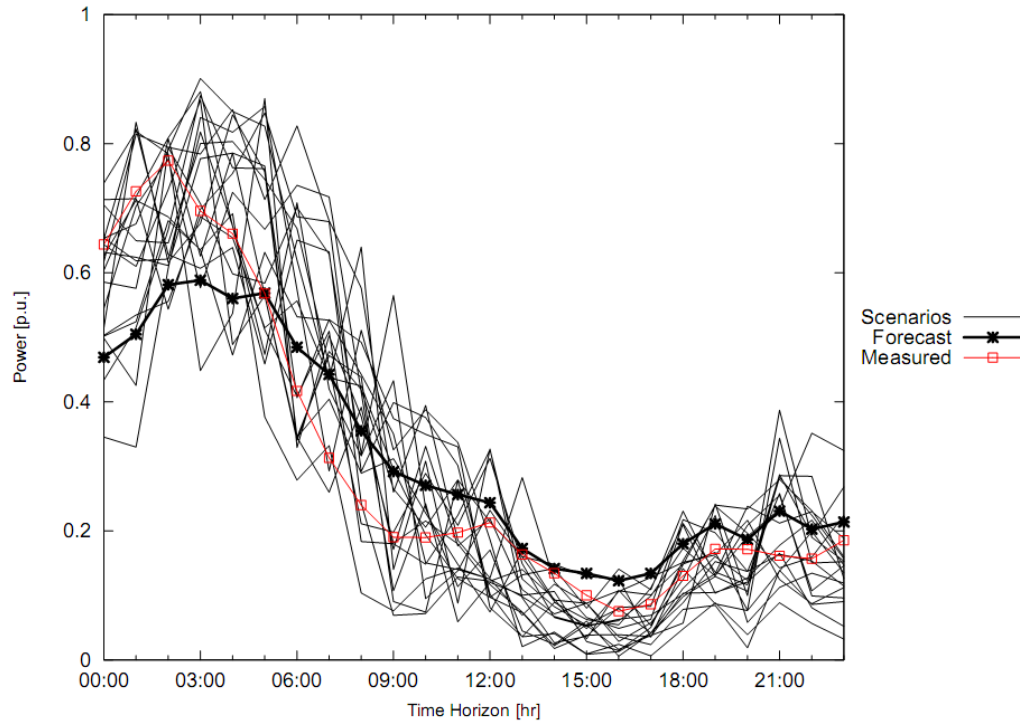
FIGURE 5-3 Scenarios of Wind Generation (20 scenarios)
