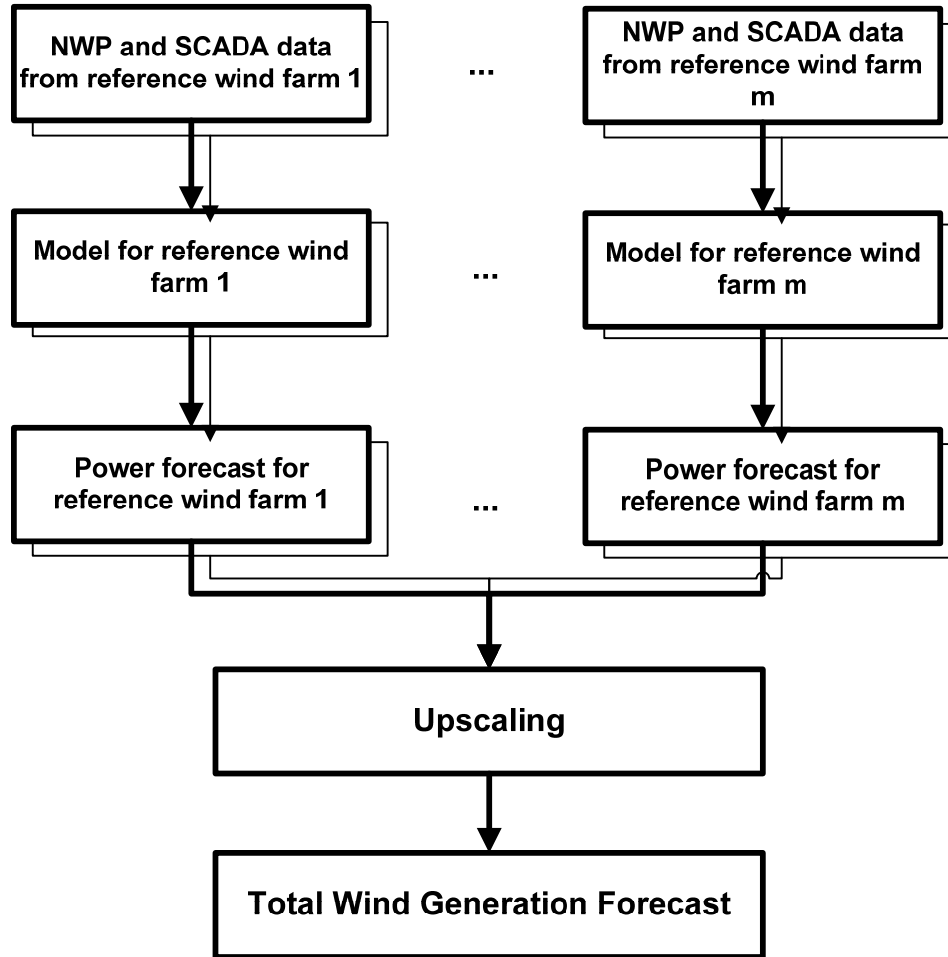
FIGURE 3-8 Cascaded Method for m Reference Wind Farms
