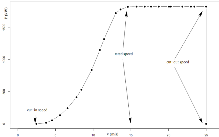
FIGURE 2-1 Wind Turbine Power Curve
