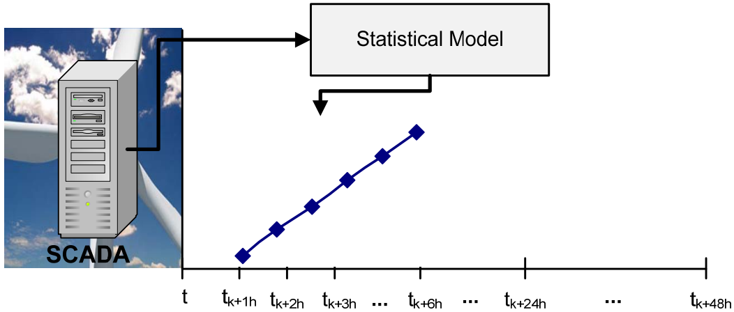
FIGURE 3-1 Very-Short-Term Forecasting Structure (adapted from [67])
