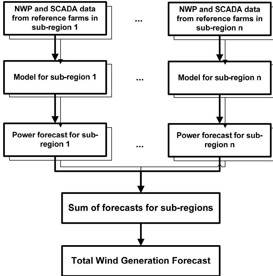
FIGURE 3-9 Cluster Method for n Clusters/Subregions
