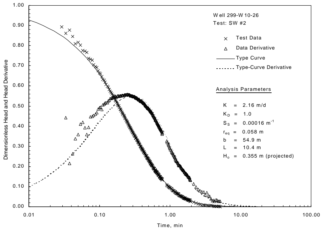
Figure 4.4. Selected Slug-Test Analysis Plots for Well 299-W10-26 (Bouwer and Rice method [top] and Type-Curve Method [Bottom])
