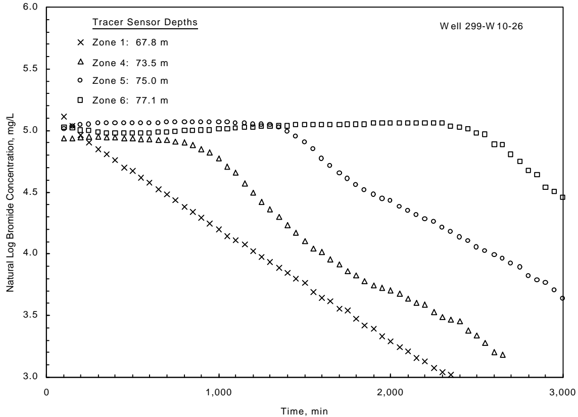
Figure 8.1. Tracer Concentration Versus Depth-Response Patterns Within Well 299-W10-26 During Tracer-Dilution Testing
