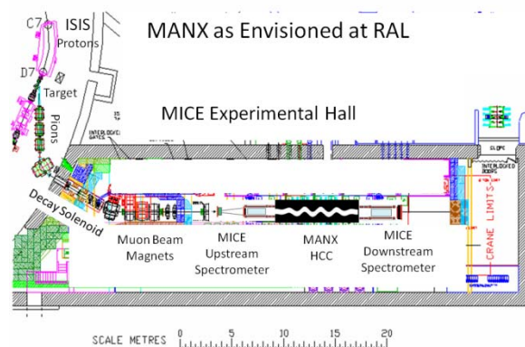
Figure 1: Layout of MANX in the MICE beam line at RAL. In addition to the MICE spectrometers there are MICE beam counters and particle identification detectors that will be reused for MANX.
