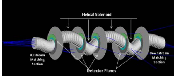
Figure 2: The helical cooling channel, with helical solenoid, matching sections and internal tracker units shown.
