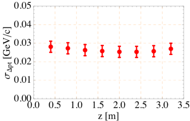
Figure 6: RMS of transverse momentum distribution in the HCC.
