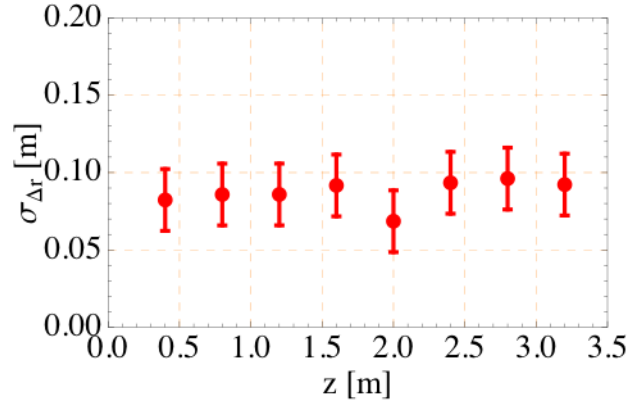
Figure 7: RMS of time spread in the HCC.
