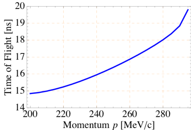
Figure 4: Time-of-flight versus momentum for a 3.2 m long HCC. This shows that the time difference per 10 MeV/c is approximately 500 psec.
