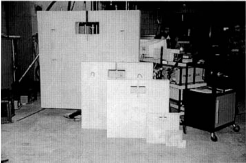
Figure 2 Concrete CT type specimens.
