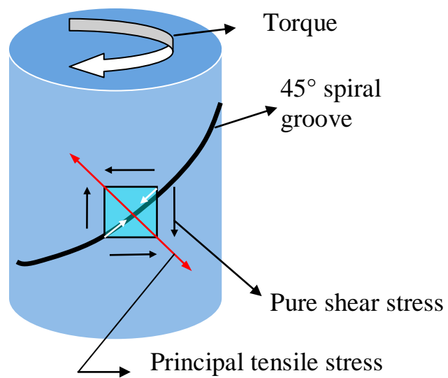
Figure 5 SNTT loading configuration.
