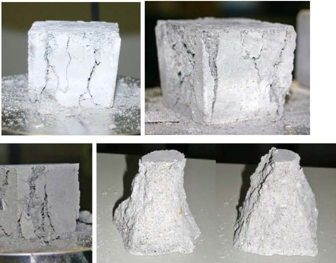
Figure 12 Compression fractured samples, w/o Teflon insert, r. h. s. shows typical core of fracture samples.
