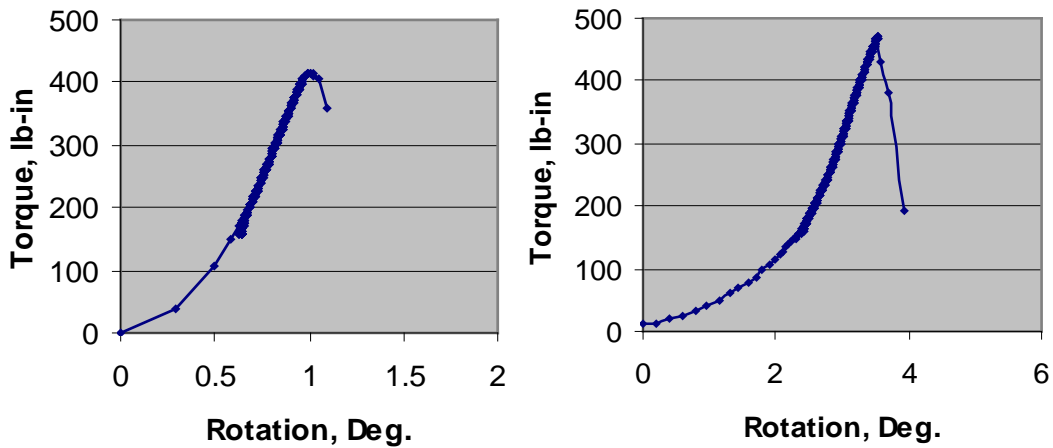
Figure 23 SNTT torsion test results, with notch depth (left) at 0.10-in, (right) at 0.075-in.
