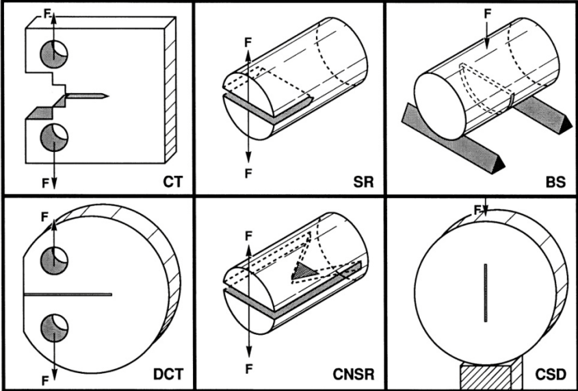
Figure 1 Brittle material fracture toughness test methods.
