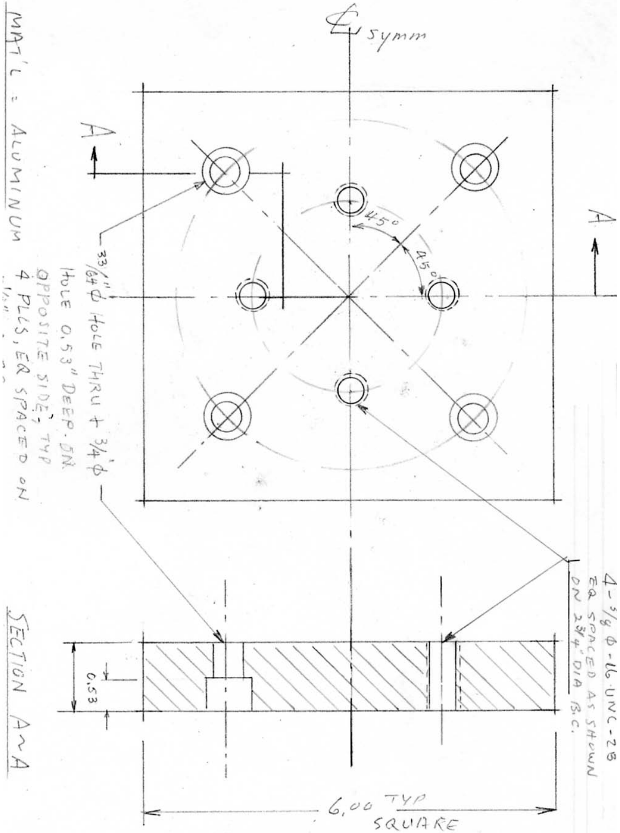
Figure 16 Adapter plate design for the Chuck type A.
