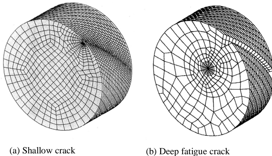
Figure 6 SNTT FEM Models: (a) for the brittle material configuration, (b) for the ductile metallic material configuration.
