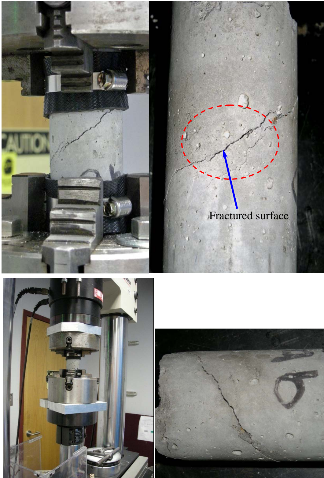
Figure 14 Chuck grip torsion test set-up. The fracture surface matches the principal tensile stress contour.
