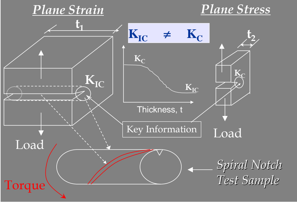
Figure 7 Specimen size effect and SNTT transformation
