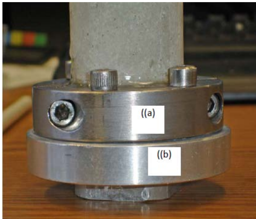
Figure 9 SNTT concrete grip fitting, (a) split-ring clamp, (b) square-end adapter base plate.
