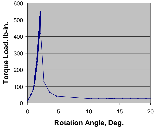
Figure 18 Pure torsion test results.
