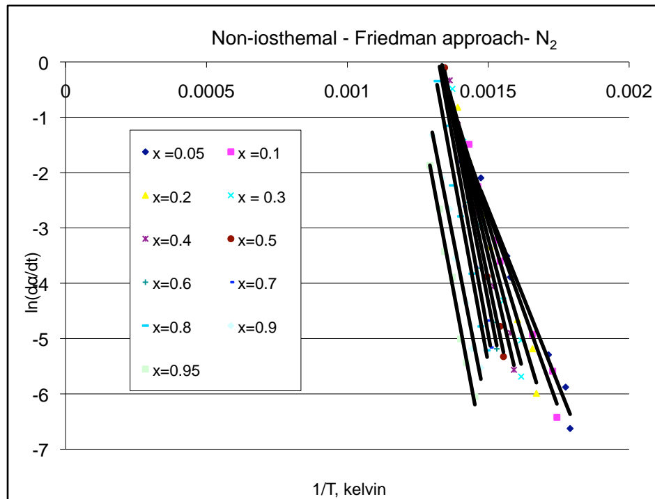
Figure - 22: An isoconversion approach (Friedman method) for the analysis of non-isothermal pyrolysis of oil shale.
