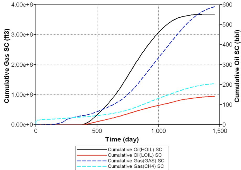
Figure 15. Cumulative oil and gas production.
