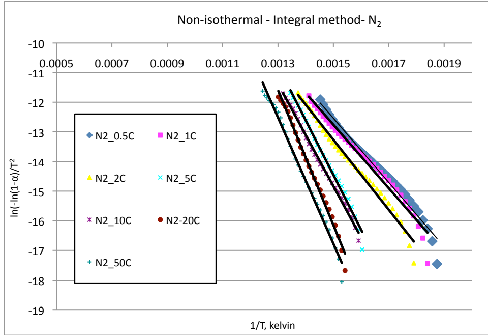
Figure - 19: Analysis of non-isothermal TGA pyrolysis data using the integral method.
