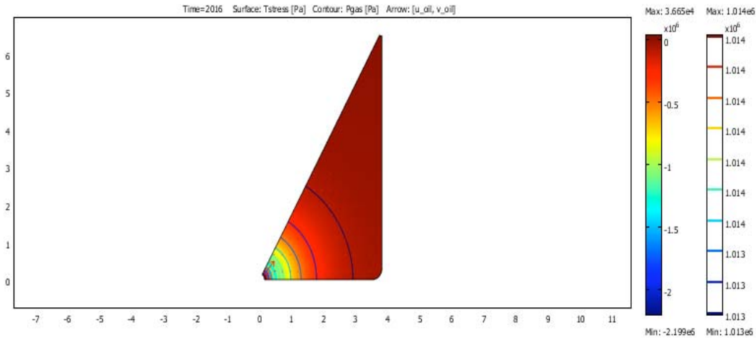
Figure 5. Thermal stress (color) and pressure (contours) on the deposit, both in units of Pa.
