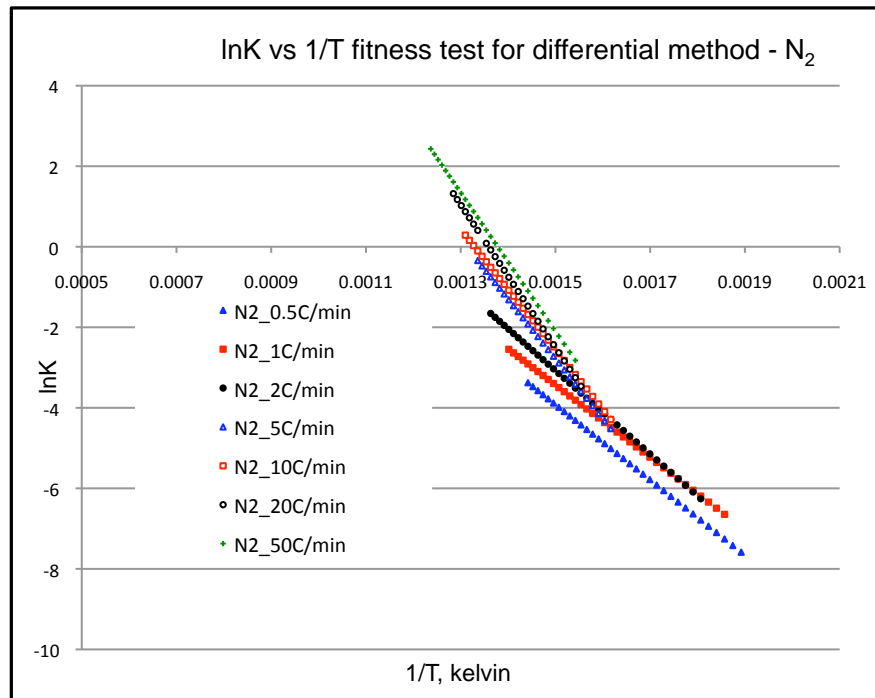
Figure - 29: Goodness of the fit using the differential method – pyrolysis.
