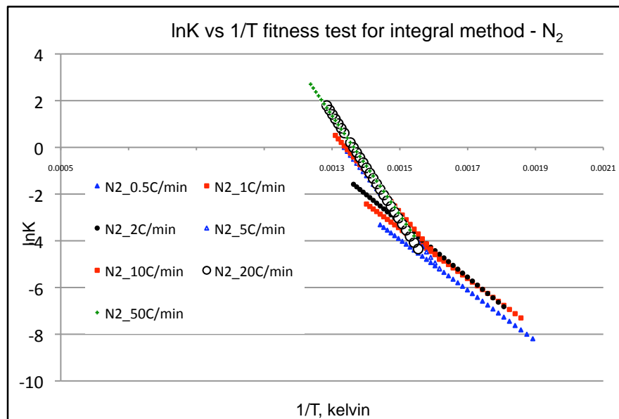
Figure - 30: Goodness of the fit using the integral method – pyrolysis.
