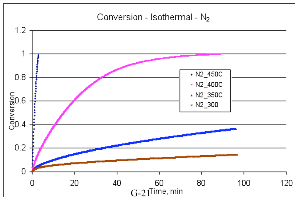
Figure - 8: Normalized conversion in isothermal TGA experiments for \text{N}_2 environment (pyrolysis).
