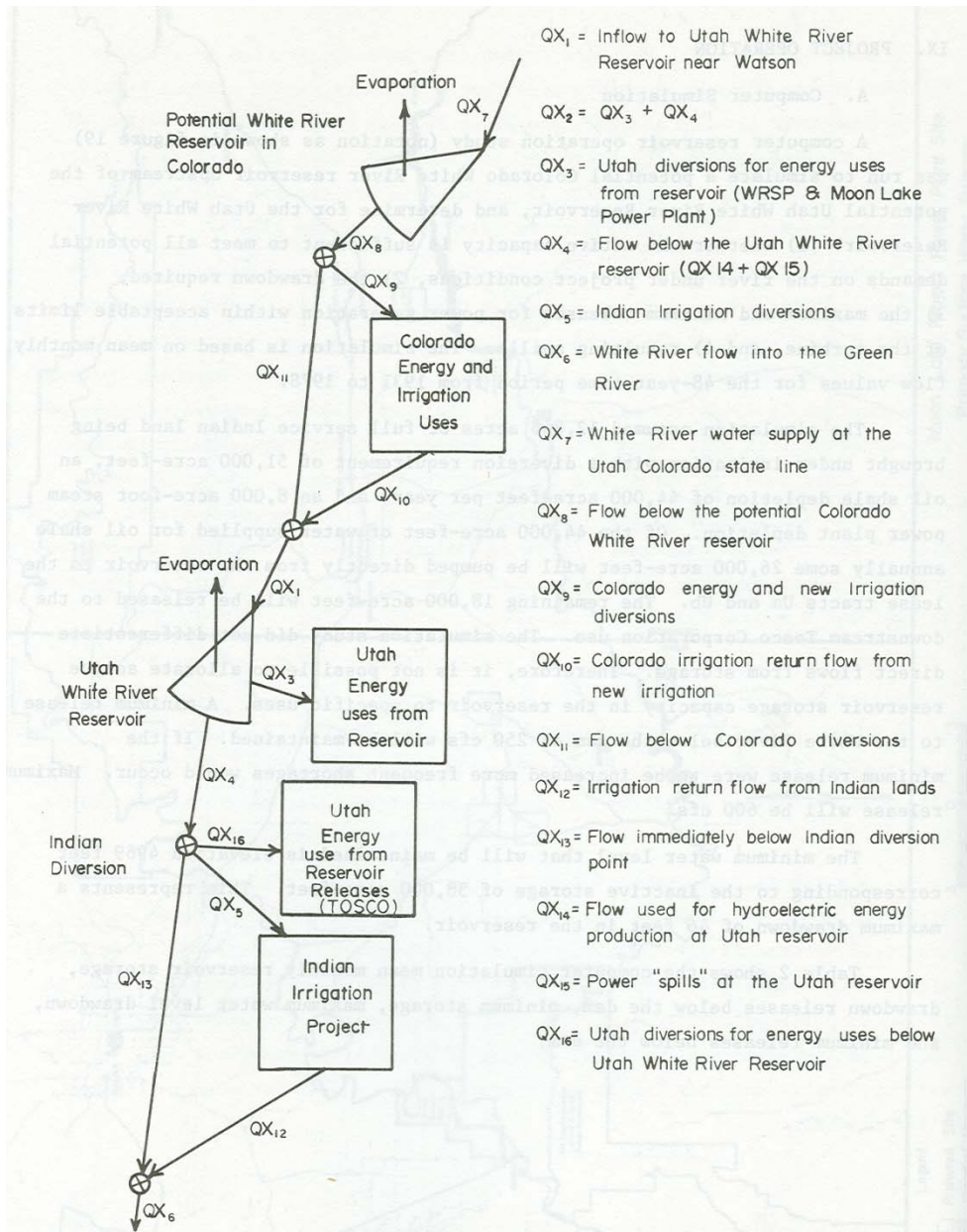
Figure 19. Diagram of White River water management modeling framework [32].
