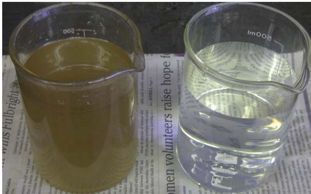
Figure 3. Visual results of ozonation in pressure cycles followed by sand filtration. Left: before treatment; Right: after treatment with 10 cycles of PC/O 3 + SF and 20 cycles of PC/O 3 + SF (gas flow rate of 5L/min).
