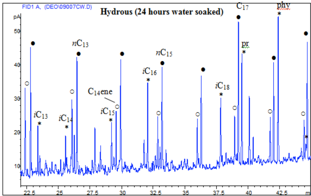
Figure - 38: Expanded chromatogram of a product from hydrous (24 hours water soaked) pyrolysis.
