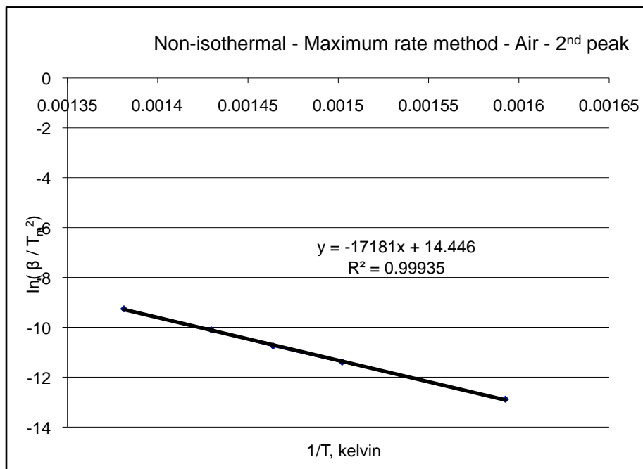
Figure - 26: Kinetic parameters using the maximum rate method for the combustion of oil shale (second peak): ( E_a = 142.842834 kJ/mol and A = 3.23E+10\text{min}^{-1} ).
