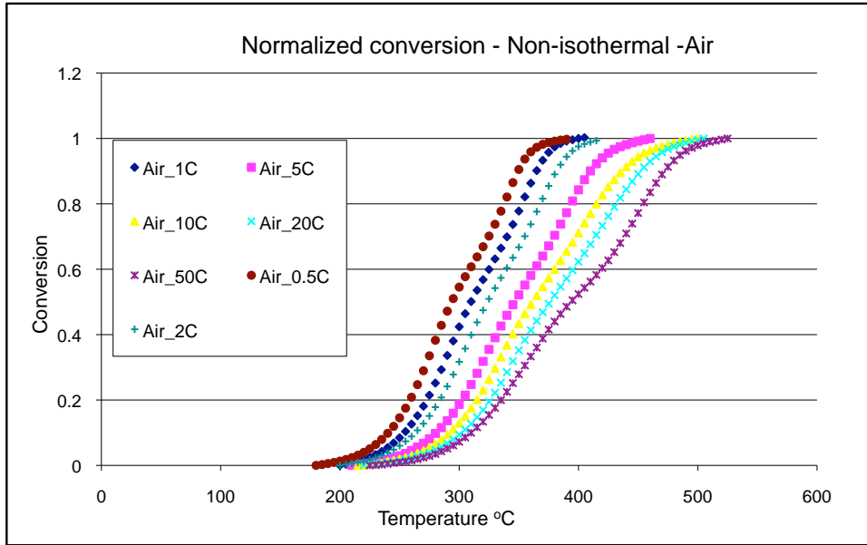
Figure - 15: Normalized conversion for non-isothermal TGA combustion data.
