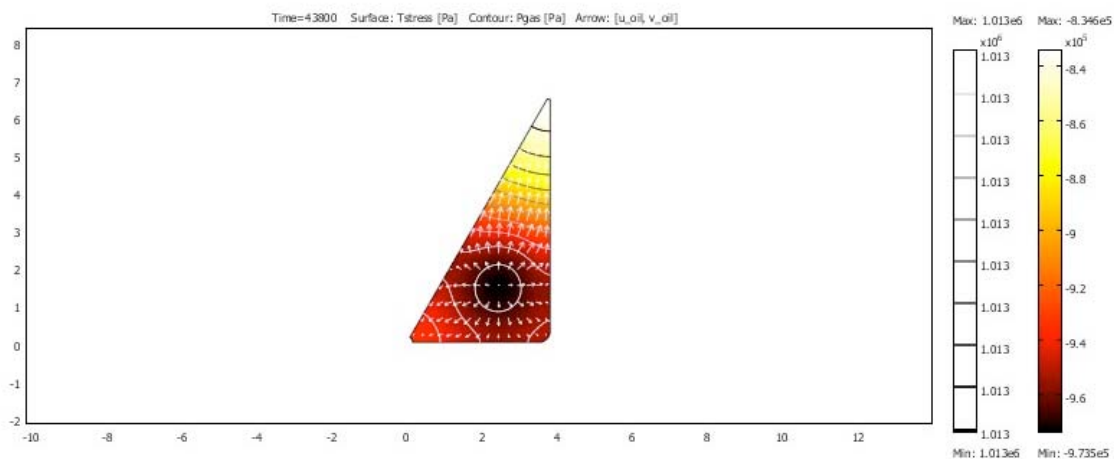
Figure 10. Thermal stress (color) and pressure (contours) on the deposit, both in units of Pa, at the end of a 5-year heating cycle with heating by the application of 628 MHz RF with 2,200 \text{ A/m}^2 external current to the deposit.
