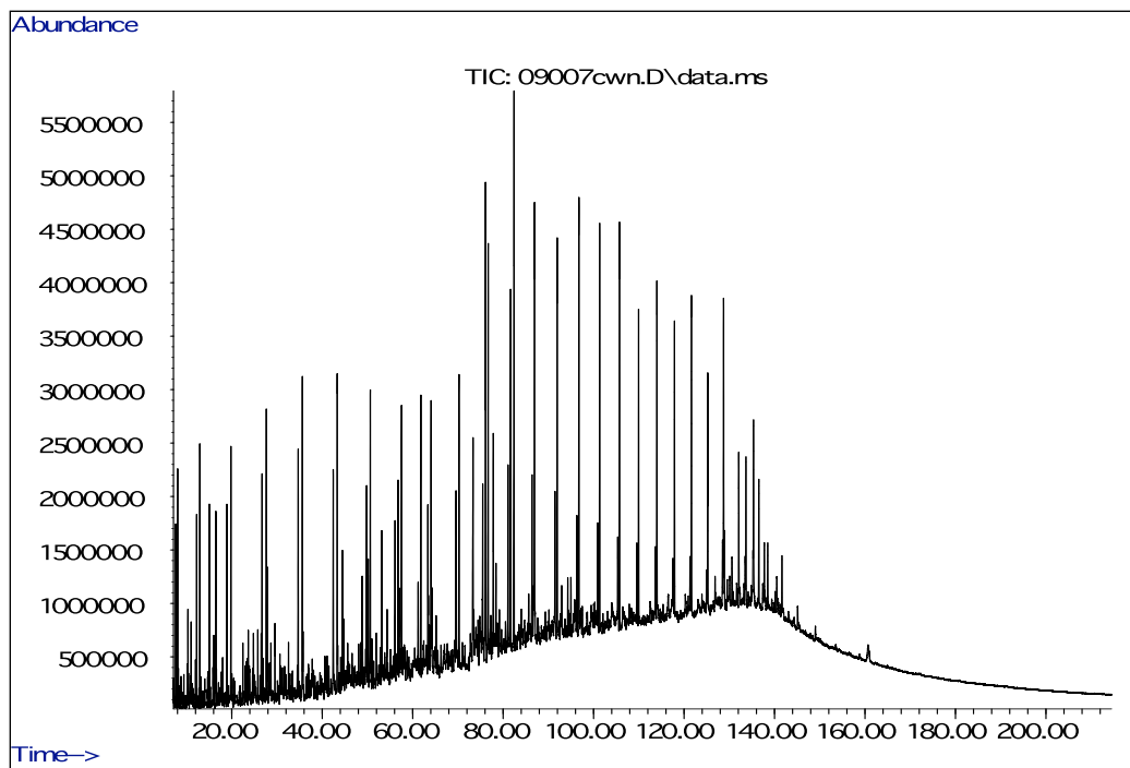
Figure – 40: GC-MS chromatogram (TIC) of a product from hydrous pyrolysis (24 hours water soaked).
