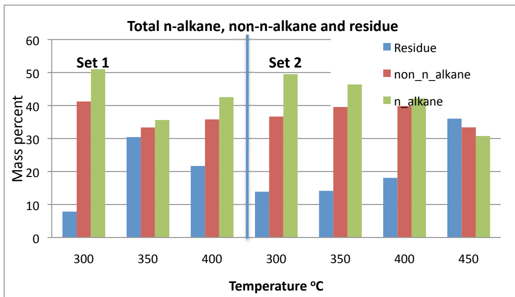
Figure - 37: Percents of n-alkane, non-n-alkane and residue in shale oil samples produced at different temperatures.
