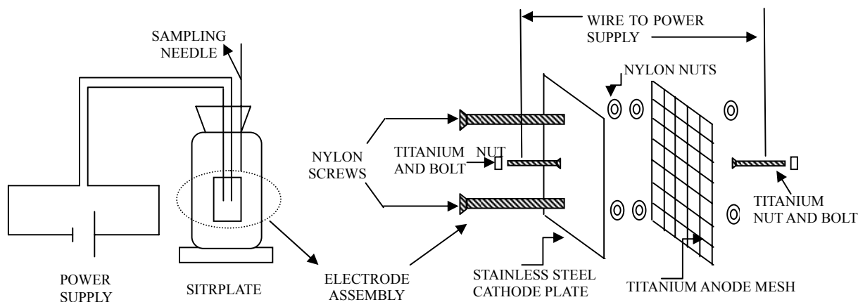
Figure 1: Schematic of the laboratory electrolytic batch reactor and the electrode assembly.
