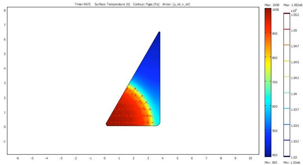
Figure 8. Temperature, pressure and velocity profile at the end of a 403 d (9,672 hr) heating cycle with heating by the application of a 1,000K heating well temperature and 1,000 volts DC at the heating well.
