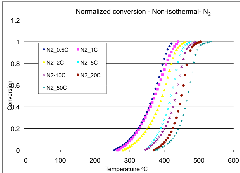
Figure - 14: Normalized conversion for non-isothermal TGA pyrolysis data.
