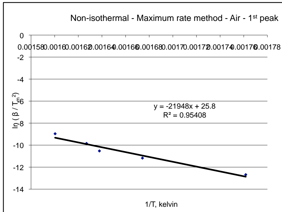
Figure - 25: Kinetic parameters using the maximum rate method for the combustion of oil shale (first peak): ( E_a = 182.47567 kJ/mol and A = 3.517E+15 min -1 ).
