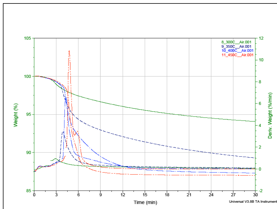
Figure -6: Isothermal TGA curves in air environment (combustion).
