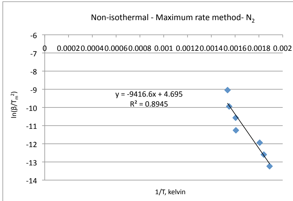
Figure - 24: Kinetic parameters using the maximum rate method for the pyrolysis of oil shale: ( E_a = 78.2846 kJ/mol and A = 1.03E+06 min -1 ).
