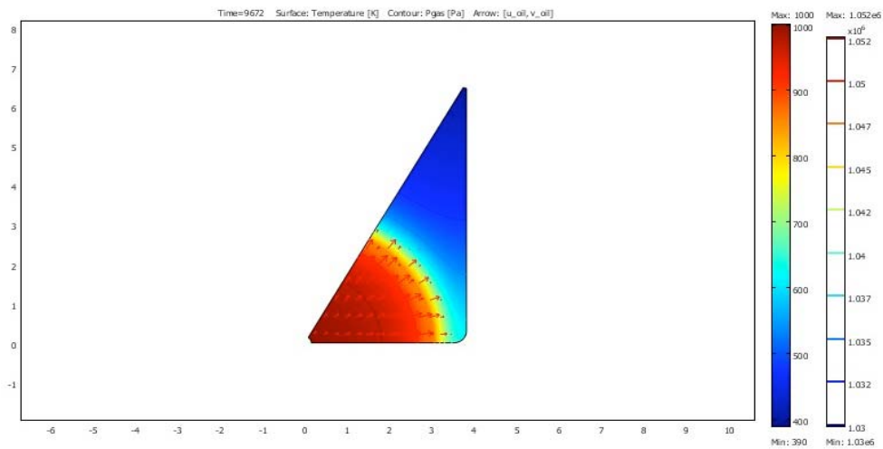
Figure 6. Temperature, pressure and velocity profiles at the end of a 403 d (9672 hr) heating cycle with heating by the application of a 1000K heating well temperature.
