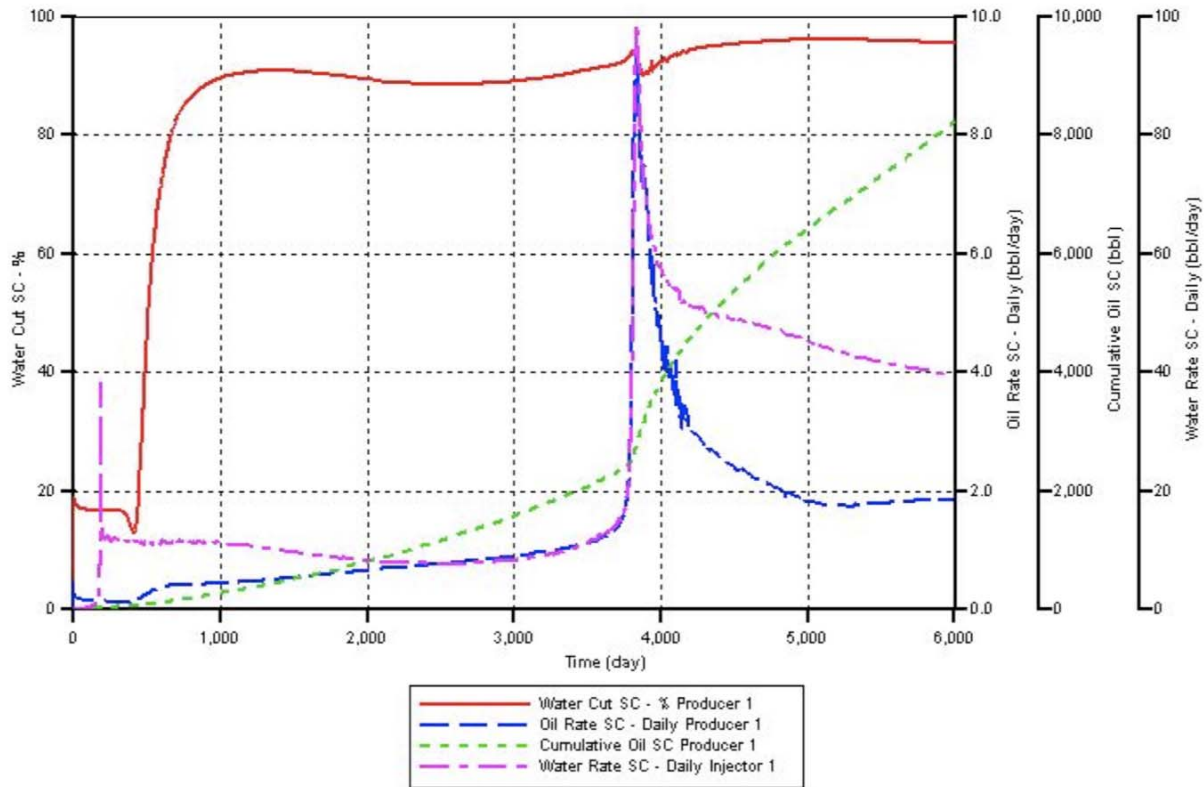
Figure 13: Oil production rates, water cut etc. for the vertical well system.
