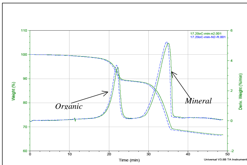
Figure - 1: Thermogravimetric analysis (TGA) of Green River oil shale. This analysis was performed to ensure reproducibility.
