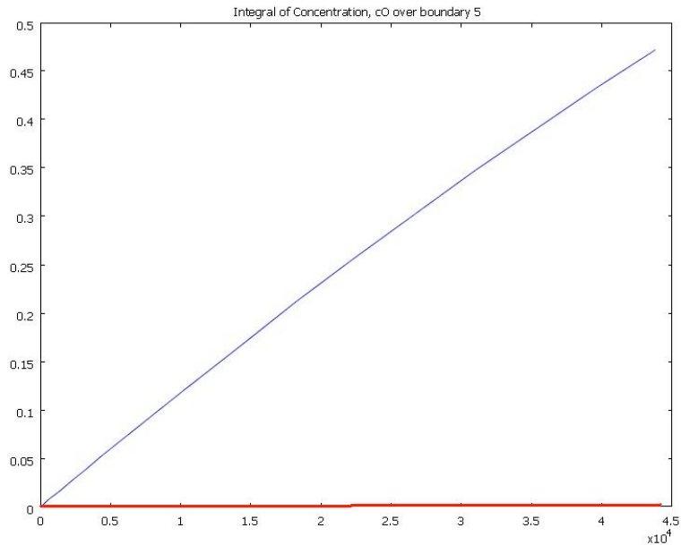
Figure 4. Oil concentration (weight %) at the producer well as a function of time (hrs) covering a period of 5 yrs (43,800 h). Red line – without pusher fluid or with constant heating well temperature boundary condition, Blue line – with pusher fluid.
