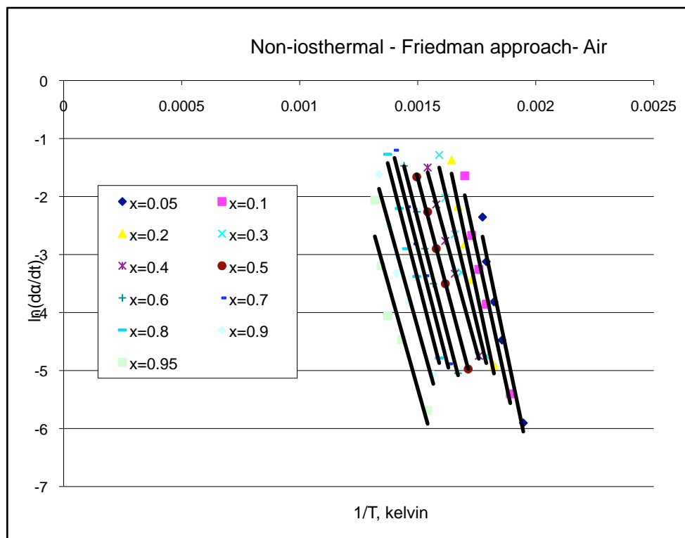
Figure - 23: An isoconversion approach (Friedman method) for the analysis of non-isothermal combustion of oil shale.
