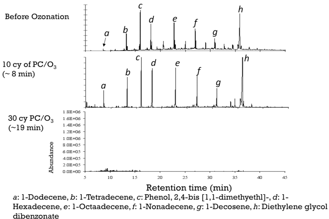
Figure 5. GC/MS Analyses - Products with increasing number of pressure cycles.
