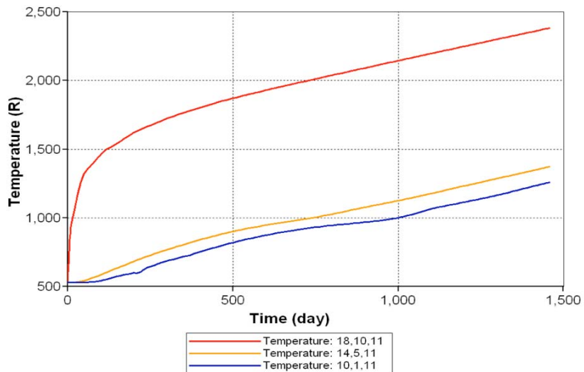
Figure 18. Temperature history comparison for three distances from heaters.
