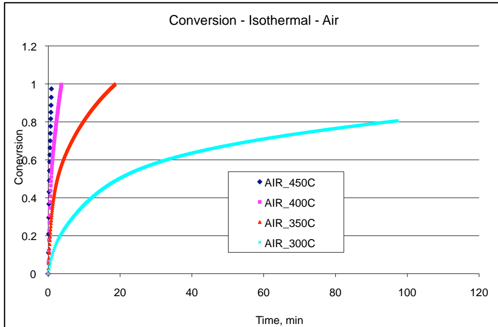
Figure - 9: Normalized conversion in isothermal TGA experiments for air environment (combustion).
