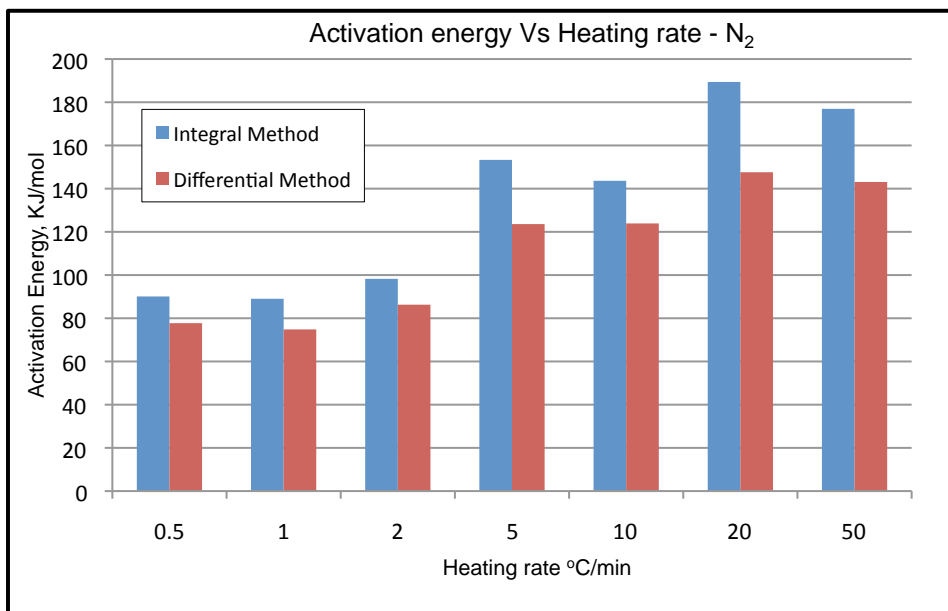
Figure - 27: Activation energies for the pyrolysis of oil shale using conventional methods.
