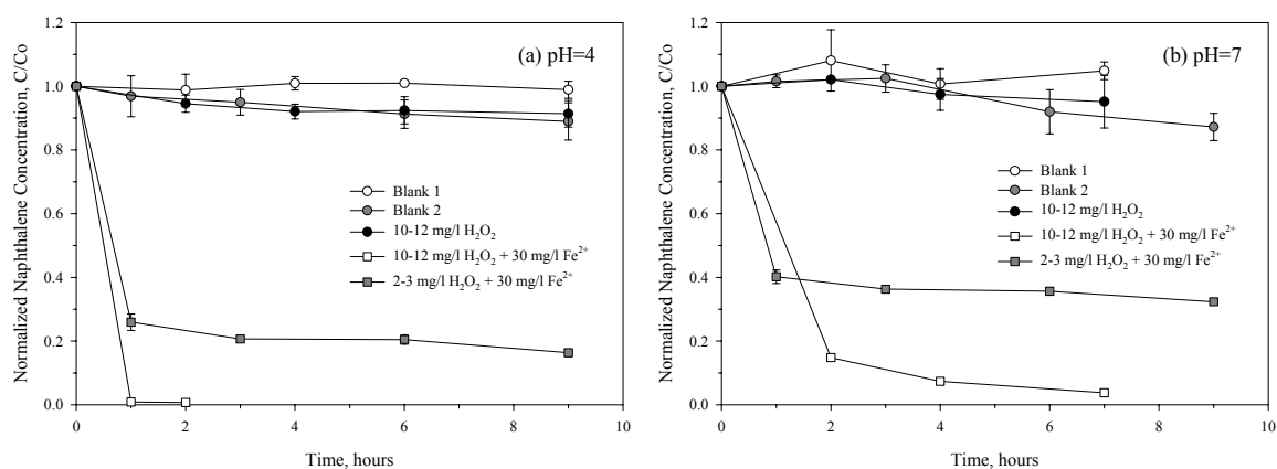
Figure 3: Naphthalene degradation using hydrogen peroxide and Fenton's reagent at (a) pH 4 and (b) pH 7.
