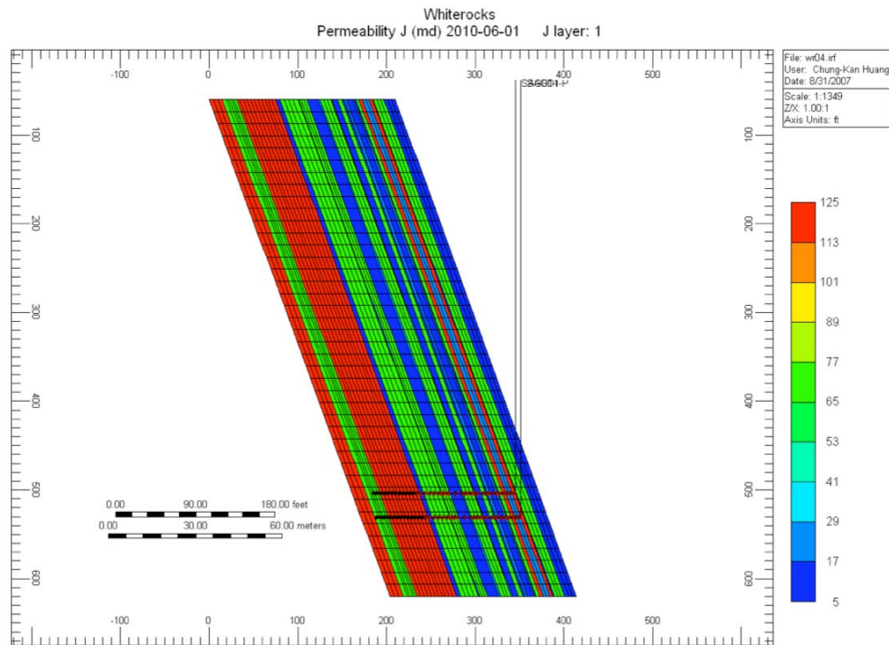
Figure 5: Model of the Whiterocks reservoir constructed in STARS.
