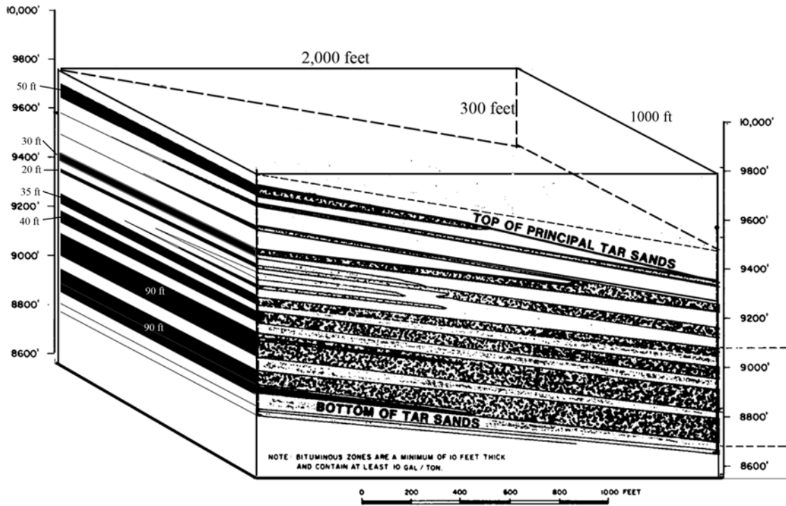
Figure 9: A geologic model of the Sunnyside deposit used in the simulations (from [20]).
