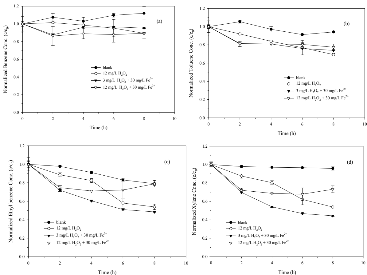
Figure 4: BTEX degradation using hydrogen peroxide and Fenton reagent at pH 7: (a) benzene, (b) toluene, (c) ethyl benzene and (d) xylene.
