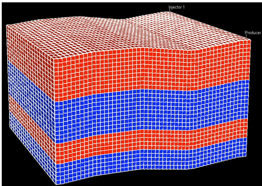
Figure 10: A small section of the Sunnyside geologic model used in the reservoir model. The model is 200 feet by 200 feet by 120 feet thick and has alternating rich and lean layers.
