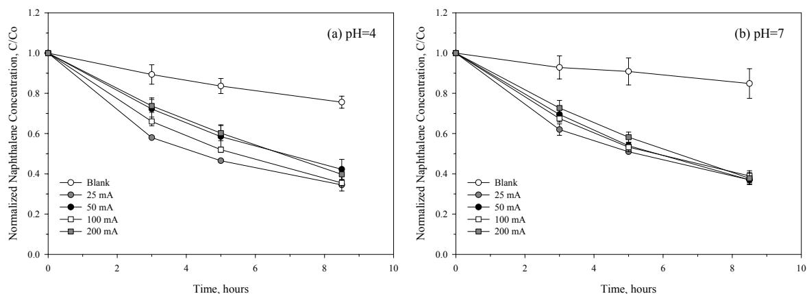
Figure 2: Electrolytic naphthalene degradation under different currents: (a) pH 4; (b) pH 7.
