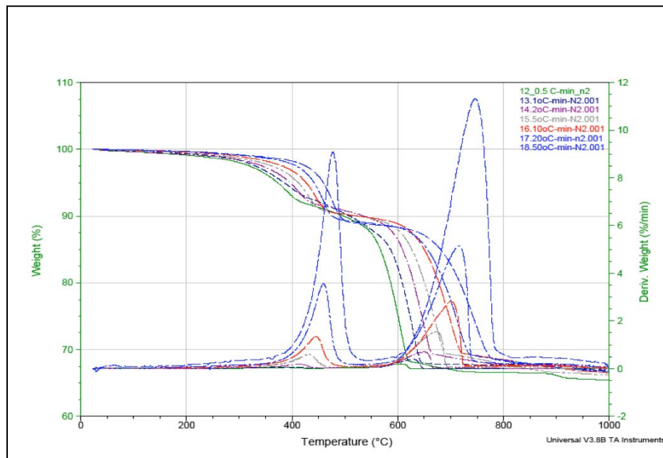
Figure - 5: Non-isothermal TGA pyrolysis curves. Rates go from 0.5°C/min to 50°C/min.
