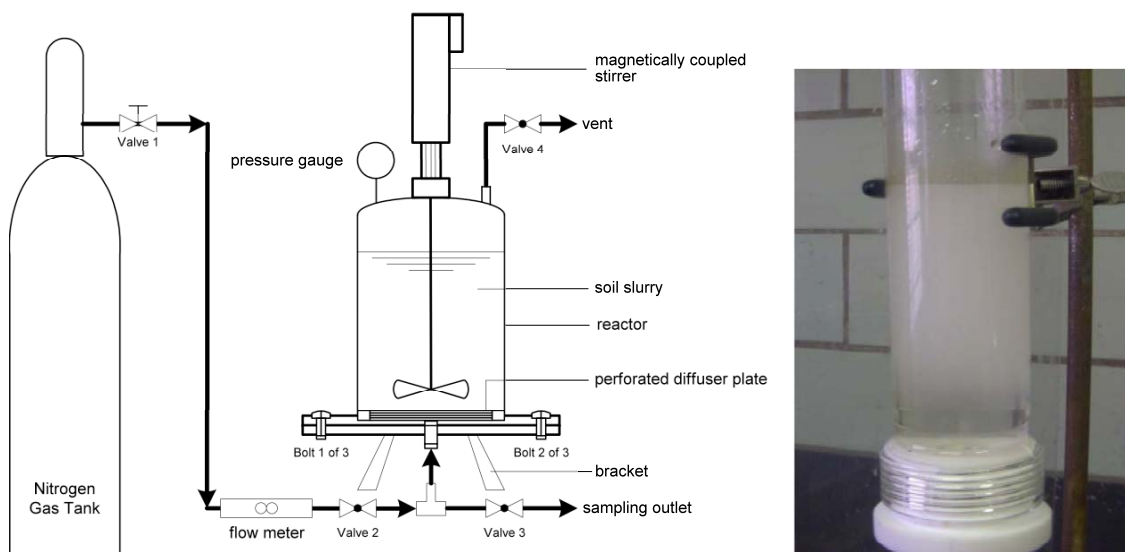
Figure 1. Reactor for pressure cycles (microbubbles shown in column).
