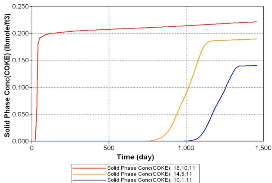
Figure 21. Coke concentration comparison for three distances from heaters.
