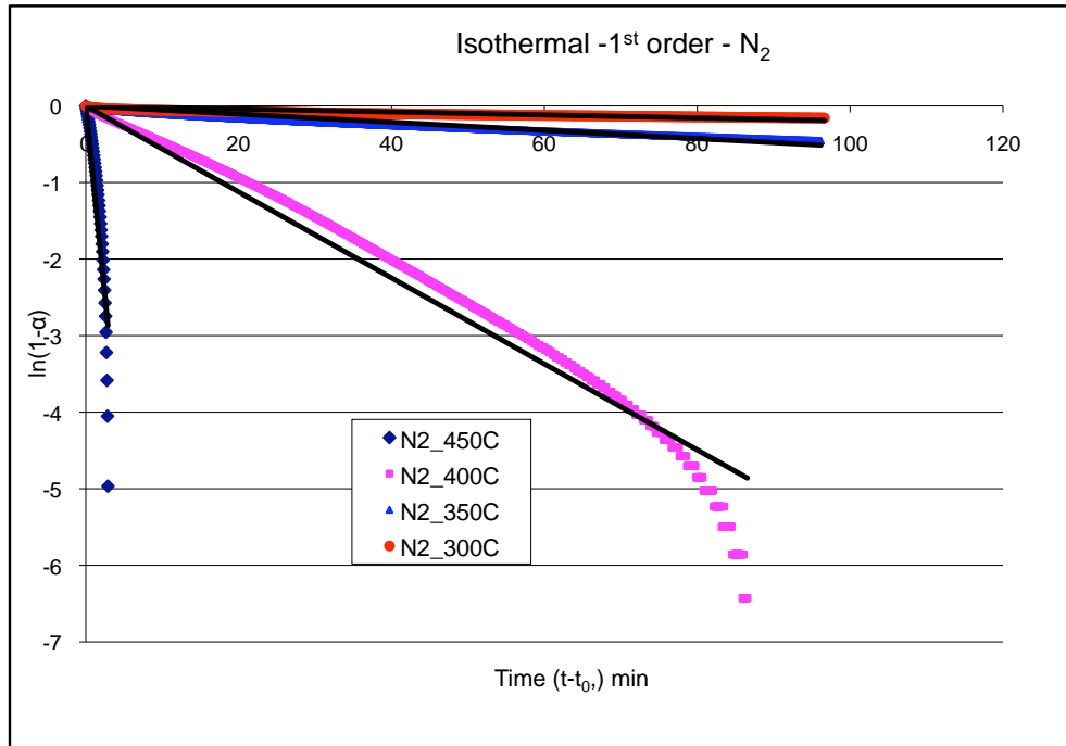
Figure - 10: Analysis of kinetic data using the integral method for 1 st order isothermal TGA pyrolysis experiments.
