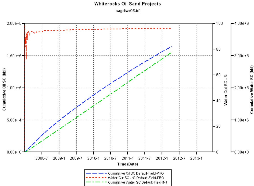
Figure 7: Oil production in Whiterocks SAGD simulations.
