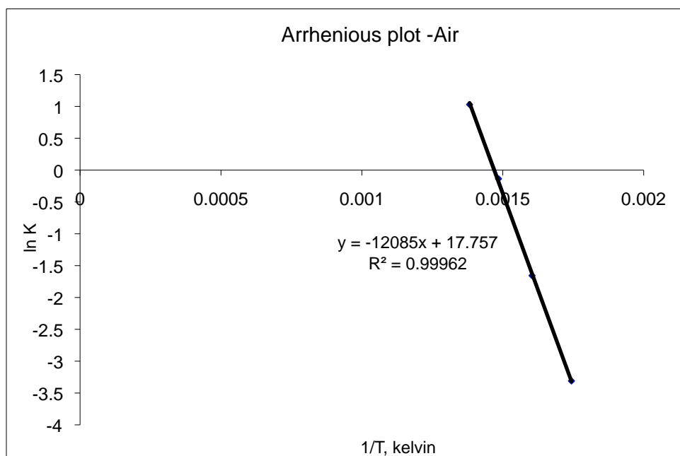
Figure - 13: Arrhenius plot for 1 st order isothermal TGA combustion experiments: ( E_a = 100.47 kJ/mol and A = 5.1E+07 min -1 ).
