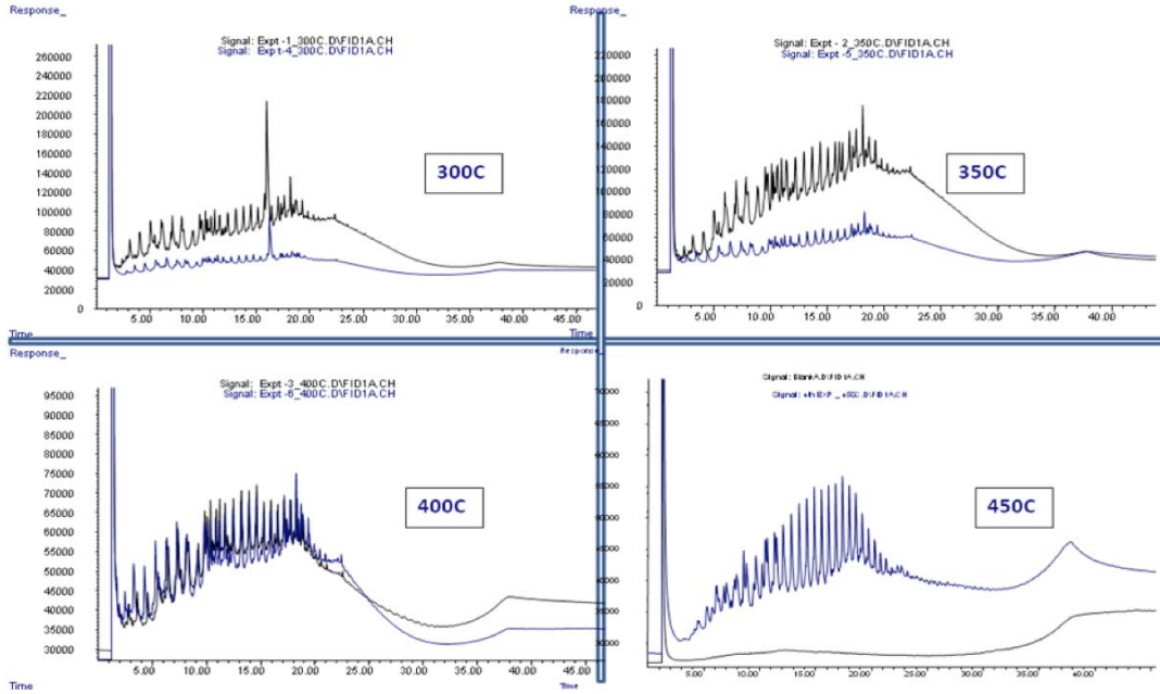
Figure – 32: Chromatographs for produced oil from pyrolysis of core samples at different temperatures.
