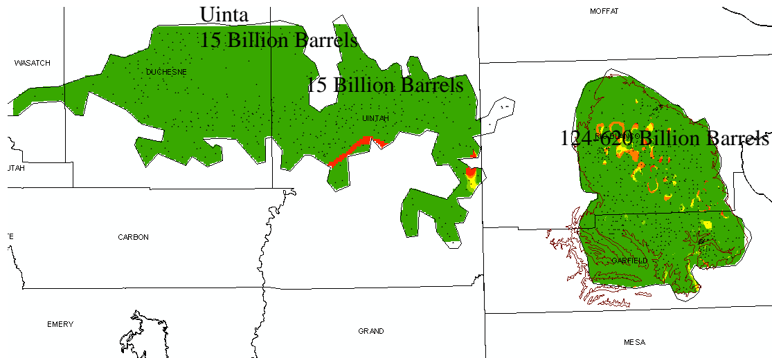
Figure 14. The estimated crude oil yield within the oil-shale Isopach of Uinta and Mahogany Areas (billion barrels) and the distribution of point features within both areas.
