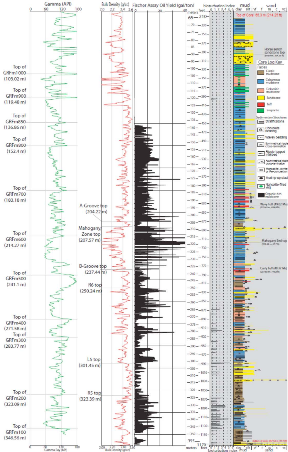
Figure 4. Geophysical, chemical, ichnological, and lithological logs for well P4 (see Figure 2 for location). Prominent marker beds, rich (R) and lean (L) oil-shale zones, and genetic stratigraphic horizons (GRFm#) are labeled.
