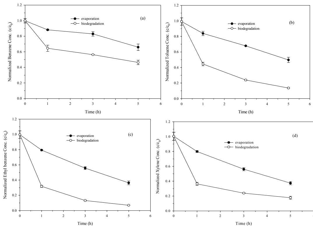
Figure 8: Biodegradation of BTEX by bacteria enriched by BTEX only: (a) benzene; (b) toluene; (c) ethyl benzene; (d) xylene.
