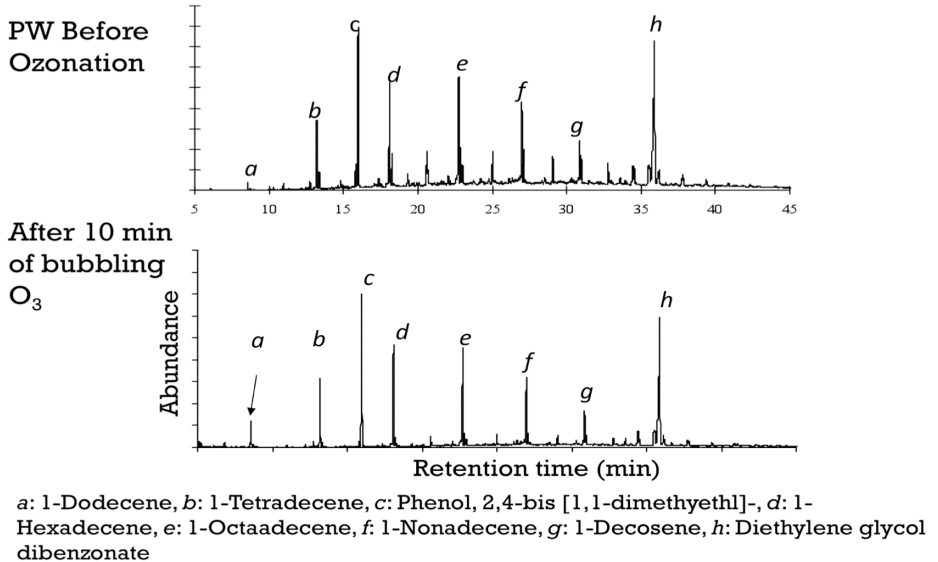
Figure 4a. GC/MS Analyses - Hexane-extractable hydrocarbons in produced water before and after 10 minutes of regular ozonation.
