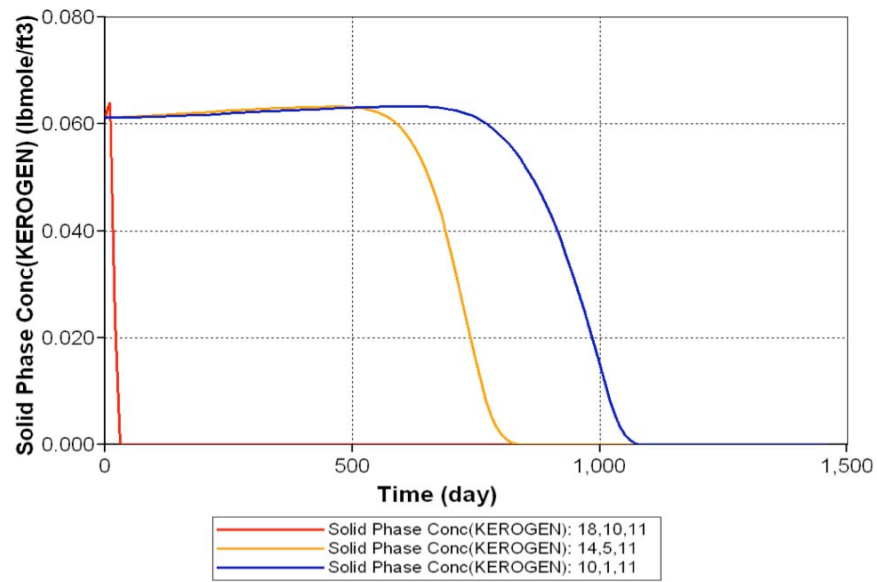
Figure 19. Kerogen concentration comparison for three distances from heaters.
