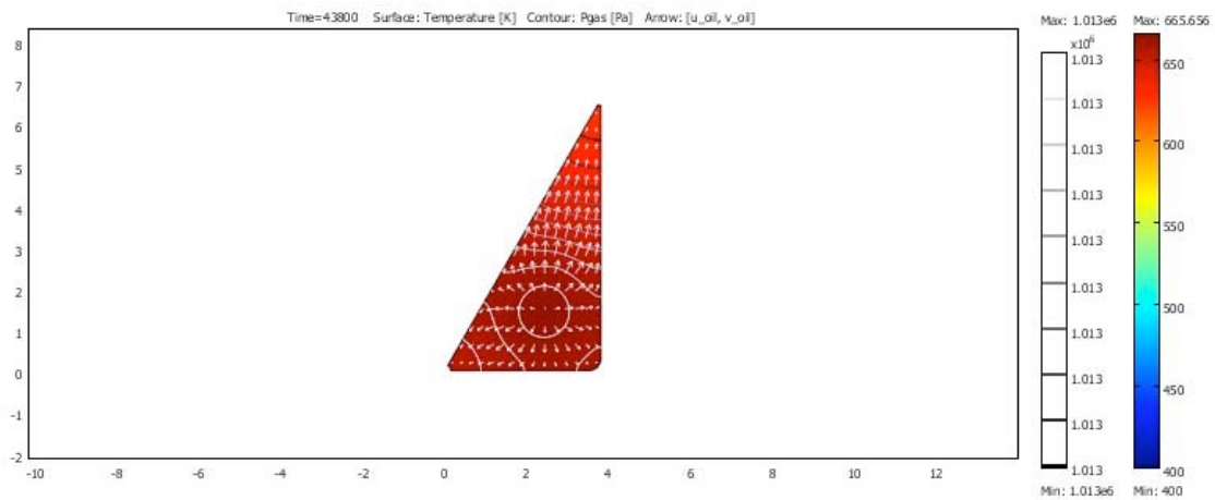
Figure 9. Temperature, pressure and velocity profiles at the end of a 5-year heating cycle with heating by the application of 628 MHz RF with 2,200 \text{ A/m}^2 external current to the deposit.
