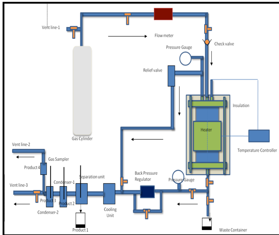
Figure – 2: Schematic diagram of the pyrolysis experimental setup for core samples.
