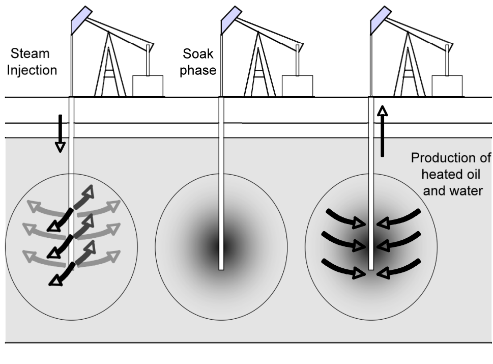
Figure 2: Schematic of the cyclic steam stimulation process showing the injection phase, the soak period and production from a single well (from [6]).
