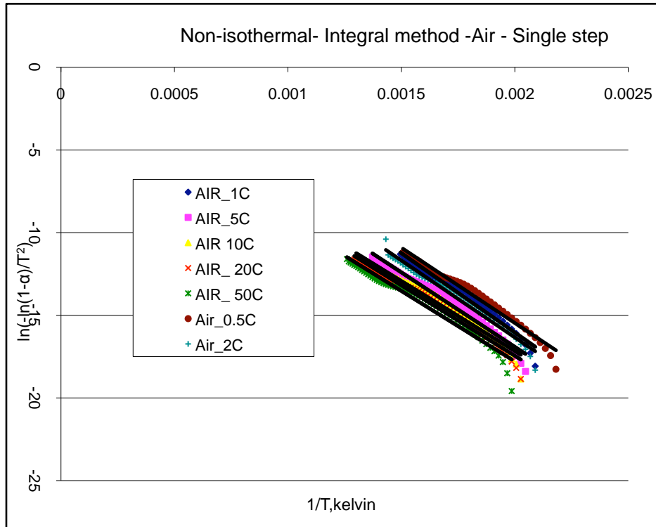
Figure - 20: Analysis of non-isothermal TGA combustion data using the integral method with a single-step mechanism.
