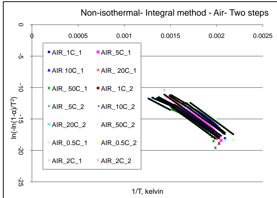
Figure - 21: Analysis of non-isothermal TGA combustion data using the integral method with a two-step mechanism.
