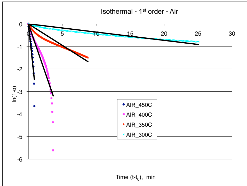
Figure - 11: Analysis of kinetic data using the integral method for 1 st order isothermal TGA combustion experiments.
