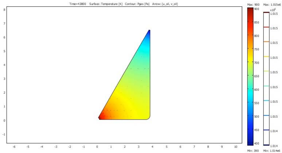
Figure 3. Temperature, pressure and velocity profiles at the end of a 5-year heating cycle with heating due to thermal conduction.
