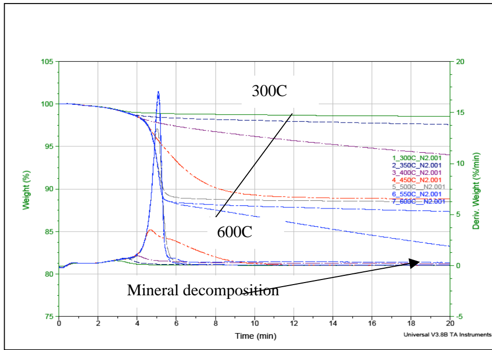
Figure -4: Isothermal TGA curves in the N 2 environment (pyrolysis). Weight loss increases and the maximum rate shifts to higher temperatures as temperatures increase.
