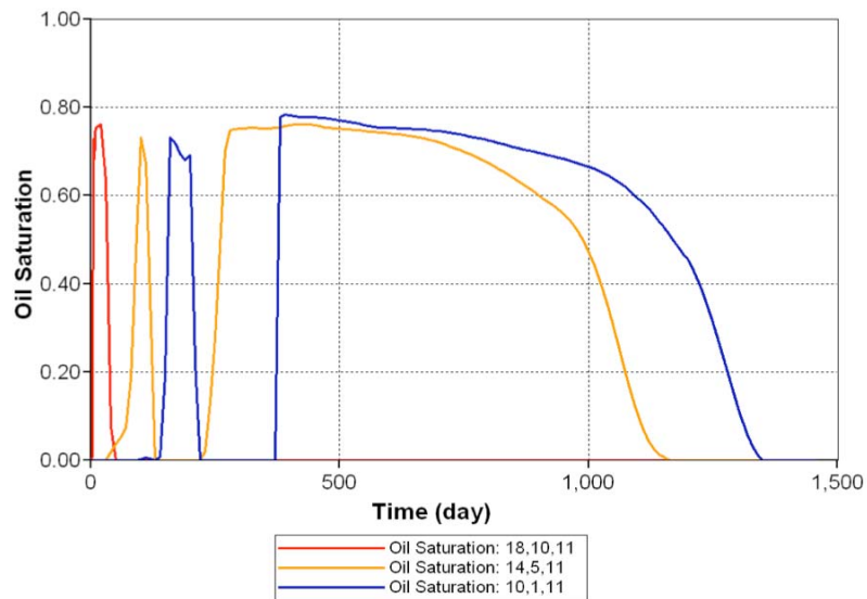
Figure 20. Oil saturation comparison for three distances from heaters.
