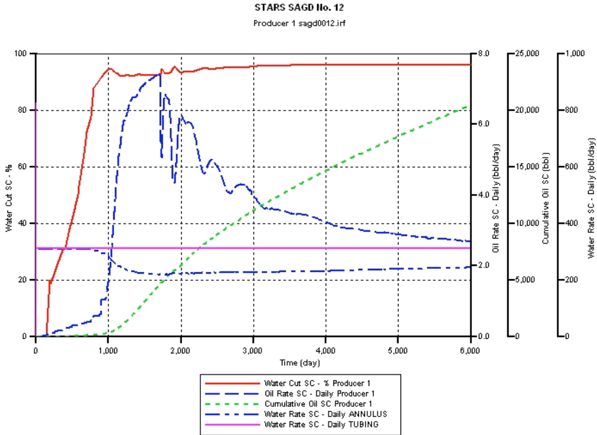
Figure 12: Production rates, cumulative production, etc. for SAGD production from Sunnyside.
