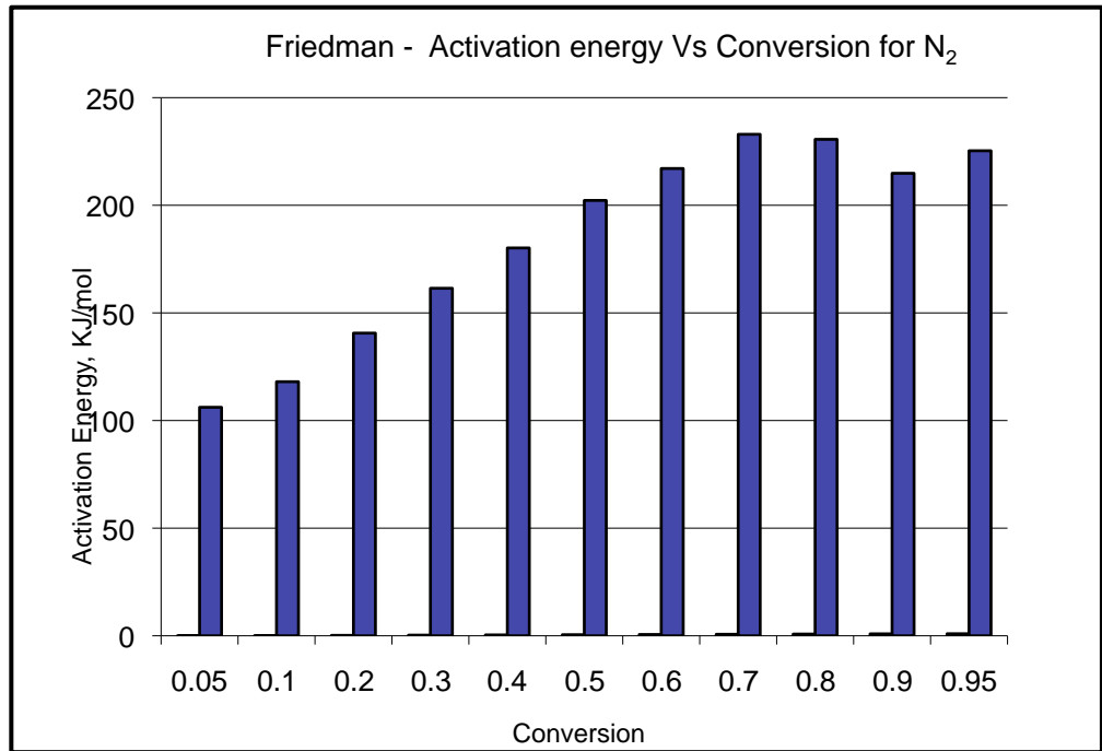
Figure - 28: Activation energy versus conversion for the pyrolysis of oil shale by the Friedman approach.
