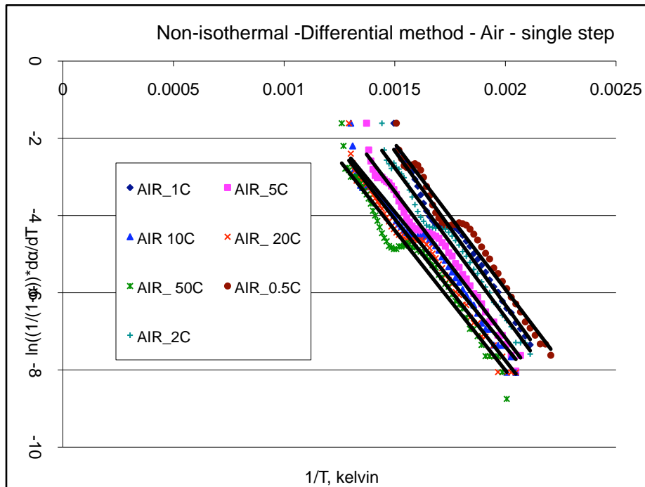
Figure - 17: Analysis of non-isothermal TGA combustion data (single-step) using the differential method.
