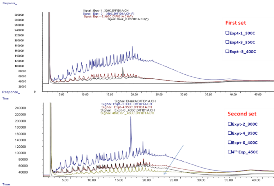
Figure – 33: Comparison of the chromatographs for produced oil from pyrolysis of core samples at different temperatures (shift towards lighter components at higher temperature). The '4 th Exp' in the legend stands for the experiment conducted with the tube reactor (Number 9 in Table 5).
