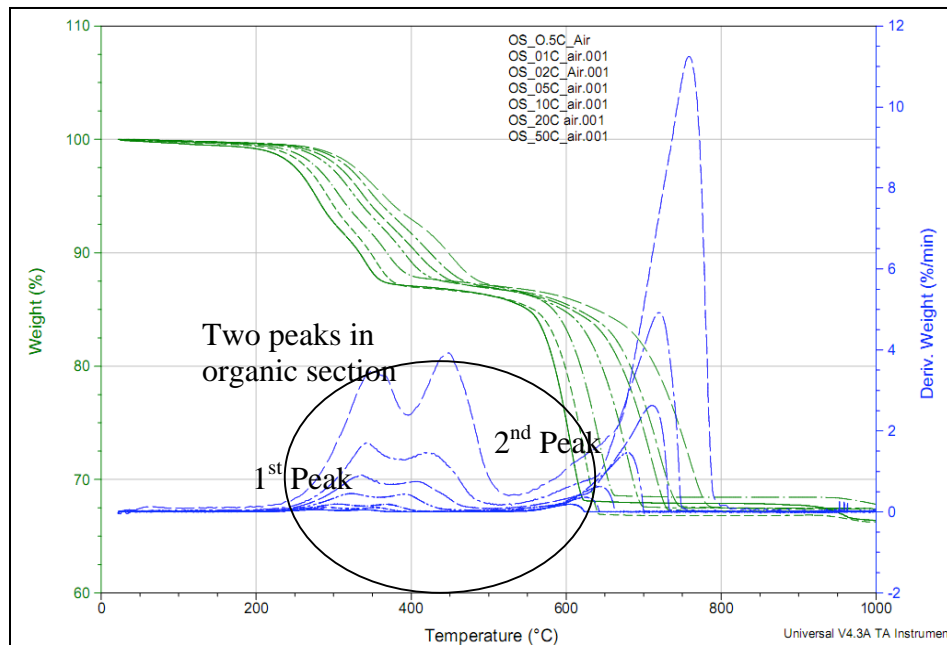
Figure -7: Non-isothermal TGA combustion curves. Rates go from 0.5°C/min to 50°C/min.
