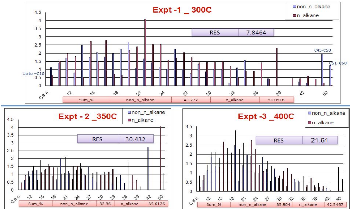
Figure – 34: Normal alkanes, non-normal alkanes and residue % in the oil samples – Set_1.
