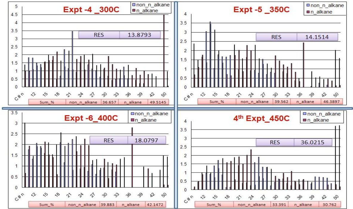
Figure – 35: Normal alkanes, non-normal alkanes and residue % in the oil samples – Set_2.
