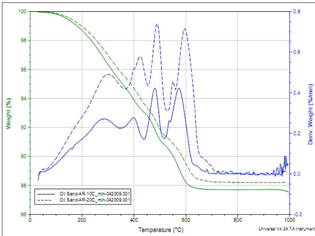
Figure – 41: Non-isothermal TGA curves for Asphalt Ridge oil sand pyrolysis at 10°C/min (31.474 mg) and 20°C/min (31.478 mg) heating rates.
