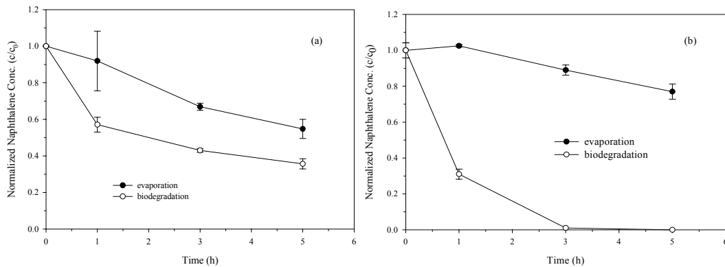
Figure 6: Biodegradation of naphthalene by bacteria enriched with: (a) naphthalene plus glucose as carbon source; (b) naphthalene only as carbon source.
