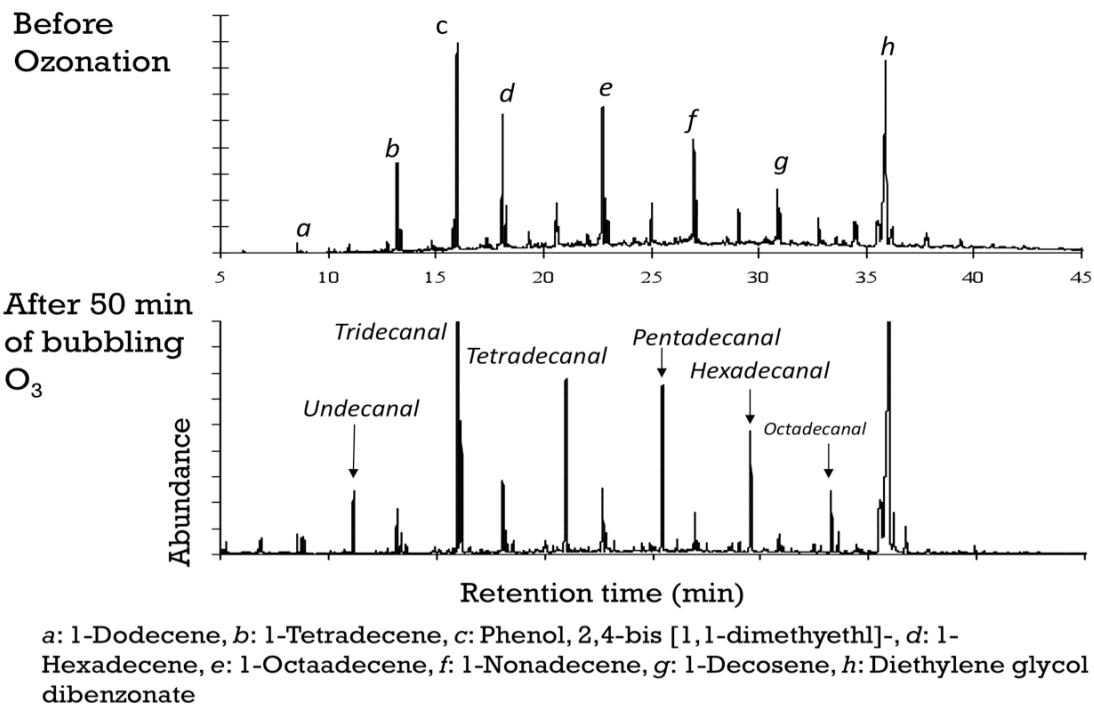
Figure 4b. GC/MS Analyses - Hexane-extractable intermediates before and after 50 minutes of regular ozonation.
