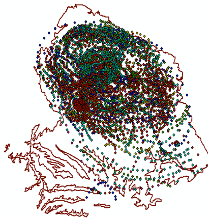
Figure 11. Point features of Isopach Rich and Lean zones in Piceance Basin Study Area (Mahogany Outcrop).
