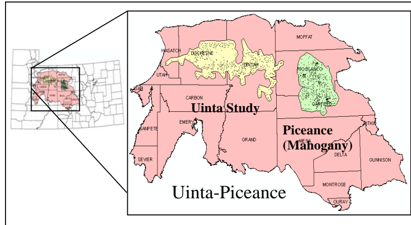
Figure 9. The Uinta (yellow) and Piceance (green) Basins are located in eastern Utah and western Colorado, respectively.
