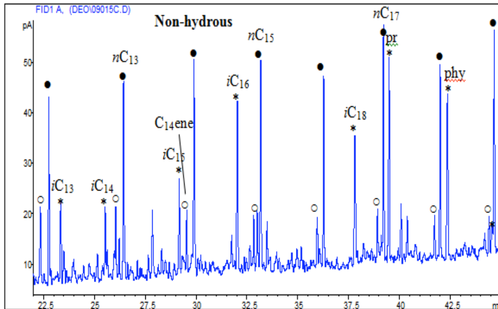
Figure – 39: Expanded chromatogram of a product from non- hydrous pyrolysis.
