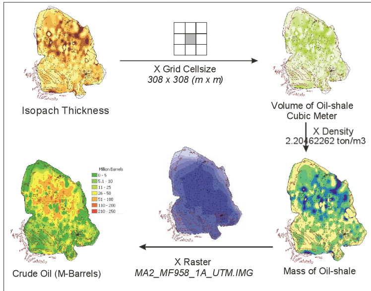
Figure 13. An example of the oil yield calculation of Mahogany Outcrop, Piceance Basin, Colorado (application of equations 1-4).
