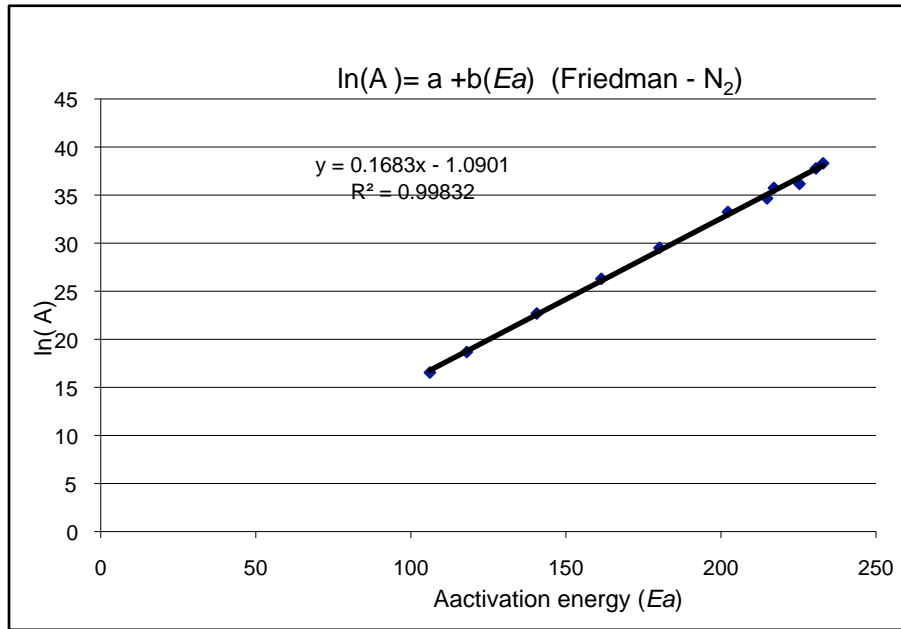
Figure - 31: Tradeoff between activation energy and pre-exponential factor for the pyrolysis kinetic data obtained by the Friedman approach.
