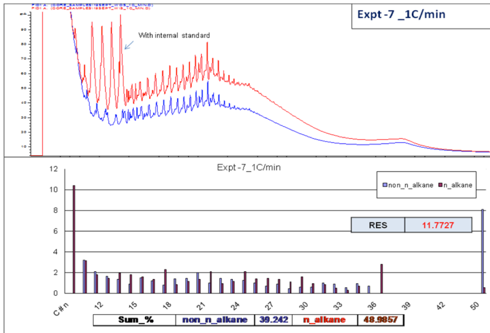
Figure – 36: Chromatogram and normal alkanes, non-normal alkanes and residue % in the oil sample from pyrolysis of core at 1°C/min.
