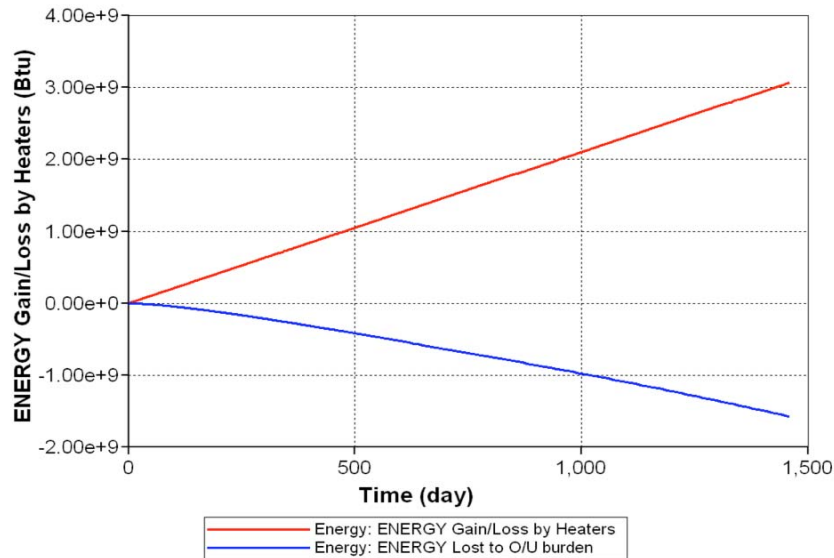
Figure 17. Energy supplied to reservoir and energy lost to under/overburden.
