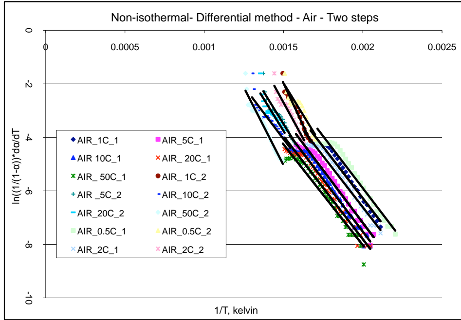
Figure - 18: Analysis of non-isothermal TGA combustion data (two-step) using the differential method.
