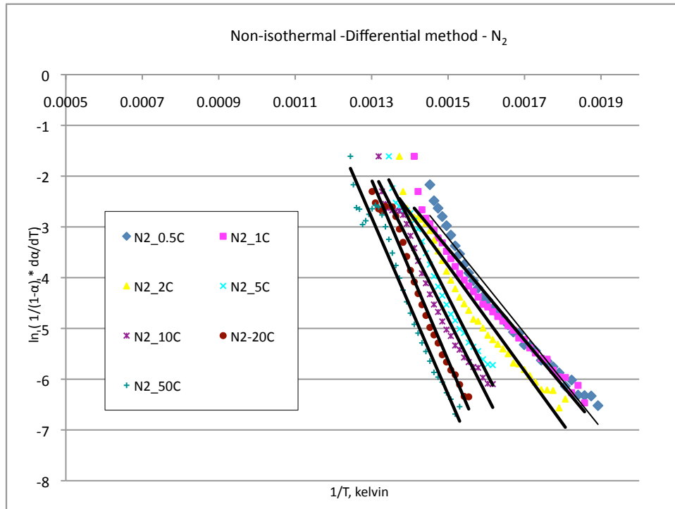
Figure - 16: Analysis of non-isothermal TGA pyrolysis data using the differential method.
