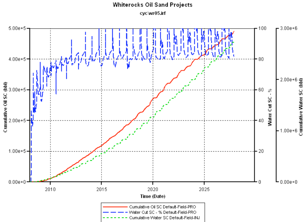
Figure 8: Oil production in Whiterocks cyclic simulations.
