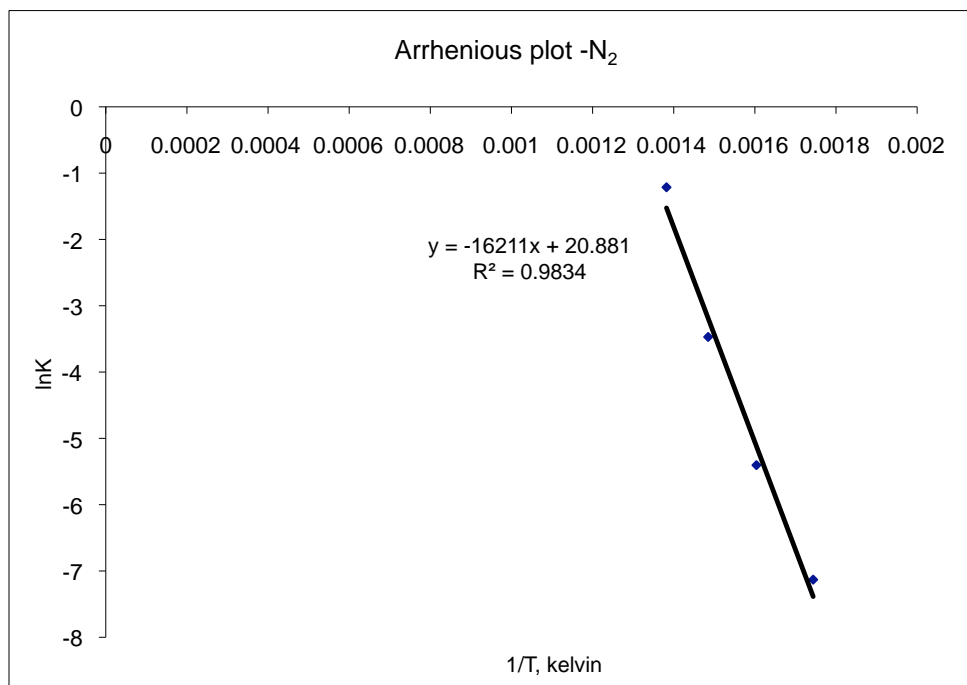
Figure- 12: Arrhenius plot for 1 st order isothermal TGA pyrolysis experiments: ( E_a = 134.77 kJ/mol and A = 1.2E+09 min -1 ).
