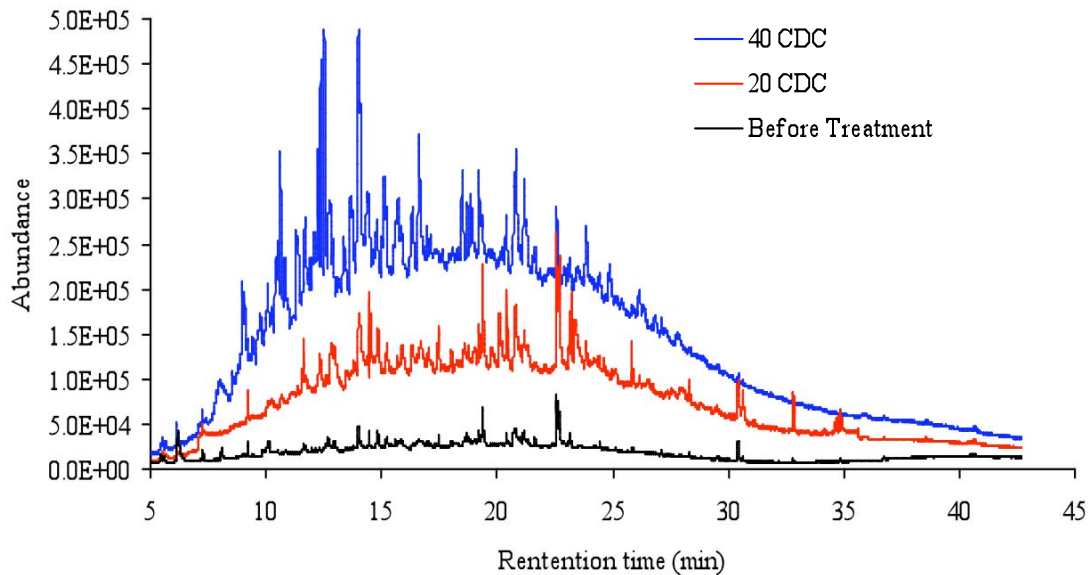
Figure 6. GC/MS Analyses – Hydrophilic products in treated produced water. Note: CDC = cyclic compression/decompression
