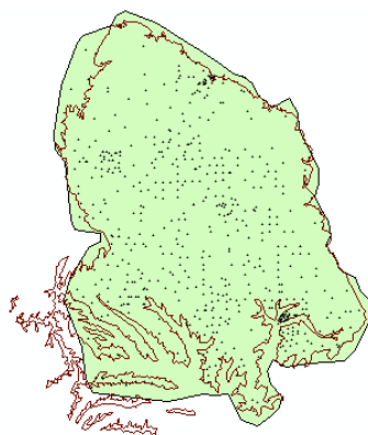
Figure 12. Isopach and in-place oil resources (587 points) of the Piceance Basin Study Area (Mahogany Outcrop) [21].
