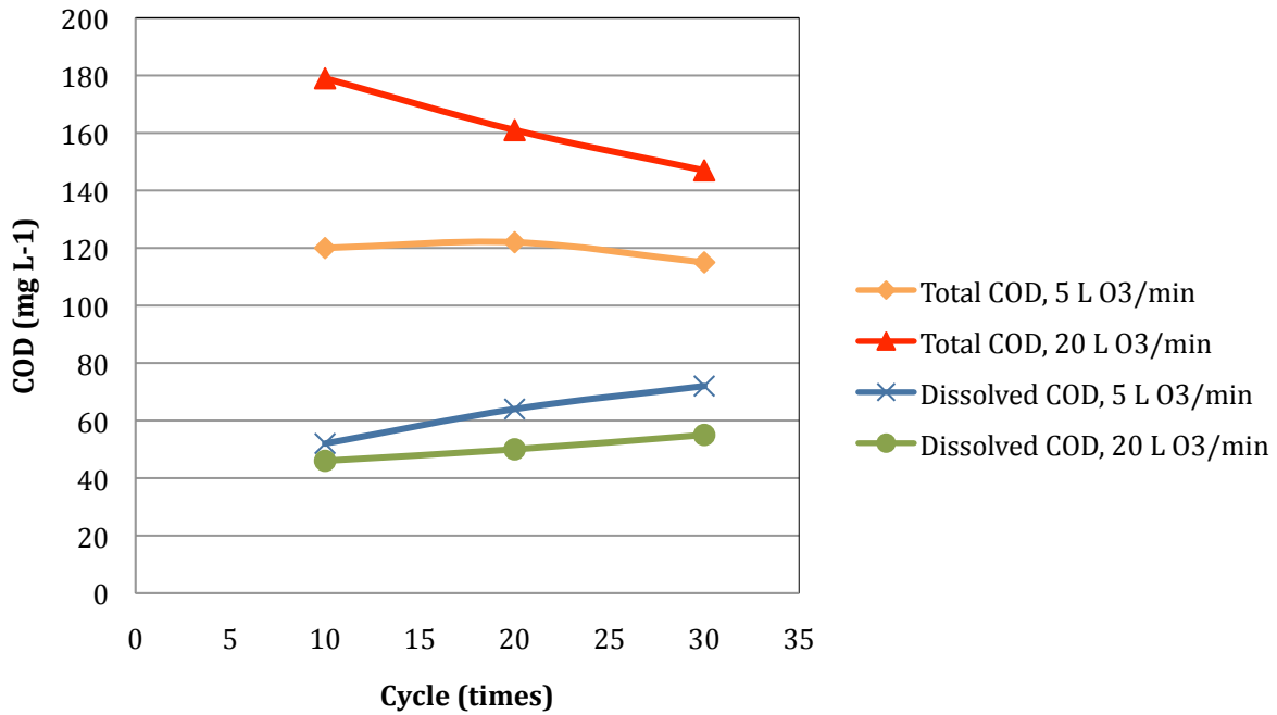
Figure 2. Hydrophilic products generated during treatment of produced water.
