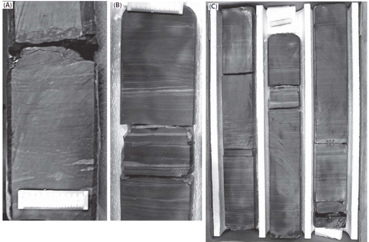
Figure 5. A) Black, organic-rich, and friable oil shale (328.88 m depth in litholog of Figure 4). B) Mahogany Bed, the richest oil shale bed in the Mahogany Zone, which is the richest oil shale zone in Green River Formation (219.46 m depth in Figure 4). Core base is bottom-right and top is upper-left. C) Details of the Mahogany Bed. Lighter interlamination are kerogen-poor calcareous and dolomitic mudstones (218.54 m depth in Figure 4). Note that scale is 5 cm long in all photos.
