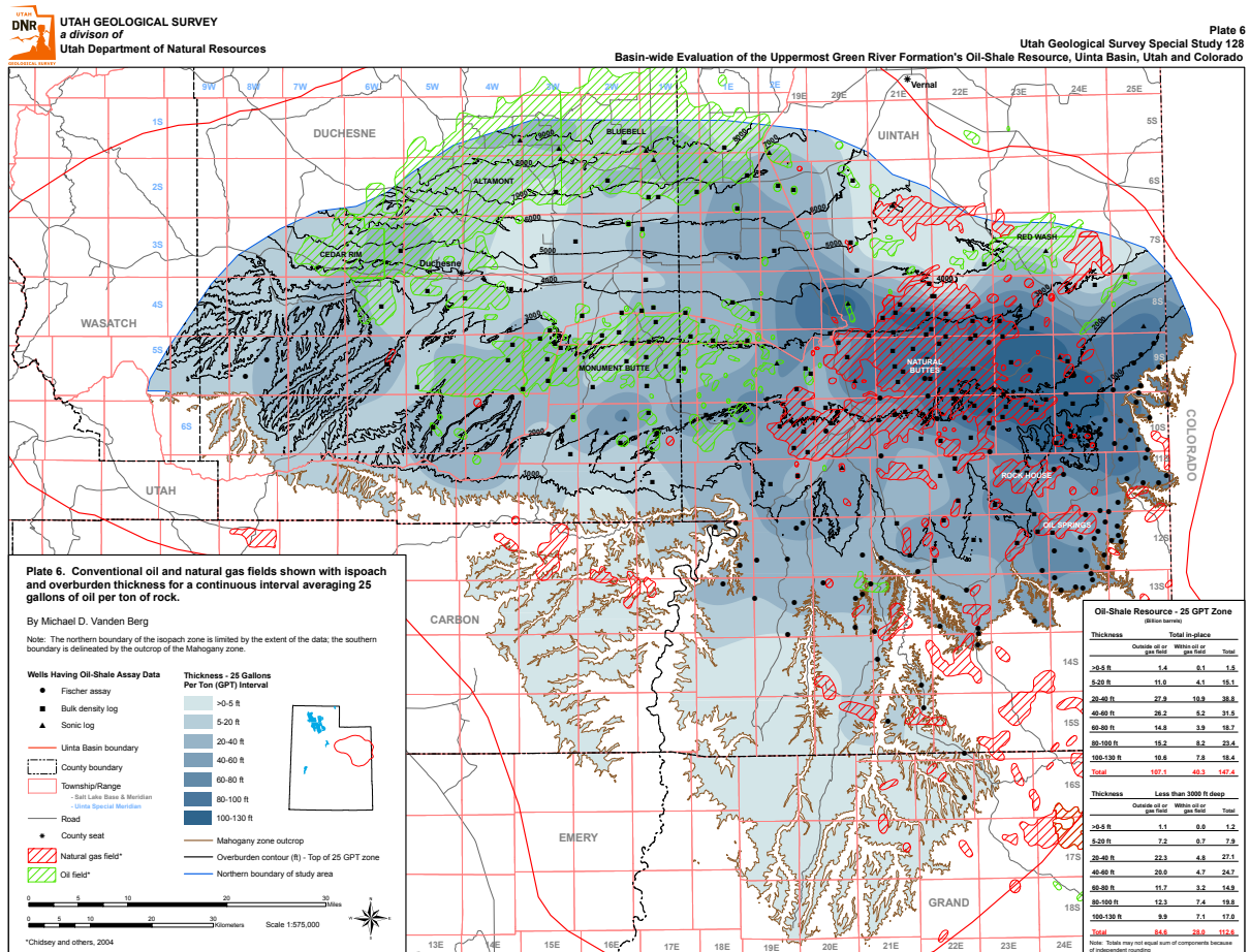
Figure 4.6.1: Basin-wide Evaluation of the Uppermost Green River Formation's Oil-Shale Resource, Uinta Basin, Utah and Colorado. Source: Michael D. Vanden Berg, Utah Geological Survey Special Study 128, Plate 6.
