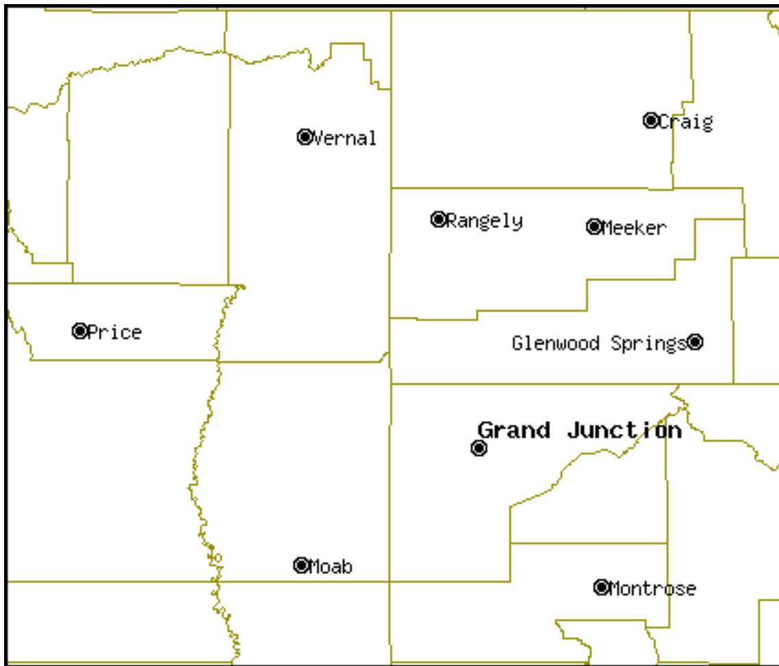
Figure 8.2.11: Map of Counties within the Most Prospective Oil Shale Area.
