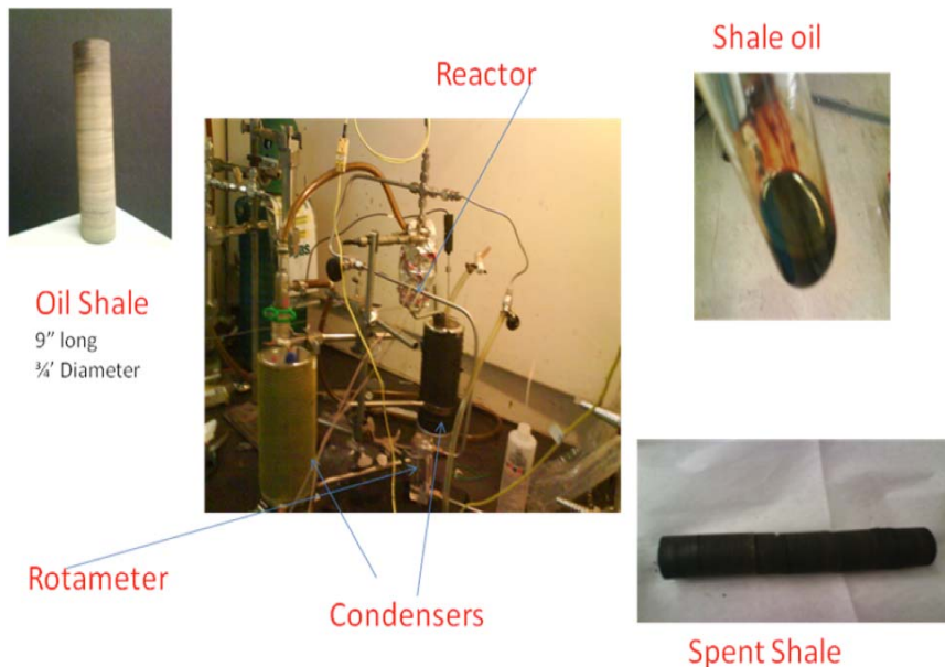
Figure – 3: Images of the small reactor section, raw sample and products.
