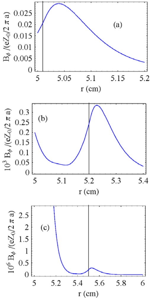
Figure 6: Radial dependence of the m=1 harmonics within the wall for (a) \Delta=0.01 cm, (b) \Delta=0.2 cm, and (c) \Delta=0.5 cm. The vertical line corresponds to the radius of a+\Delta . The radial behaviour shows the resonance character
