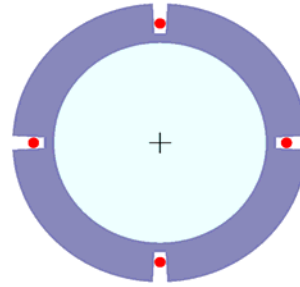
Figure 5: Sketch of the BPM design. Red circles show longitudinal wires located in the grooves.
