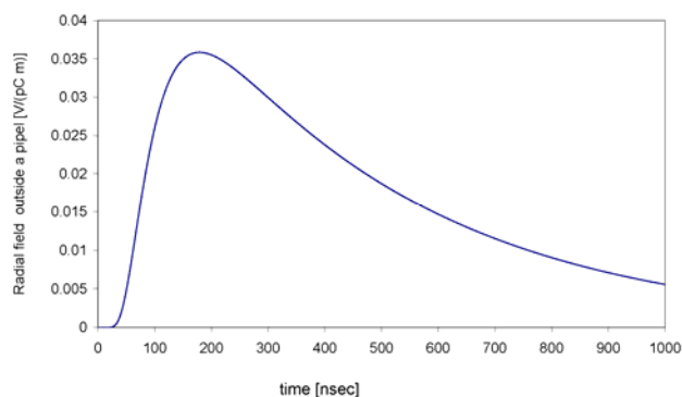
Figure 2: Field outside of the Al 0.5 mm round beam pipe.
