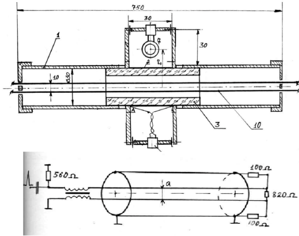
Figure 3: Schematic view of the experimental set-up and electrical diagram of the transmission line. 1- aluminium pipe, 2 – 50 micron stainless steel foil, 3 - Plexiglas foil support, 7 - measuring coil, 10 – two-wire transmission line.
