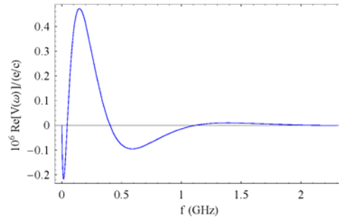
Figure 7: Spectral density of the voltage induced by a dipole harmonics of a single particle for wire length of L=10 cm.
