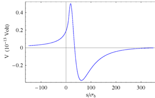
Figure 8: Voltage induced in the wire loop by the dipole harmonics of the azimuthal magnetic field of a single beam particle for \Delta=0.01 cm.
