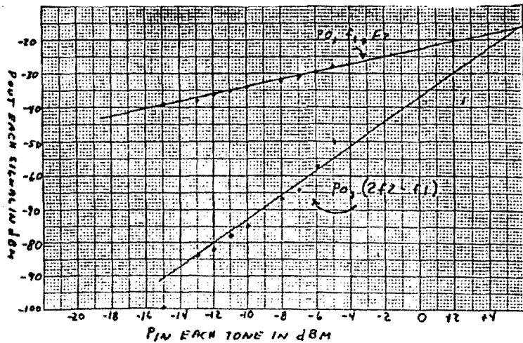
Fig. 8. Third Order Products at Output of FOL
