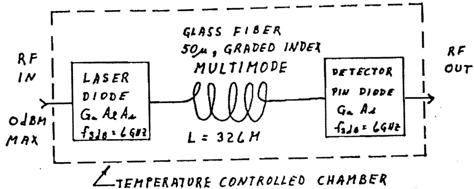
Fig. 1. Major FOL Components
