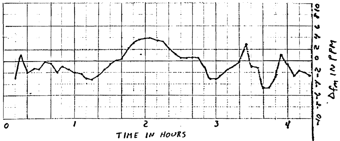
Fig. 9. FOL time delay variation with FOL operating on a table top in a room ambient air temperature of \sim 72^\circ\text{F} . The FOL temperature regulator was set to maintain the FOL chamber at 65^\circ\text{F} .
