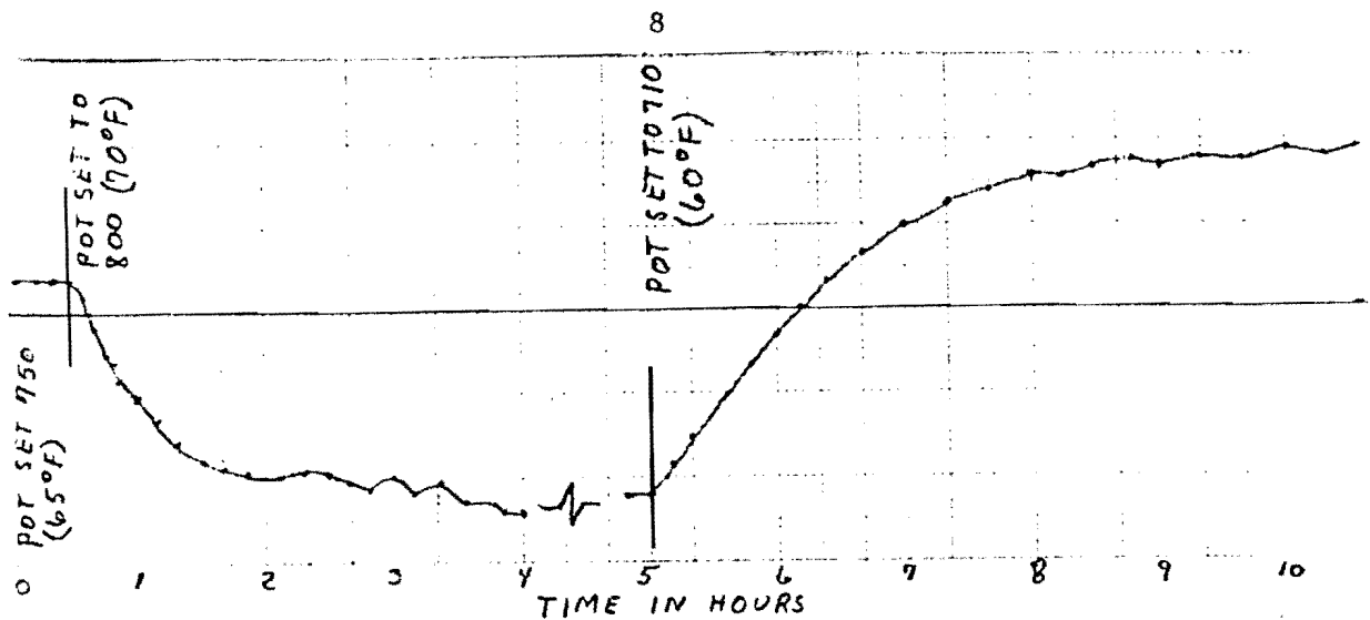
Fig. 11. This data shows the FOL's effective length sensitivity to regulated temperature values and the time needed to reach stability at newly selected FOL temperatures.
