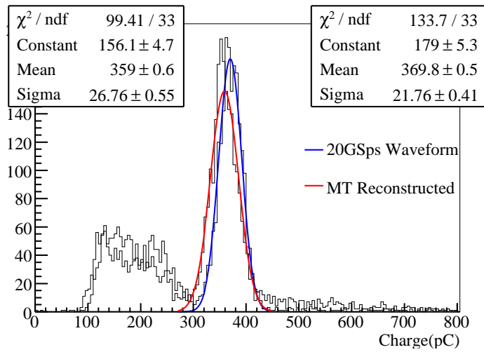
Figure 5: Pulse-height spectrum obtained from the samples generated by our MT-sampling prototype (red curve), showing an \sim 18\% energy resolution at 511 keV, and that from thousands of samples generated by using a Tektronix TDS6154C oscilloscope at 20GSps, showing an \sim 13\% energy resolution at 511 keV. See Section 2.3 for the analysis methods generating the pulse height.
