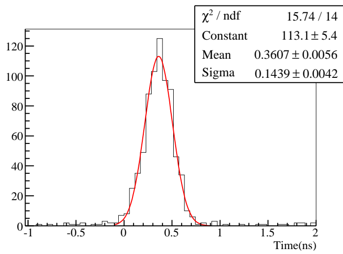
Figure 7: The differential time in coincidence measurement obtained from two samples on the rising edge of the pulse generated by the MT-sampling prototype. The distribution shows a coincidence timing resolution of \sim 340 ps FWHM.
