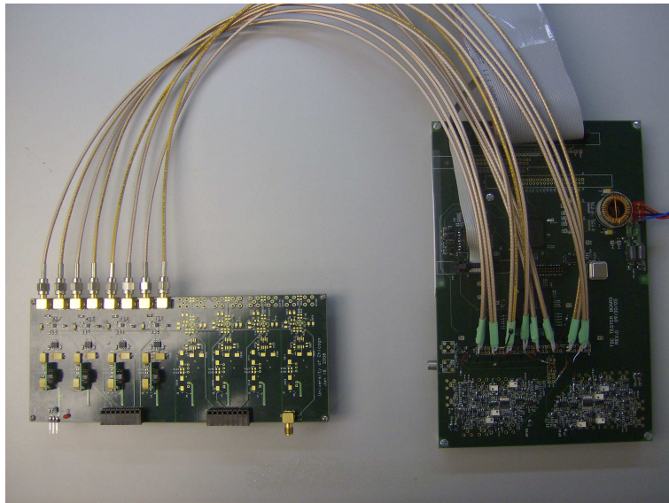
Figure 1: A multi-threshold discriminator board (left) and the TDC board (right). The discriminator can provide up to 8 thresholds for sampling its input signal. Currently, four channels have been implemented. The discriminator outputs are connected to the HPTDC chip on the TDC board. The HPTDC chip, developed at CERN, can provide 8 TDC channels at 24.4 ps/bit resolution.
