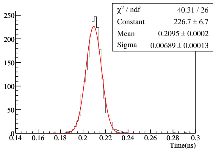
Figure 4: A sample histogram showing the time offset between the outputs of two channels on the same multi-threshold board. The peak position gives the time offset between the two channels and the width shows the timing jitter, which is \sim 16.2 ps in FWHM in this case. The width of the other channel combination shows similar values, and the average timing jitter of a single channel was estimated to \sim 12.5 ps in FWHM.
