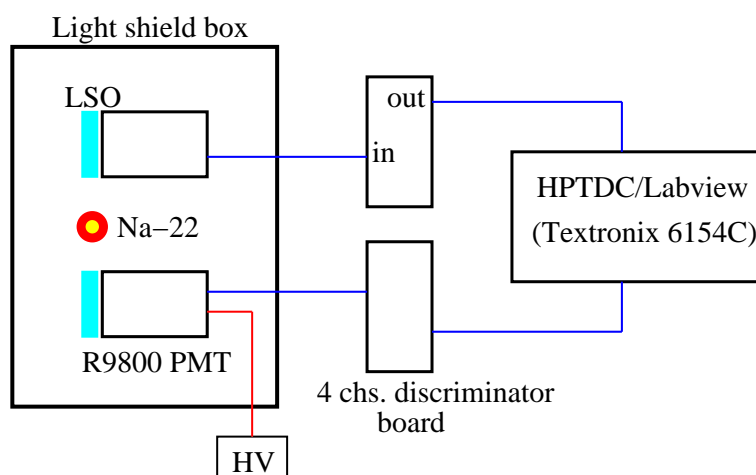
Figure 2: Block diagram of the test setup. Four outputs from each discriminator boards were connected to HPTDC for time digitization. The PMT signals were directly fed to the oscilloscope to read out waveform.
