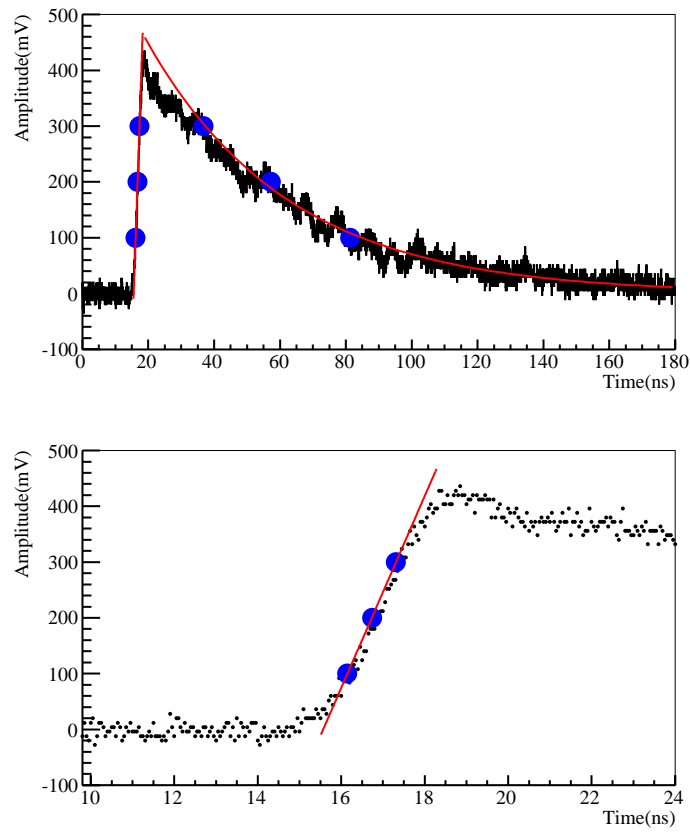
Figure 3: Waveform vs. multi-threshold sampling. Samples acquired by the MT sampling are marked with blue points. The line fitting on the rising edge and the exponential fitting on the trailing edge were applied to reconstruct the pulse shape. The waveform of PMT signal with 20 GSps sampling was shown in black.
