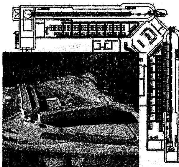
Figure 2. Aerial photograph of the Los Alamos DARHT facility overlaid on a line drawing showing the first axis accelerator (right) and the second axis accelerator (top).
