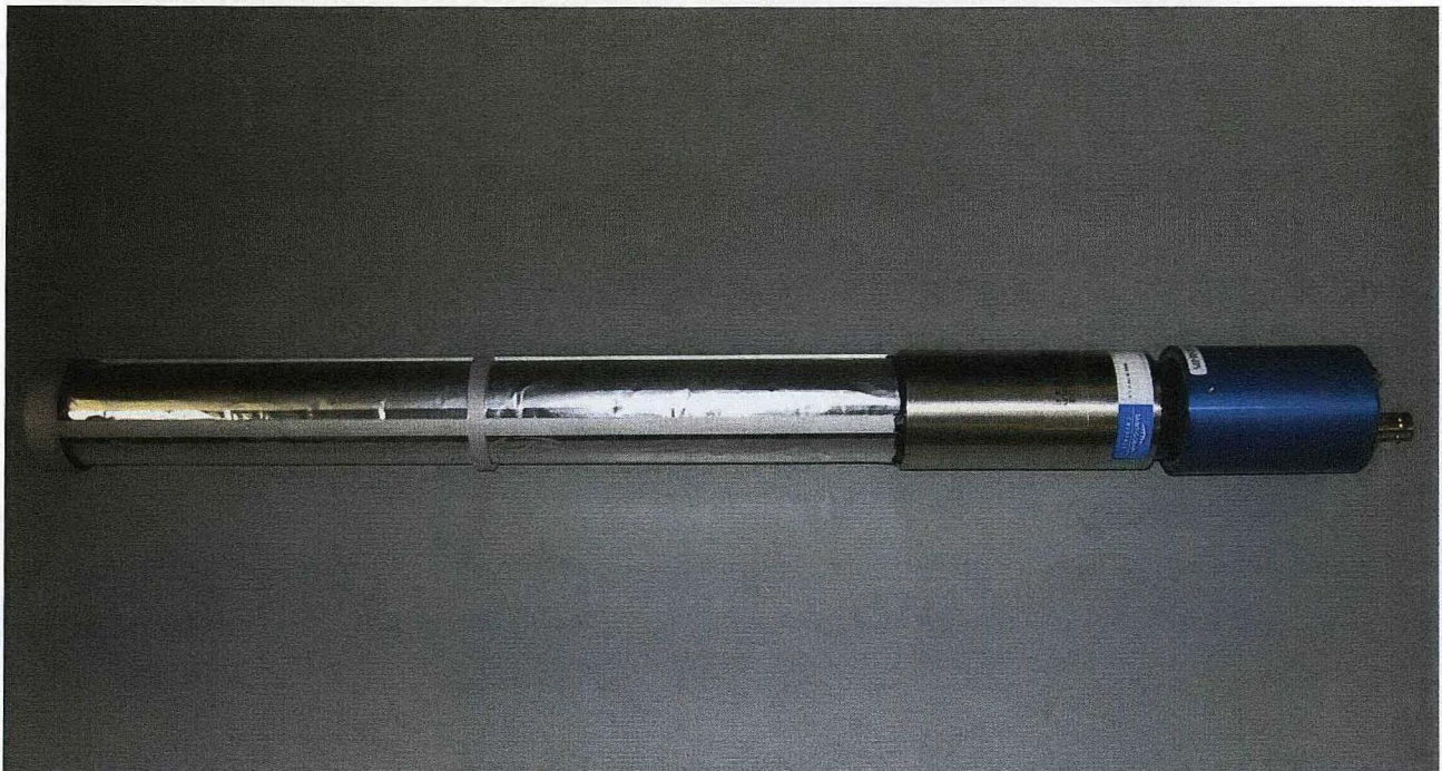
Fig. 3. Prototype in-situ beta detection probe.
