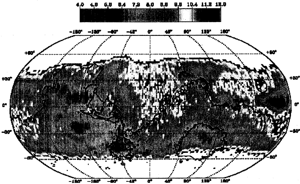
Figure 7 (below). Mid-latitude map of the partial macroscopic absorption cross section (the contribution from hydrogen is removed). The units are 10^{-3} \text{ cm}^2/\text{g} . A contour of topography at 0 km elevation is superimposed on the map.
