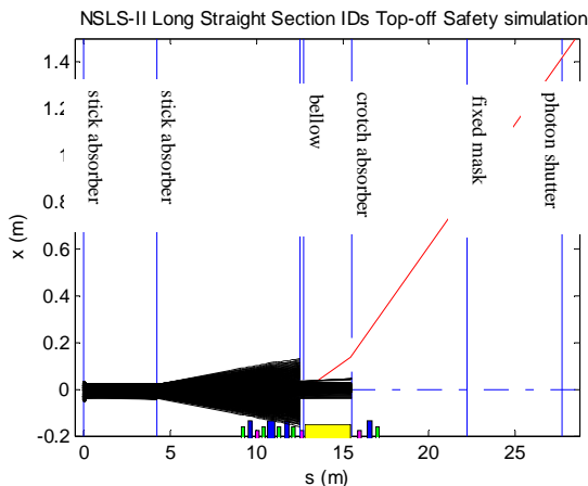
Fig. 4: Beam trajectories (in black) in the normal condition. The central orbit of electron beam (blue dash line) is chosen as the reference, red solid line is the photon beamline centre, and blue solid lines are collimators.
