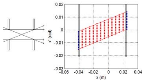
Fig. 3 Determination of initial phase space area for forward tracking by four extreme rays
