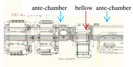
Fig. 5: Two ante-chambers are separated by a bellow
