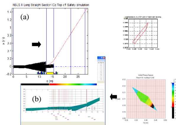
Fig. 1: Forward (a) and backward (b) tracking
