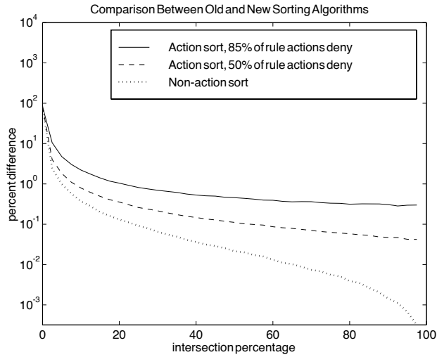
Figure 8: Percent decrease in the number of rule comparisons as the dependency percentage increases for a 1000 rule policy. The new sorting algorithm (action sort) performs better.
