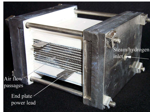
10-cell stack (2004) 640 cm 2
