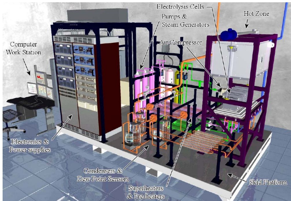
Figure 4. Rendering of Integrated Laboratory Scale experimental facility
