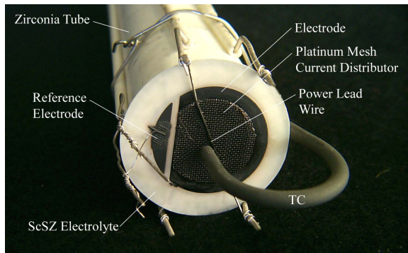
Button Cell (2003), 3.2 cm 2
