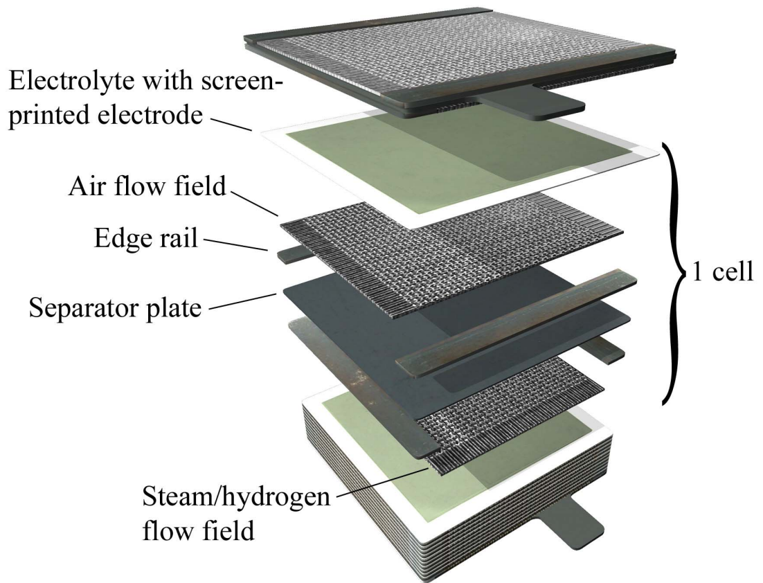
Figure 2. Ceramatec's solid oxide cell/stack construction
