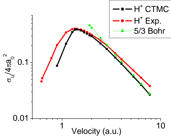
Fig. 2. Normalized ionization cross section for proton collisions with atomic hydrogen in atomic units; the value of the cross section is normalized to 4\pi a_0^2 = 3.517 \cdot 10^{-16} \text{ cm}^2 ; the velocity in atomic units can be calculated from the projectile energy per unit mass from
