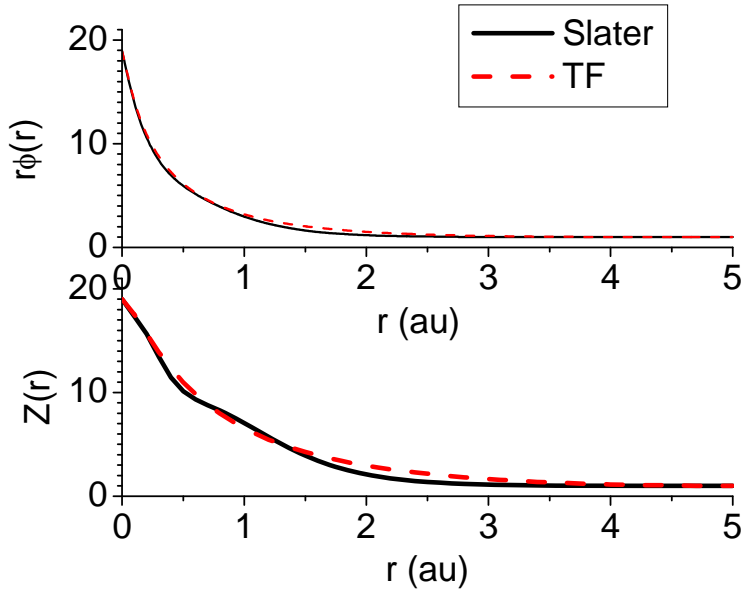
Fig. 10 Comparison of the Thomas-Fermi and Slater models for the potassium ion potential, r\phi(r) , and profile of charge, Z(r) , inside of a sphere of radius r . Note the differences between the two models at the outer edge of the ion. The orbital structure is evident for the Slater model.
