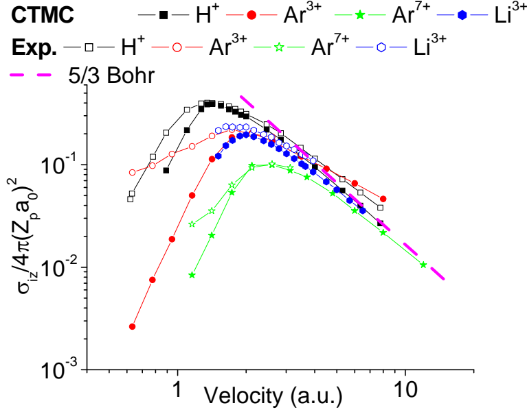
Fig. 5. Ionization cross sections of argon ions ( \text{Ar}^{+3} and \text{Ar}^{+7} ) compared with fully stripped ions of the same charge ( \text{H}^+ and \text{Li}^{+3} ) on atomic hydrogen. The experimental values for the Ar ions are taken from Ref. [26].
