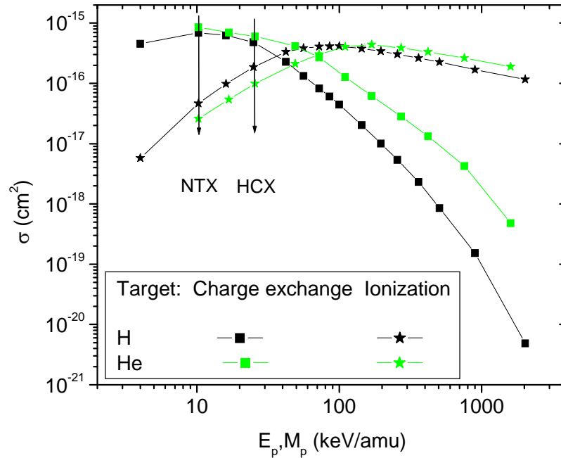
Fig. 8. Charge exchange and ionization cross sections of atomic H and He target ions interacting with K^+ ions, predicted using CTMC calculations. The HCX parameters (1 MeV K^+ ion) correspond to 25 keV/amu.
