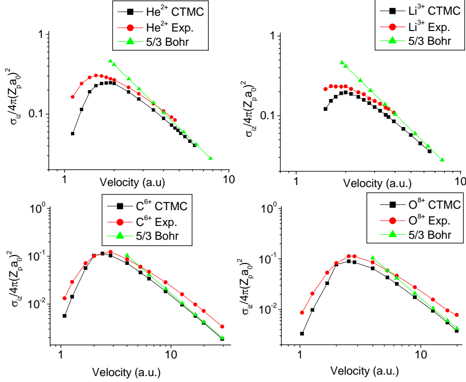
Fig. 3. Normalized ionization cross sections for fully stripped ions colliding with atomic hydrogen; the value of the cross section is normalized to 4\pi a_0^2 Z_p^2 = Z_p^2 3.517 \cdot 10^{-16} \text{ cm}^{-2} . The experimental results for He, Li, and C and O are from Refs. [23], [24], and [25], respectively.
