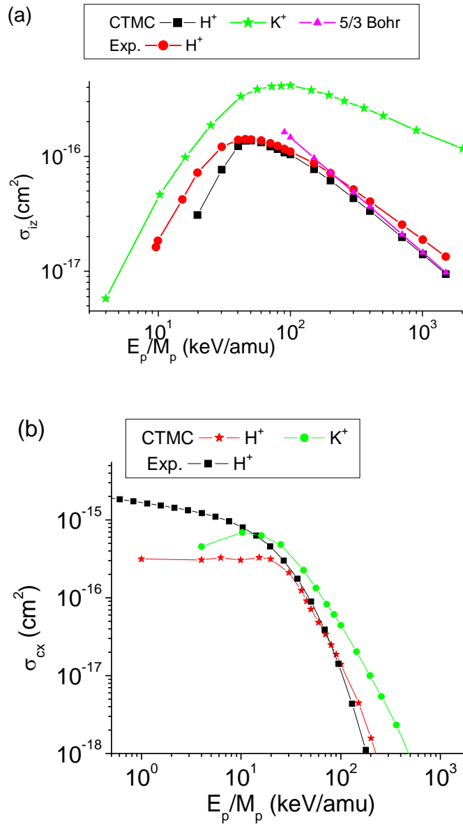
Fig. 9. Comparison of ionization cross section (a) and (b) charge exchange cross sections for proton and potassium ion projectiles colliding with atomic hydrogen. The experimental data are from Refs. [1,3].
