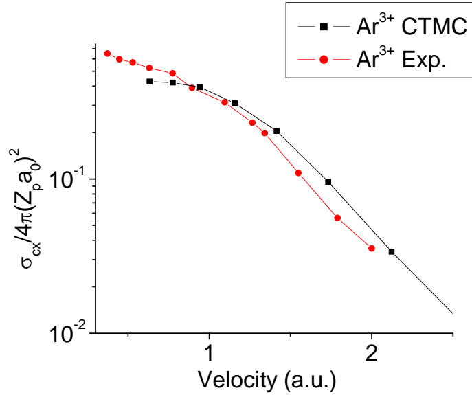
Fig. 6. Charge exchange cross sections for collisions of argon ions ( \text{Ar}^{3+} ) with atomic hydrogen. The experimental values were taken from Ref. [26].
