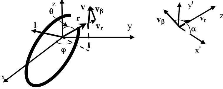
Fig. 1. Schematic of electron trajectory and definition of the angles (\theta, \phi, \alpha) .
