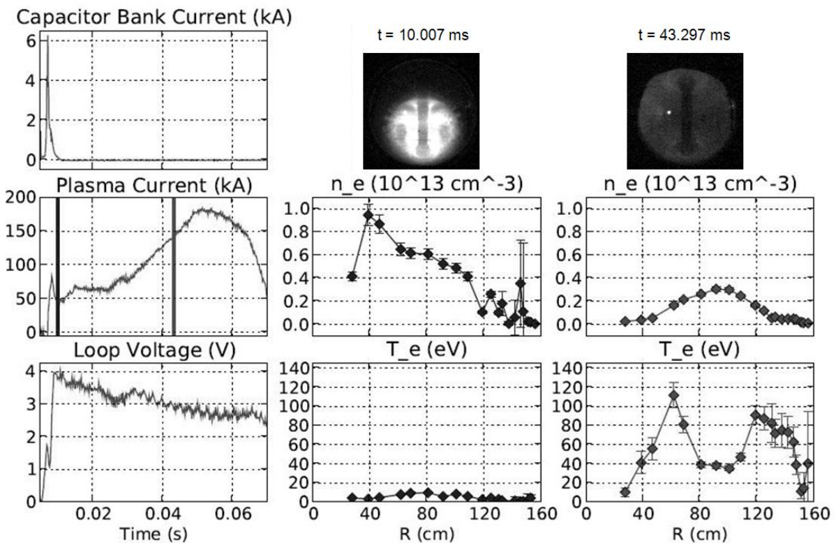
Figure 2: Shown are from top to bottom: Left column – injector current, plasma current, loop voltage for discharge 128108, Middle column – camera image during the CHI phase, density and temperature profiles at 10ms, Right column – camera image electron density and temperature profiles at 43ms.
