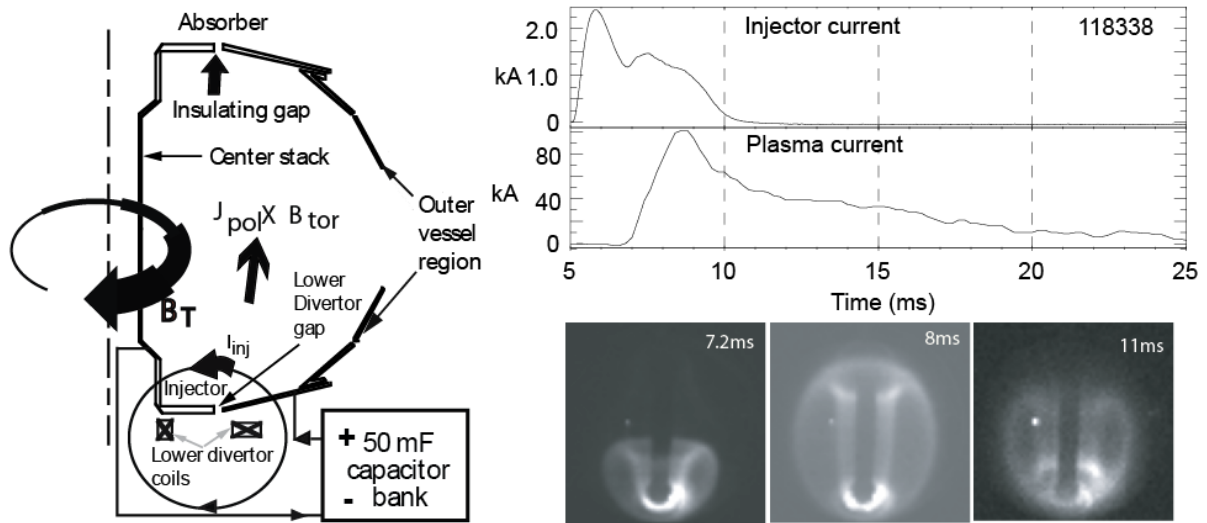
Figure 1: Shown are: Left – line drawing to identify the main components needed for CHI operation, Right Top – CHI injector current and plasma current and Right Bottom – Fast camera fish eye images for discharge 118338.
