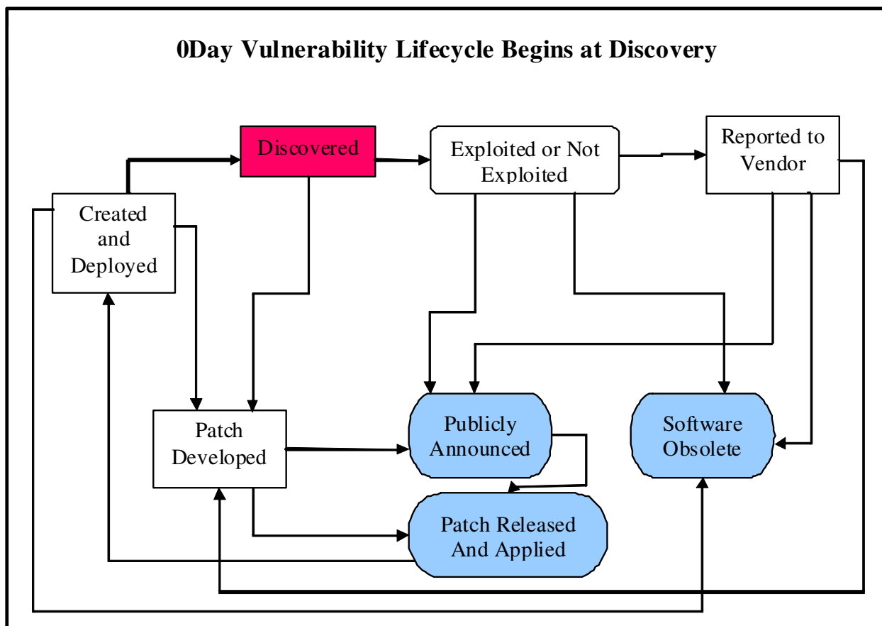
Figure 1. Vulnerability Lifecycle.
