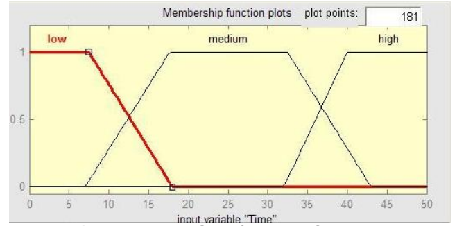
Figure 4. Input Fuzzy Sets for Time Concept
