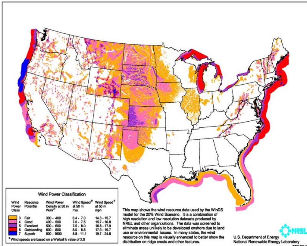
FIGURE 2. The wind resource potential at 50m on land and offshore.
