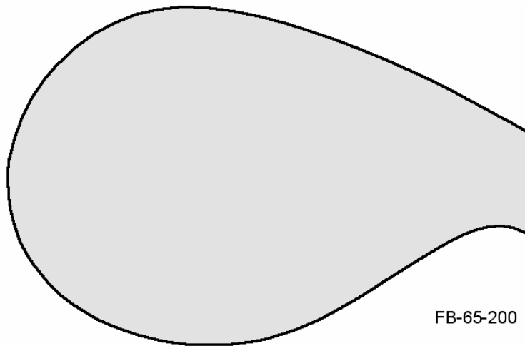
FIGURE 9. A flat-back thick airfoil shape with high structural efficiency and easier highway transport.
