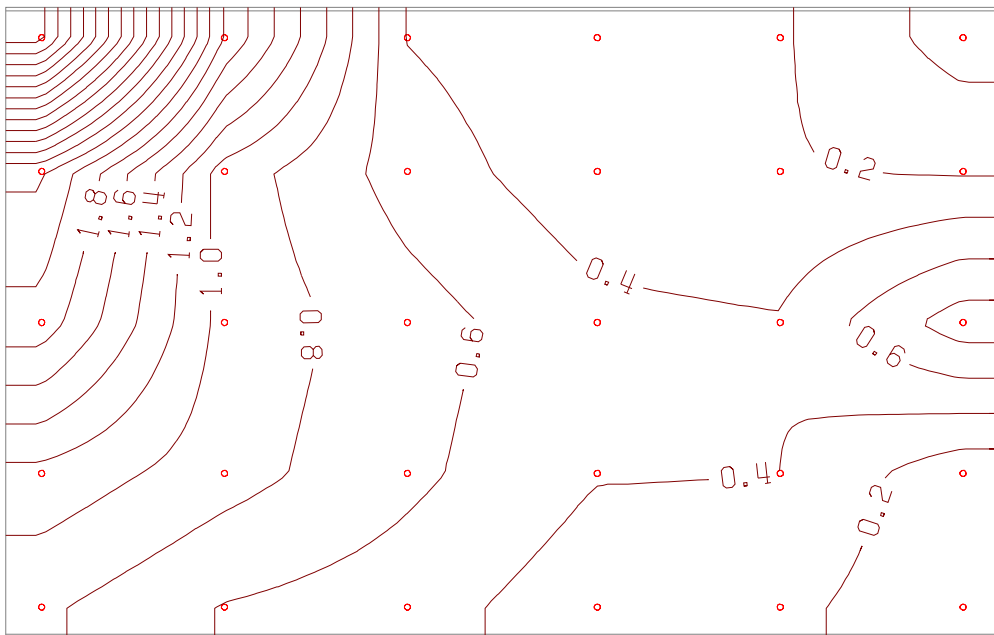
Peak Positive Differential Pitch: 15 deg. Configuration B3 (continued)
