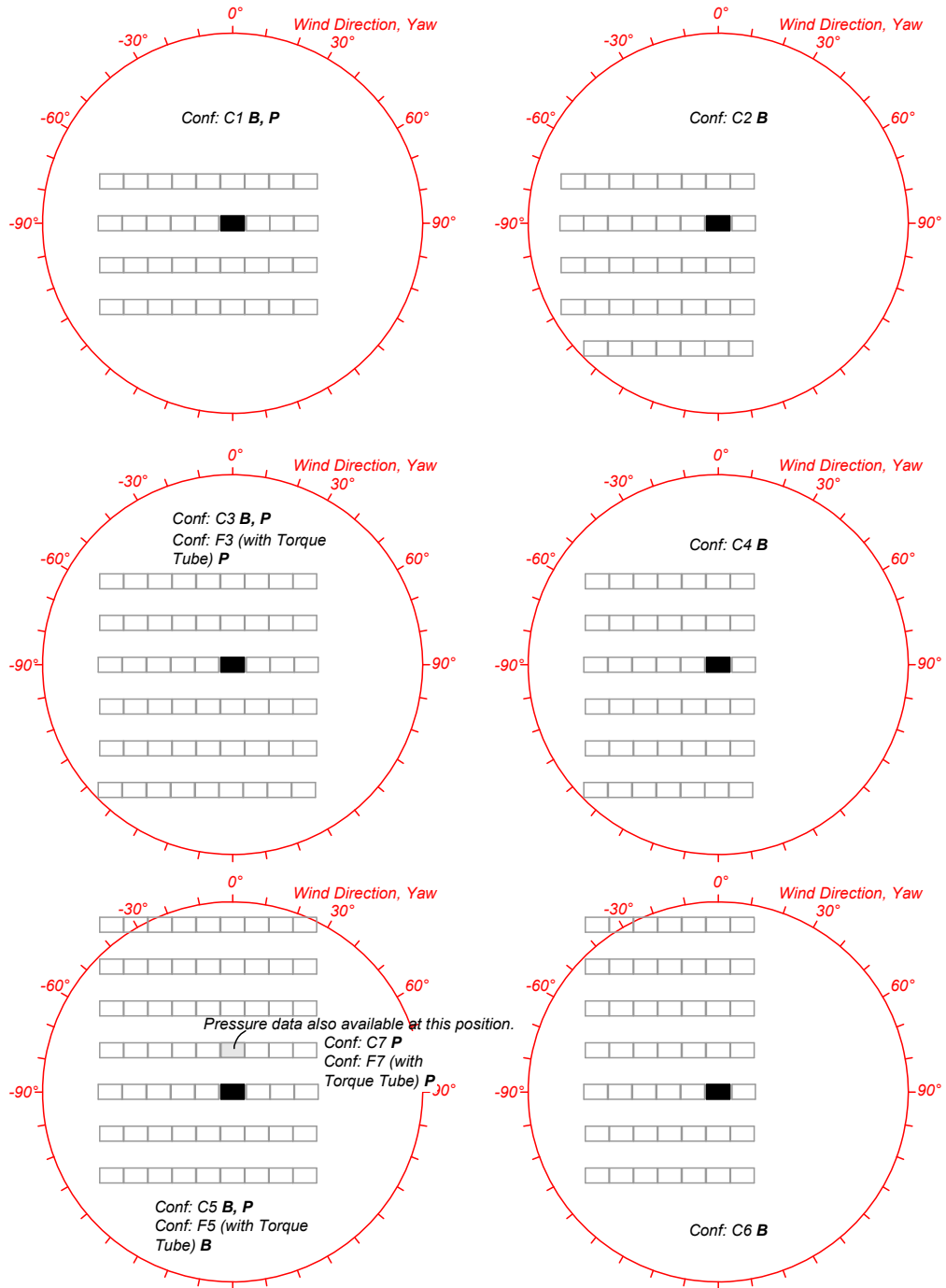
Figure 2-11b Test configurations for array field study, interior field
