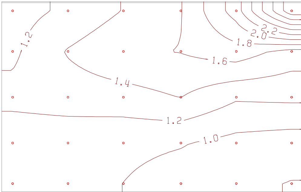
Peak Positive Differential Pitch: -60 deg. Configuration D1 (continued)
