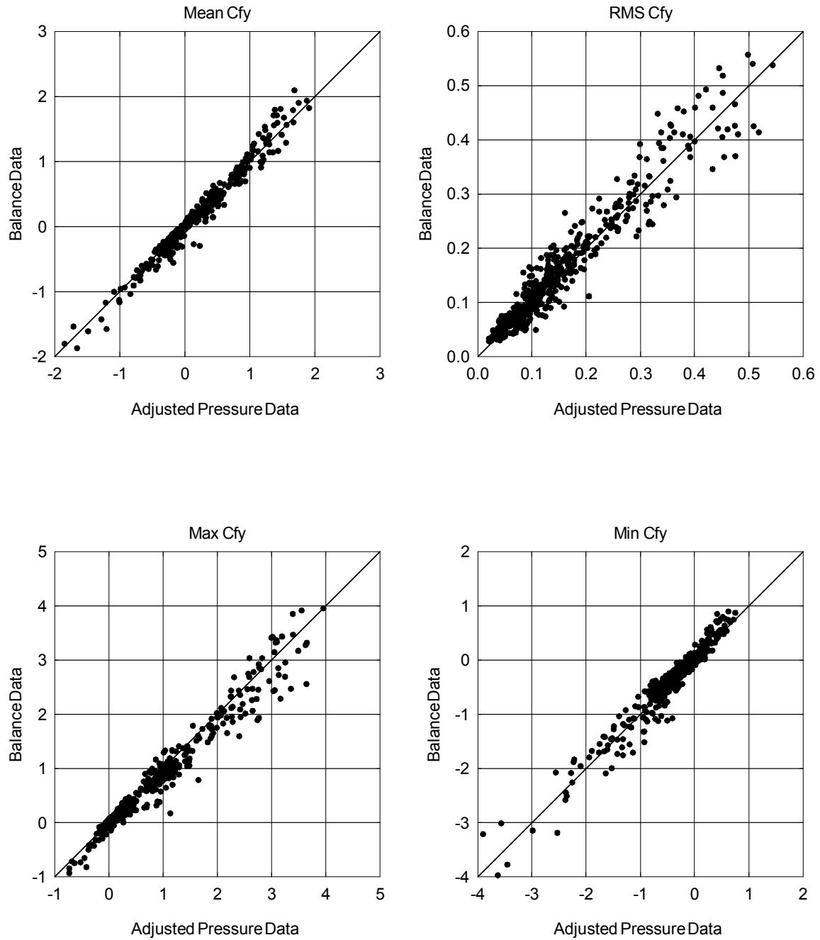
Figure 4-40 Comparison of Balance and Adjusted Pressure Data, (b) Vertical Force Component
