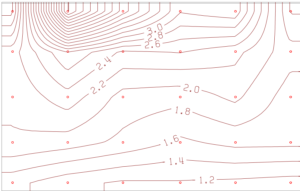
Peak Positive Differential Pitch: -60 deg. Configuration C5 (continued)
