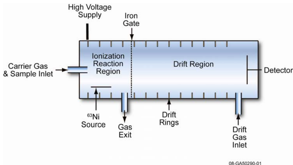
Figure 1. Basic configuration of an ion mobility spectrometer.
