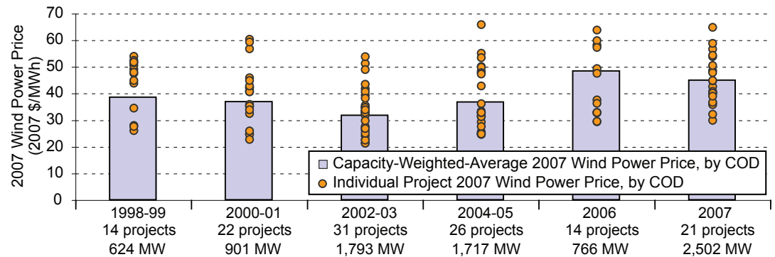
Figure 13. Cumulative Capacity-Weighted-Average Wind Power Prices Over Time
