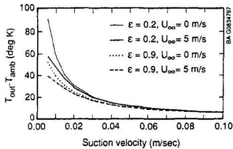
Figure 1 Efficiency and temperature rise of transpired solar collector Figure taken from Kutscher et al. (1993), 0.01 \text{ m/s} \cong 2 \text{ FPM} , 700 \text{ W/m}^2
