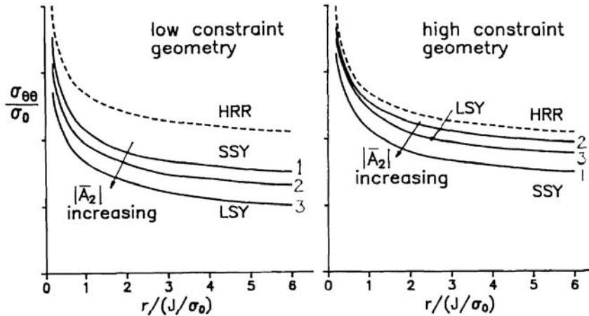
Figure 2a Stress ahead of a crack tip in low constraint specimen geometry Figure 2b Stress ahead of a crack tip in high constraint specimen geometry
