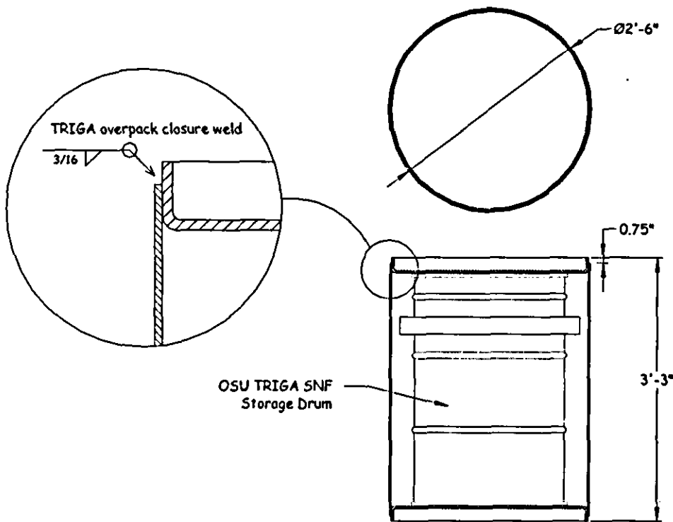
Fig. 1. Overpack sketch and closure weld joint design
