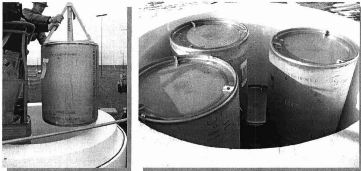
Fig. 5. Packaged overpack placement into the RadVaults
