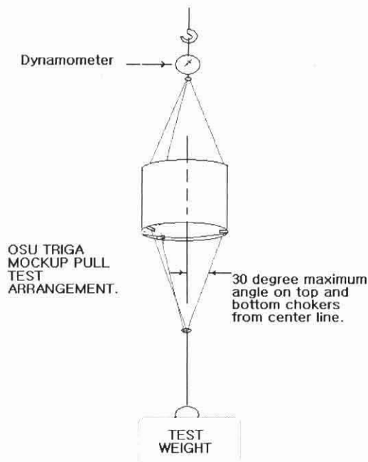
Fig. 3. Setup for pull testing
