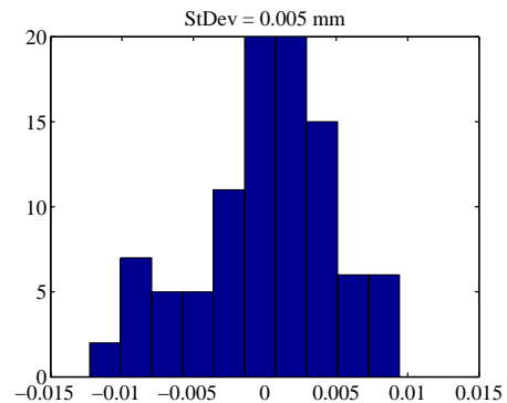
Figure 4: Histogram of the residual (in mm) of the beam position measured in one cavity against the prediction from the two adjacent cavities.
