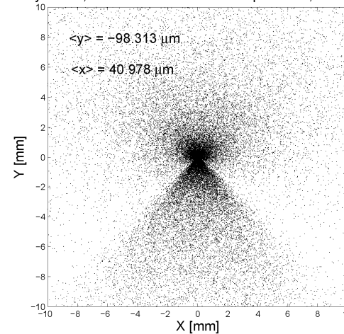
Figure 18: X-Y disrupted beam distributions at Compton IP for the Nominal (top), Large Y-emittance (middle) and Low Power (bottom) parameter options without (left) and with (right) IP y-offset, when solenoid field is turned on without compensation. Here \langle x \rangle and \langle y \rangle are the horizontal and vertical offsets of beam core with |\Delta p/p| < 1\% .
