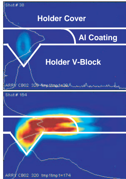
Figure 2: Visible light images (displayed with the same scaled-to-intensity color map) of a 100 \mu\text{m} ID fiber tip as the electron beam pulse current is ramped up. In the top image, the electron beam pulse length is long ( \sigma_z \sim 100 \mu\text{m} ) and the fiber end glows faintly with incoherent optical wavelength emissions. The various boundaries of the fiber holder, which is viewed at an angle of 45^\circ from the beam axis, are also illustrated along with the area in which the fiber's aluminum coating blocks optical emissions. In the bottom frame, the electron beam is near its minimum pulse length ( \sigma_z \sim 20 \mu\text{m} ) and a breakdown event has occurred producing a large flash of visible light.
