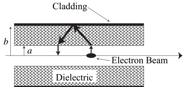
Figure 1: Schematic of the dielectric wake accelerator.
