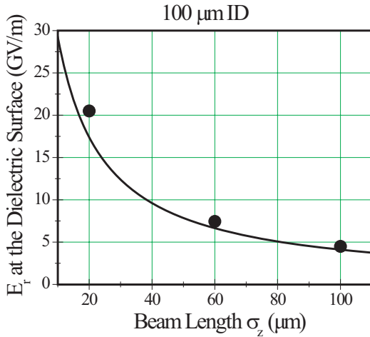
Figure 3: Radial electric field at the inner surface of a 100 \mu\text{m} ID fused silica capillary tube as a function of electron beam pulse length. The black line is the prediction of Eq. 1 and the dots are the results of OOPIC simulations.
