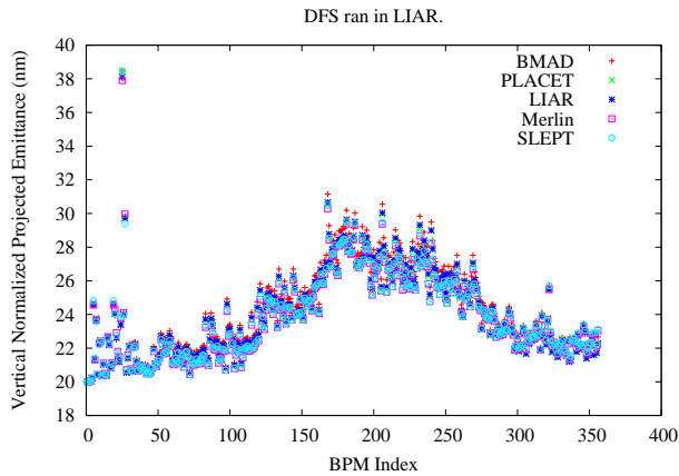
Figure 2: Emittance dilution after performing DFS in LIAR and reading the misalignments and corrector settings into the other codes.
