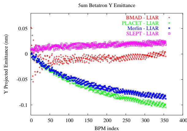
Figure 1: Betatron oscillation emittance growth through the main linac due to a 5 micron vertical offset. Plotted here is the difference in emittance between five codes.
