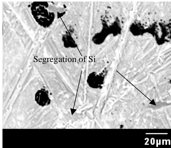
Figure 10 - Microstructure of aluminum alloy 356 before testing.
