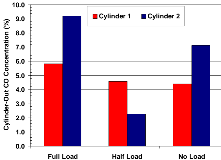
Fig. 3.17. Individual cylinder CO concentration for E0 fueling at three loads for Kohler generator.
