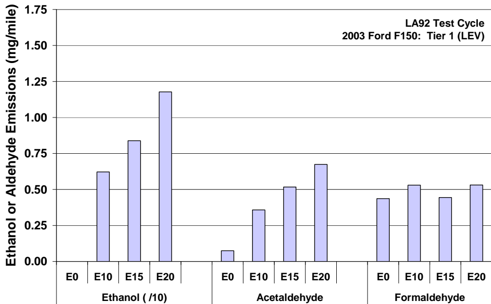
Fig. C.6. Ethanol, acetaldehyde, and formaldehyde emissions for 2003 Ford F150 on LA92 cycle. Bars show average of 3 tests at 75°F.
