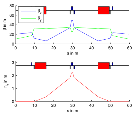
Figure 3: Twiss parameters of the double bend achromat.
