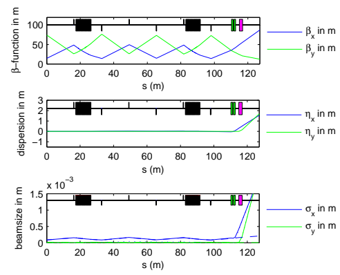
Figure 4: Beam parameters of the abort line for 150 mrad vertical bending angle.
