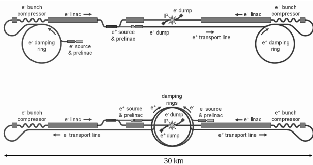
Figure 1: ILC layout with damping ring tunnels at both ends of the main linac (top) and one central damping ring tunnel (bottom).
