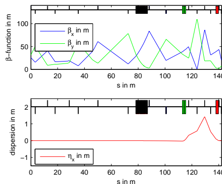
Figure 2: Twiss parameters of the ring connector.
