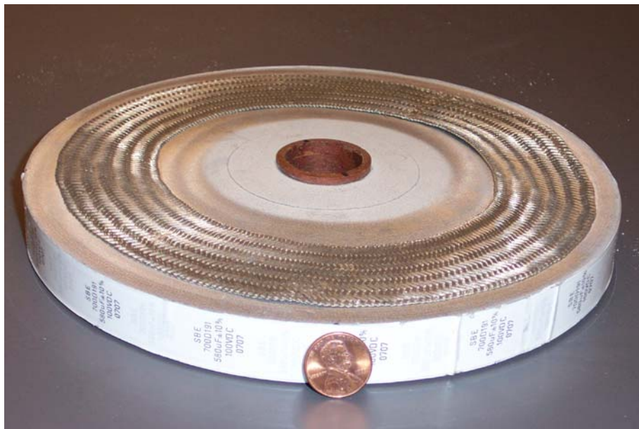
Fig. 2.12. SBE 580 \mu\text{F} 100 Vdc film capacitor.
