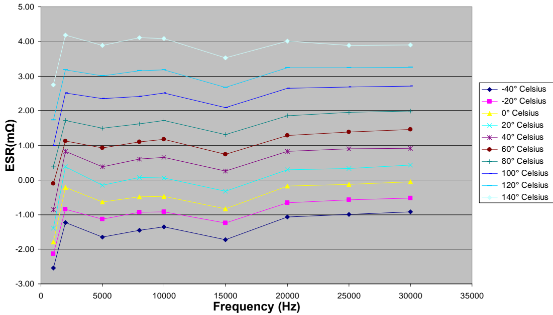
Fig. 2.14. SBE 580 µF film capacitor ESR frequency response.
