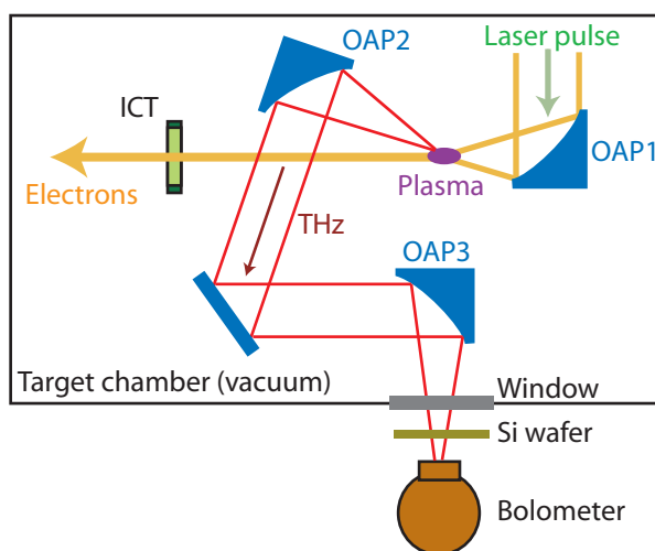
Figure 1: Setup for measurement of the THz pulse energy generated by a 1 MeV electron beam. A 6-inch effective focal length off-axis parabola (OAP) is used to collect partially the THz pulse emitted by transition radiation. A 7-inch OAP is used to focus it back into the bolometer aperture.
