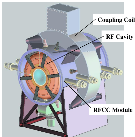
Figure 1. The RFCC Module and Coupling Magnet
