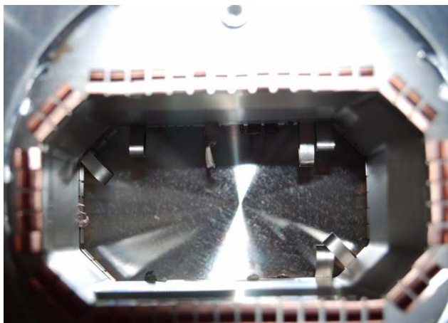
Figure 7: Damaged and melted fingers of 9062-bellows.
