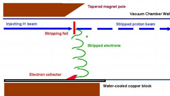
Figure 1: Injection area schematic layout.
