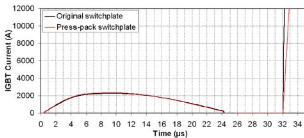
Figure 5: Simulated IGBT current during a shoot-through fault. The opposing IGBT is triggered at \sim 32 \mu\text{s} .
