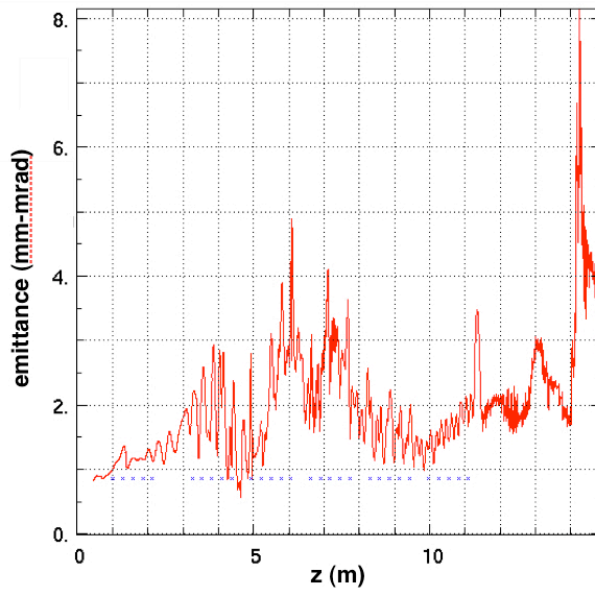
Figure 3. Evolution of the beam r-r' emittance during an axisymmetric WARP simulation of a 30\text{-nC L}^+ beam initialized in equilibrium. The beam was initialized with an x-x' emittance of 1\text{ mm-mrad} in the absence of bulk rotation. The blue “x”s again mark the centers of the thirty induction gaps.
