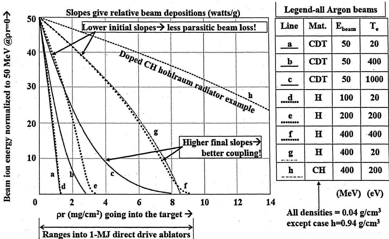
FIG. 3. Argon beam ion energy as a function of penetration \rho r into the ablated plasma/absorber, for the first three implosion times given in Table I, for various ablator materials at equal mass (except for h), incident ion energies, and electron temperatures.
