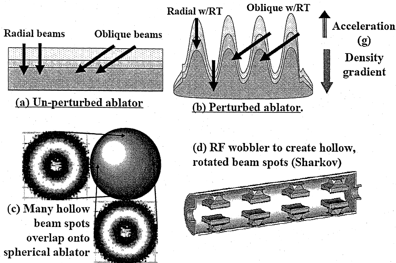
FIG. 5. Comparison of oblique as opposed to radial ion-beam deposition using rotated beam spots onto direct drive target ablators (proposed). (a) Unperturbed ablator; (b) perturbed ablator; (c) projection of hollow beam spots onto a spherical ablator, for smoothing and mitigation of RT instability; (d) schematic of a series of phased R . RF cavities that can produce and control hollow beams [after Sharkov (Ref. 21)].
