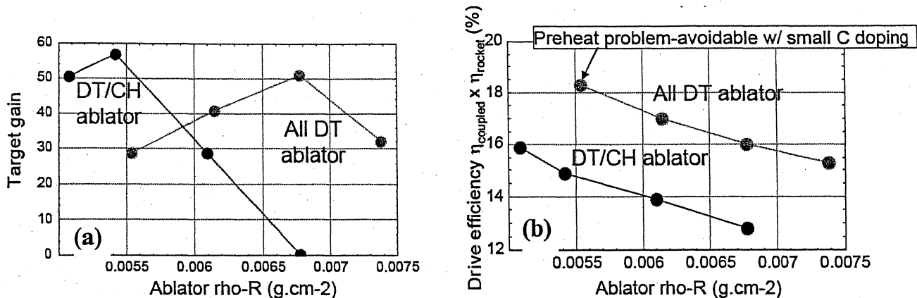
FIG. 4. LASNEX 1-D results for target gain (a) and drive coupling efficiency (b) as a function of ablator \rho r (g/cm 2 ) for the same fuel capsule and incident beam energy as in Fig. 2 (but retuning the pulse shape).
