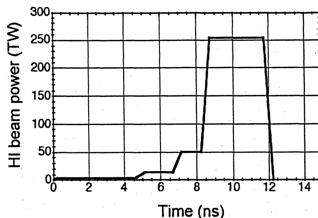
FIG. 2. A "pie" diagram of the target construction for the LASNEX calculation (a), and the 50 MeV argon ion-beam power pulse shape used (b). This case gives a fusion gain of 50 for 1 MJ of beam drive, assuming the incident beam profile zooms in a factor of 2 in radius (from 2 to 1 mm) during the drive.
