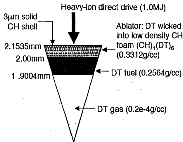
FIG. 2. A "pie" diagram of the target construction for the LASNEX calculation (a), and the 50 MeV argon ion-beam power pulse shape used (b). This case gives a fusion gain of 50 for 1 MJ of beam drive, assuming the incident beam profile zooms in a factor of 2 in radius (from 2 to 1 mm) during the drive.
