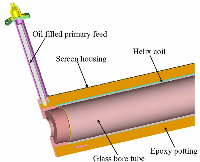
Figure 4: The PLIA assembly concept.
