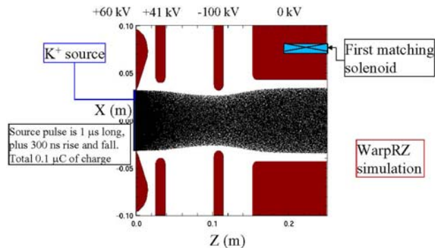
Figure 3: The Accel-Decel Injector.
