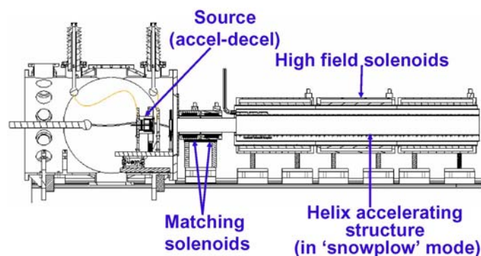
Figure 1: NDCX1c Experiment.
