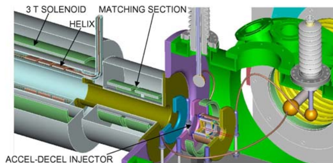
Figure 2: NDCX1c Experiment (cut-away view).
