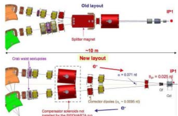
Figure 14: (top) Original layout of the DAΦNE ring, where the two beams collided head-on. (bottom) New layout for testing large crossing angle configuration, including crab waist sextupoles.
